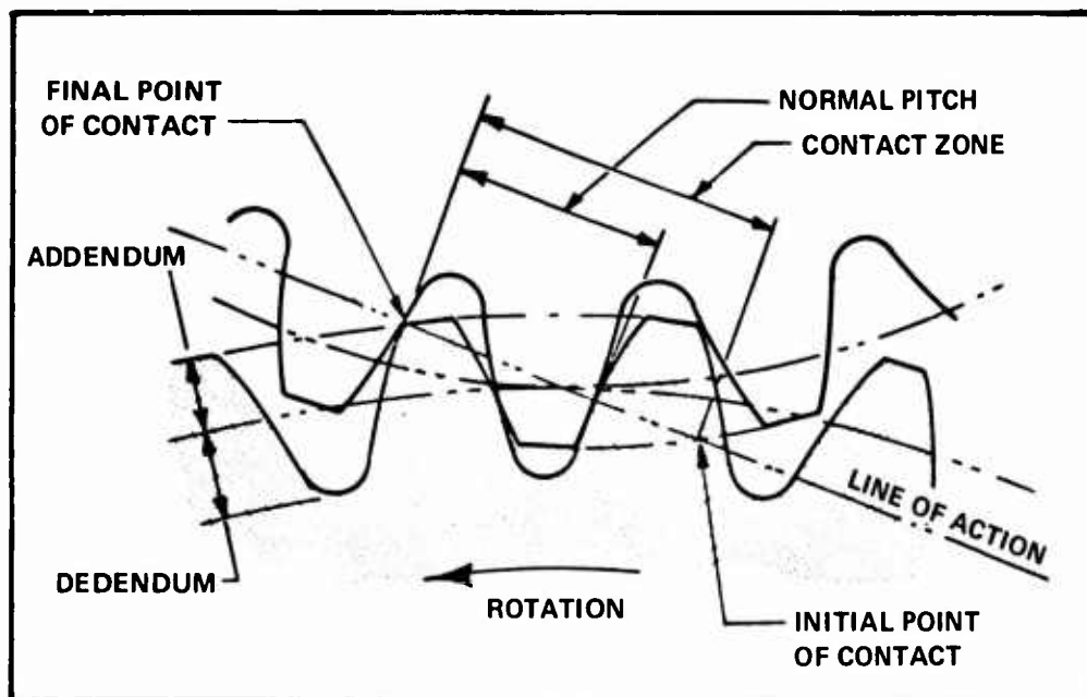
Figure 12. - High-contact-ratio gearing.
