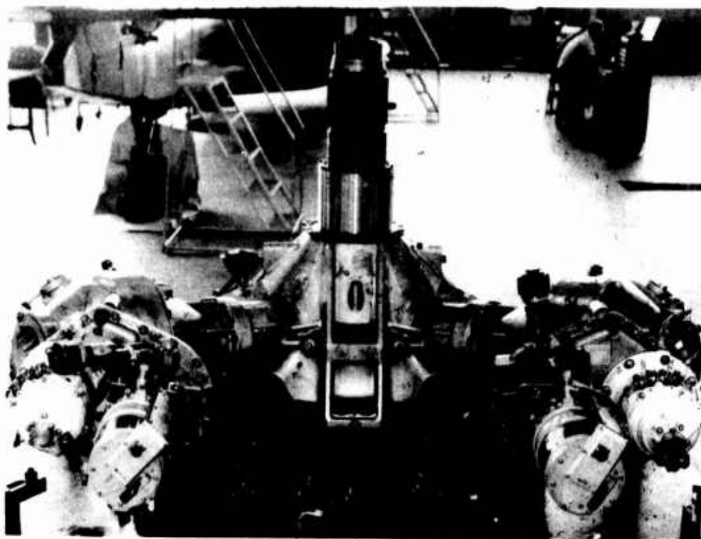
Figure 3. - Black Hawk main gearbox.
