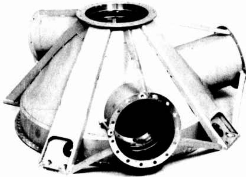
Figure 6. - Fabricated main transmission housing.
