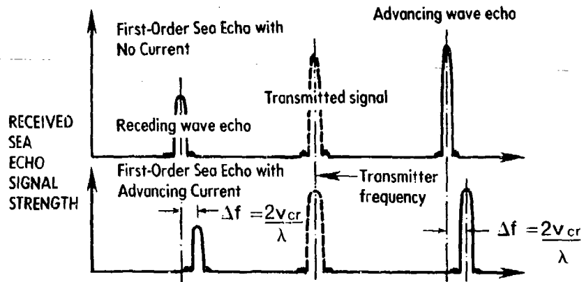
Figure 1 Sketch showing principles of first-order Bragg backscatter from the sea. Upper plot shows positions of echo energy in the signal spectrum from wave trains half the radar wavelength traveling toward and away from the radar. Lower plot shows symmetrical shift of these peaks by a current whose radial speed is v_{cr} .
