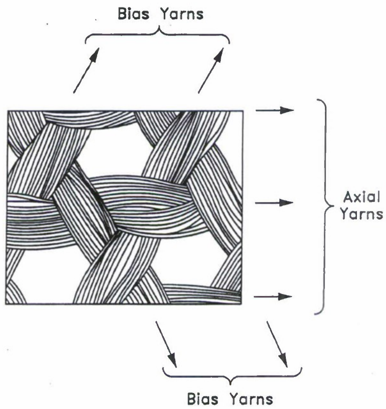
FIG. 18 (PRIOR ART)
