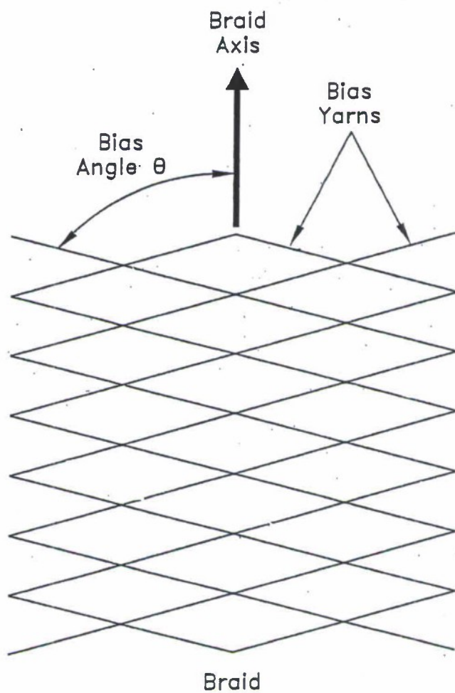
FIG. 12 (PRIOR ART)
