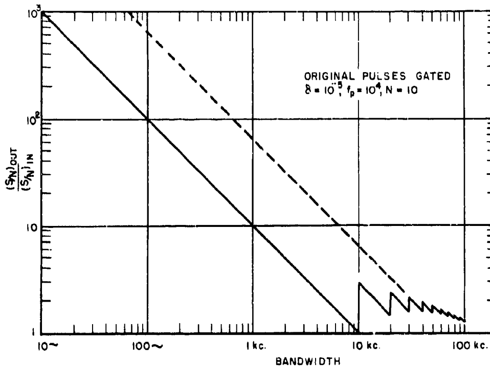
Figure 3 - Ratio (S/N)_{out}/(S/N)_{in} vs. bandwidth
