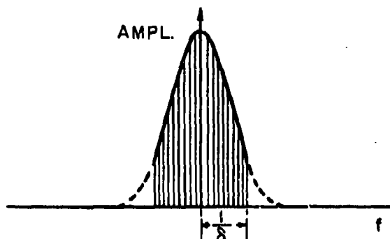
Figure 2 - New pulse spectrum - after envelope matching
