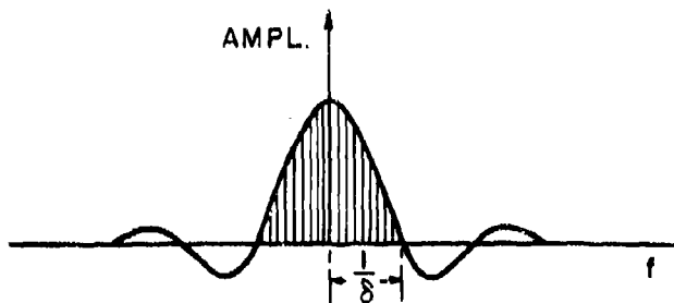
Figure 1 - Original pulses - before envelope matching
