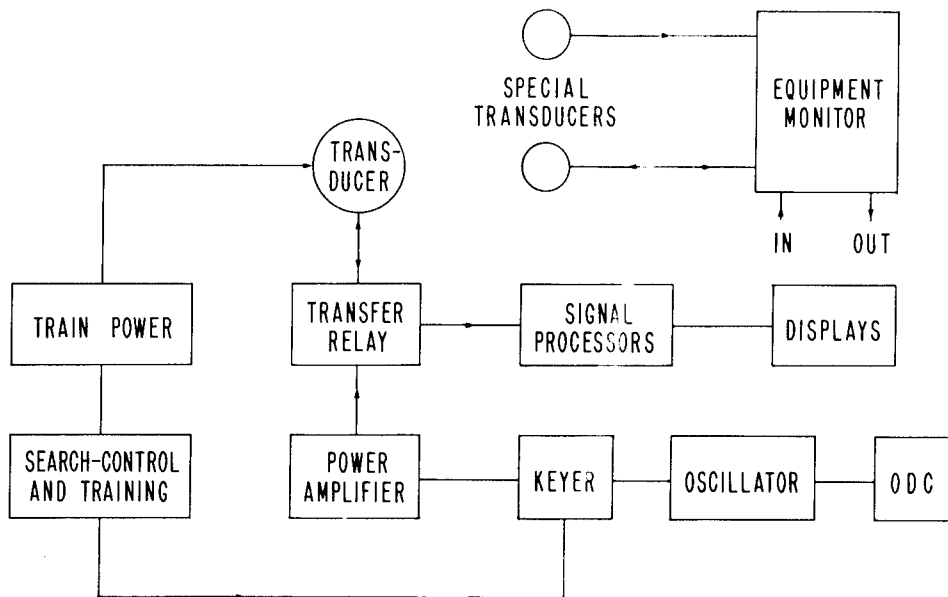
Figure 4 - Major components
