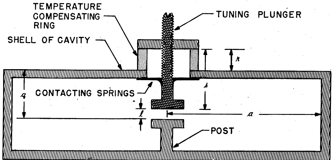
Figure 10 - Geometric configuration of cavity (cross-section view with critical dimensions noted)
