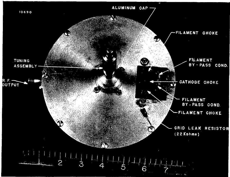
Figure 7a - External view, low-voltage cavity oscillator
