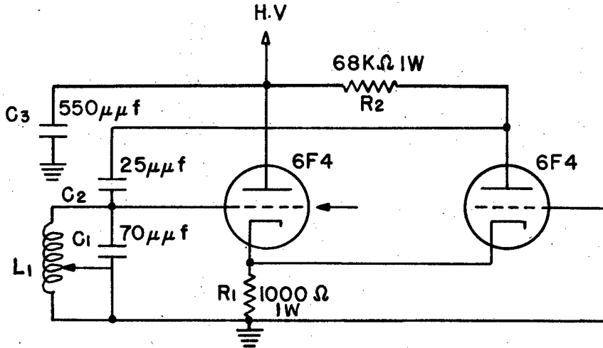
Figure 3 - Cathode-coupled oscillator
