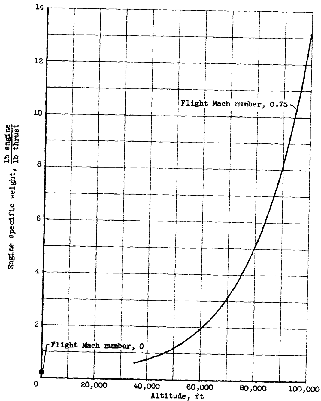
Figure 10. - Effect of altitude on engine specific weight.
