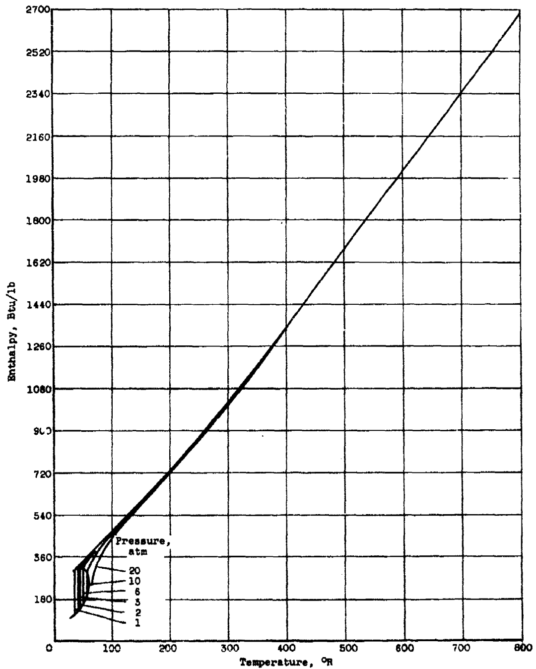
Figure 3. - Enthalpy of hydrogen.
