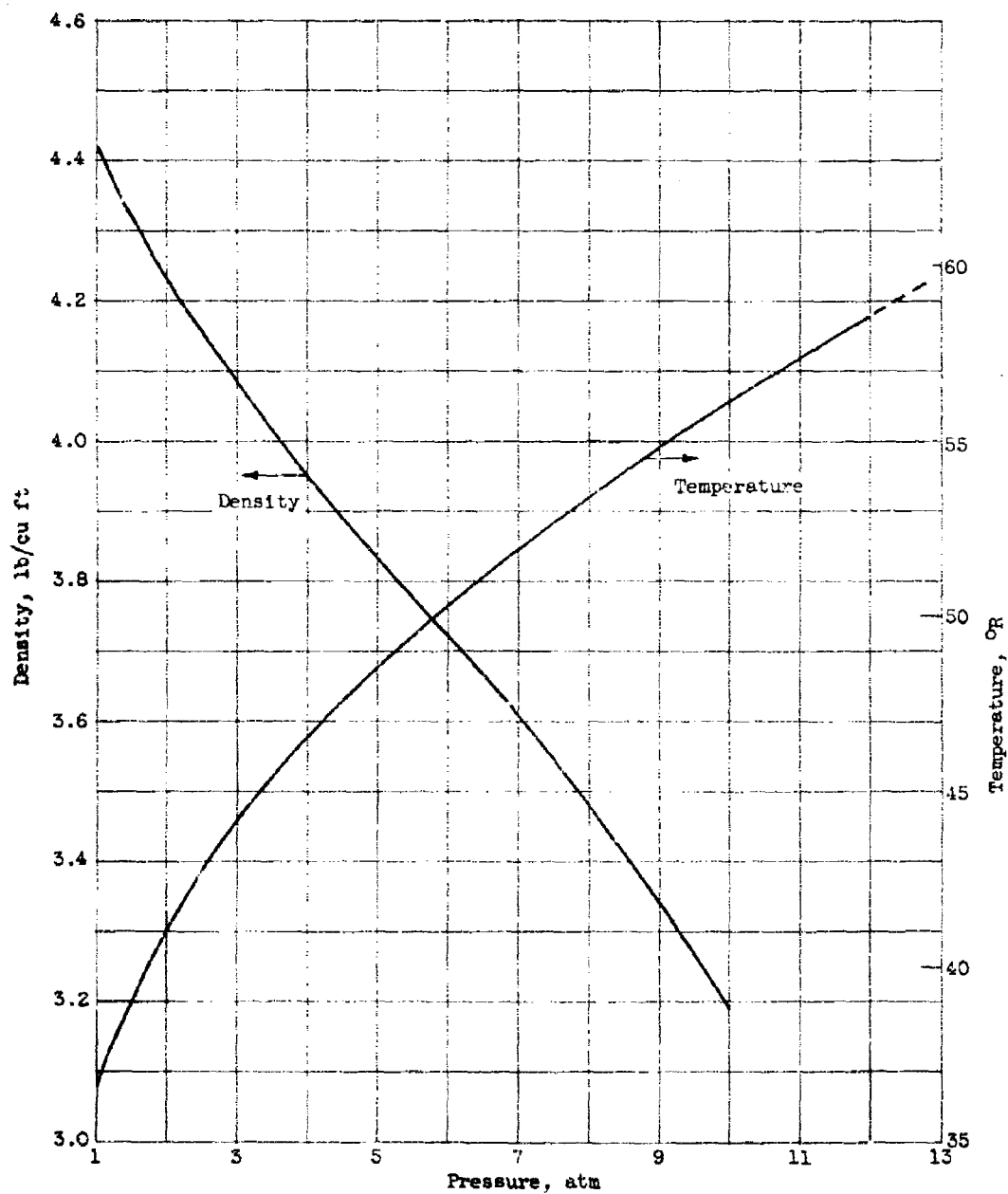
Figure 2. - Temperature-pressure-density relation of saturated liquid hydrogen.
