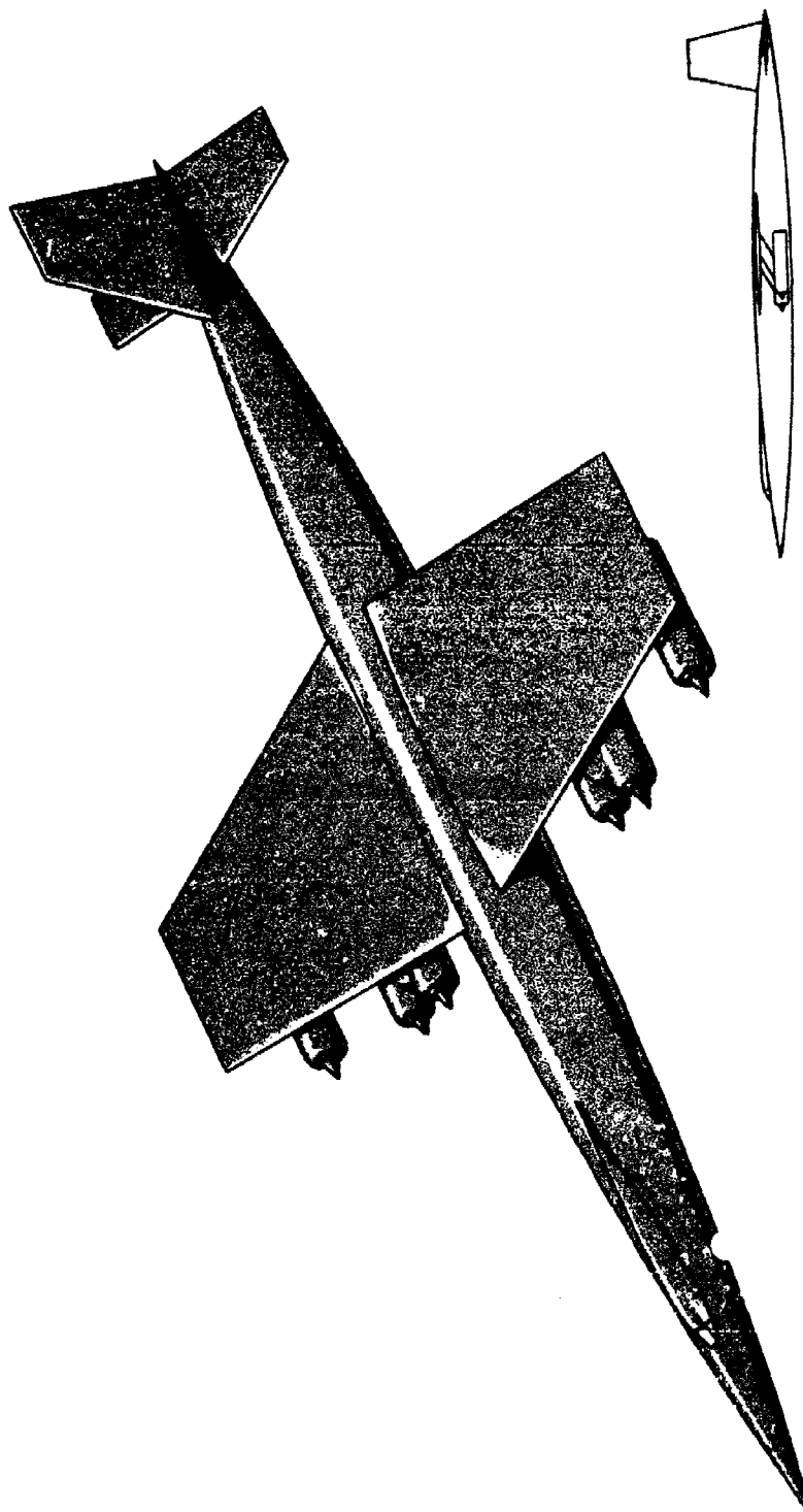
Figure 20. - Supersonic bomber. Flight Mach number, 2.0; target altitude, 75,000 feet.
