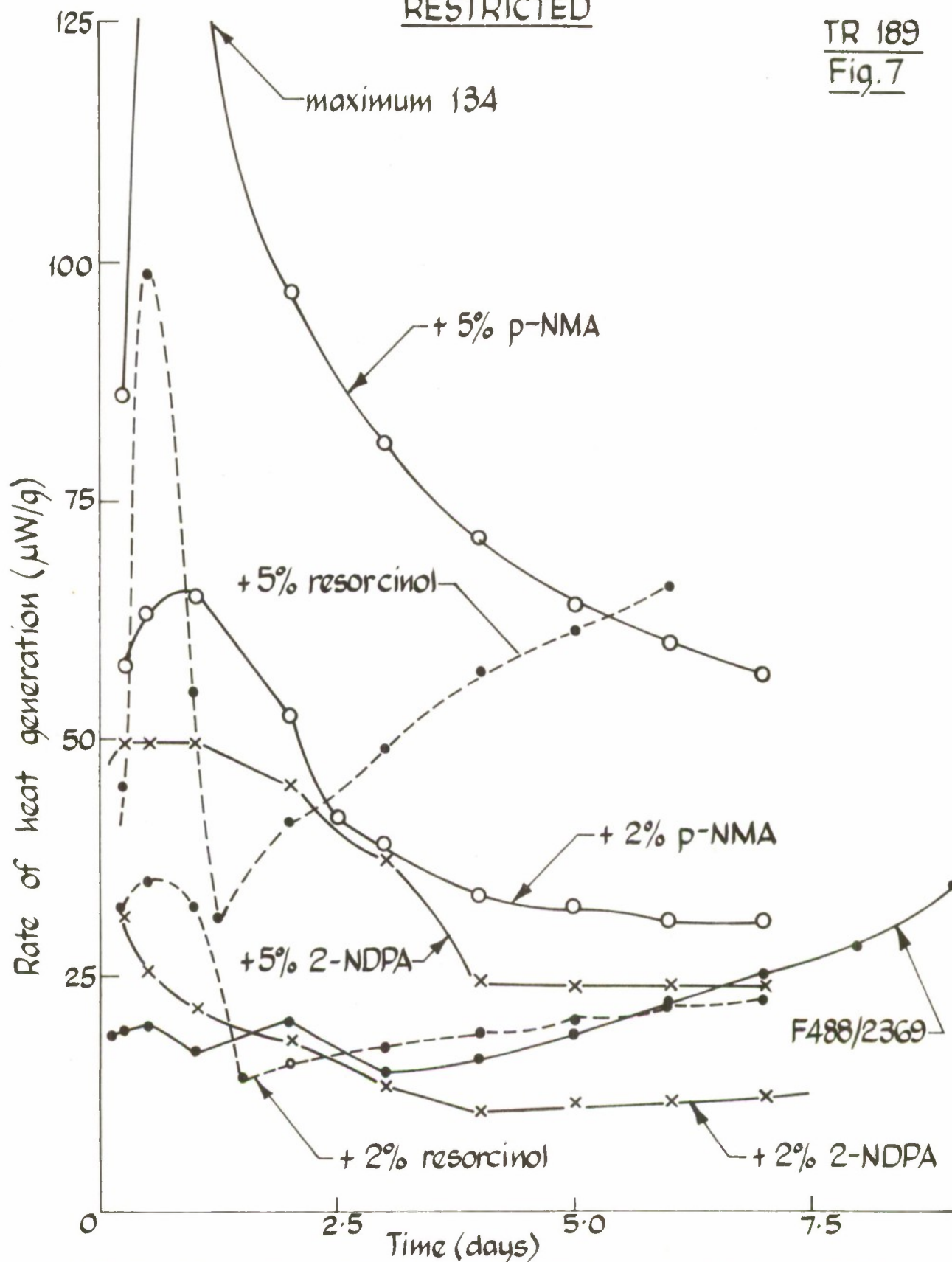
FIG.7 EFFECT OF ADDED STABILISERS ON THE HEAT GENERATION OF AN UNSTABILISED PROPELLANT AT 80^\circ\text{C}
