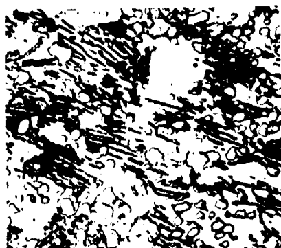
LOT I 1907 - CRITICAL SECTION. PEARLITE. SPHEROIDIZED CEMENTITE. SMALL FERRITE AREAS.
