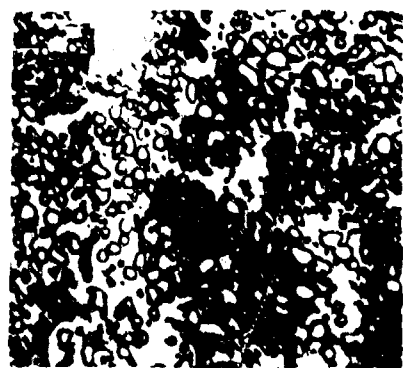
LOT I 1914 - CRITICAL SECTION SPHEROIDIZED CARBIDES. MARKED TRACES OF PEARLITE.
