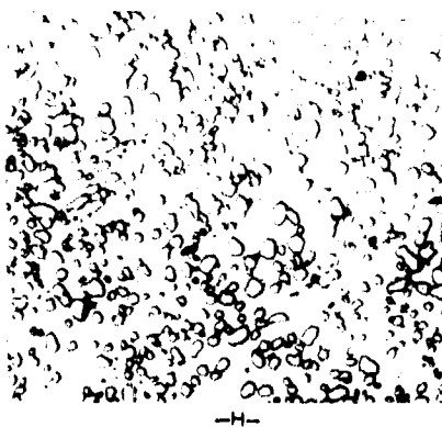
LOT H - CRITICAL SECTION SPHEROIDIZED CARBIDES. BAYONET NO. 1.
