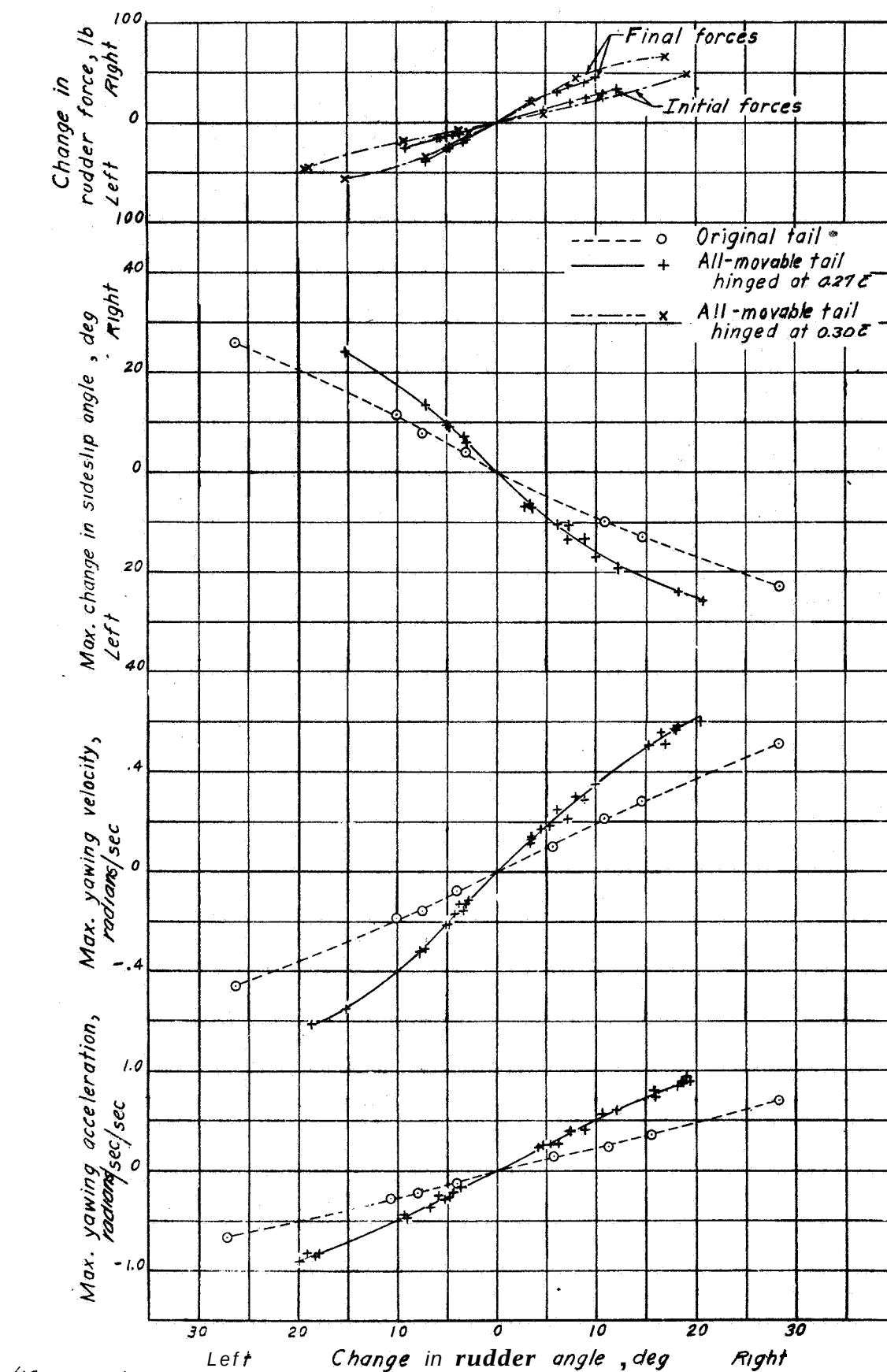
Figure 18.- Variation of maximum yawing acceleration, maximum yawing velocity, maximum change in sideslip angle, and change in rudder force with change in rudder angle. Abrupt rudder deflection with Fairchild XR2K-1 airplane at 60 miles per hour in the gliding condition.
