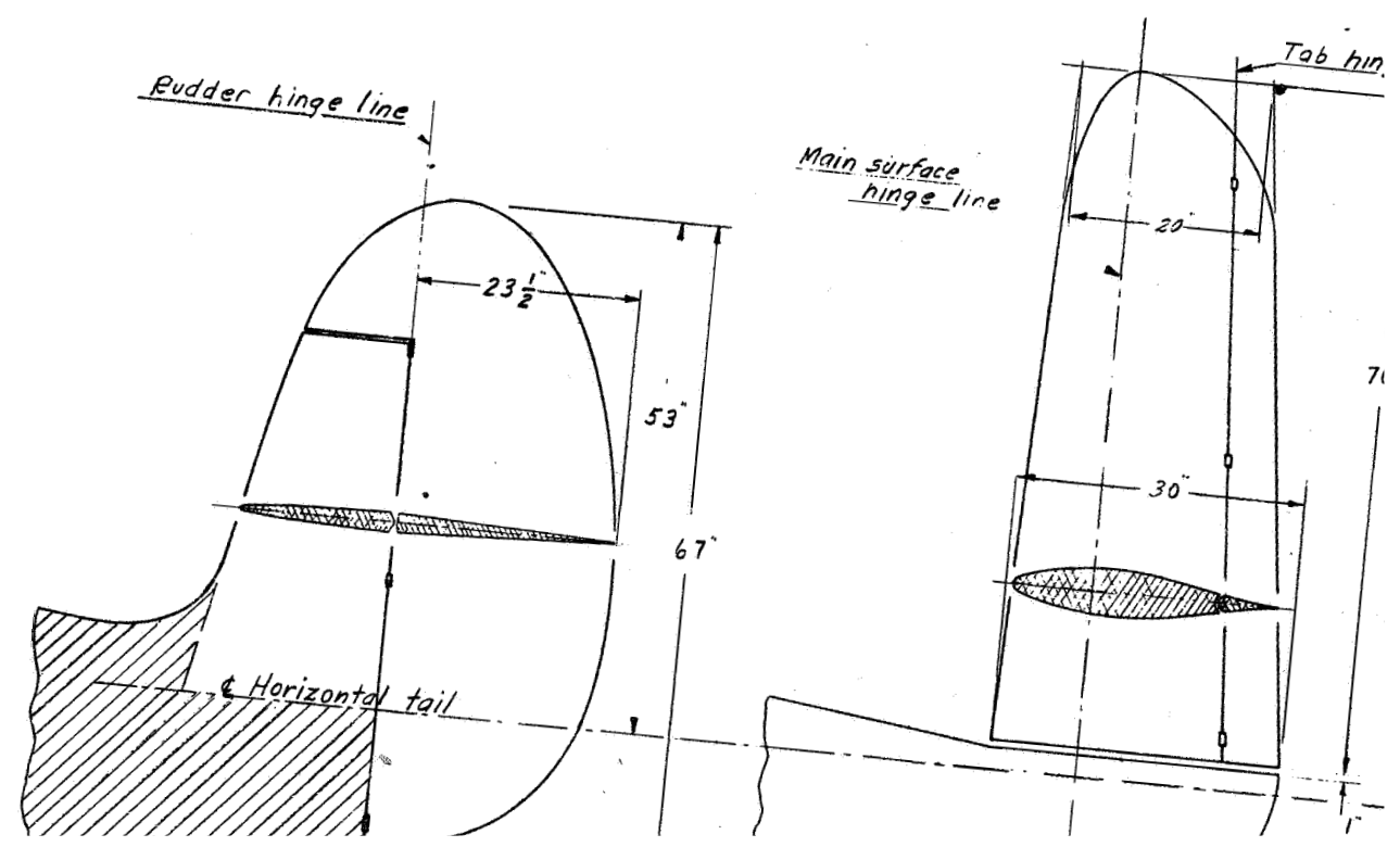
Figure 13. - Original vertical tail.
