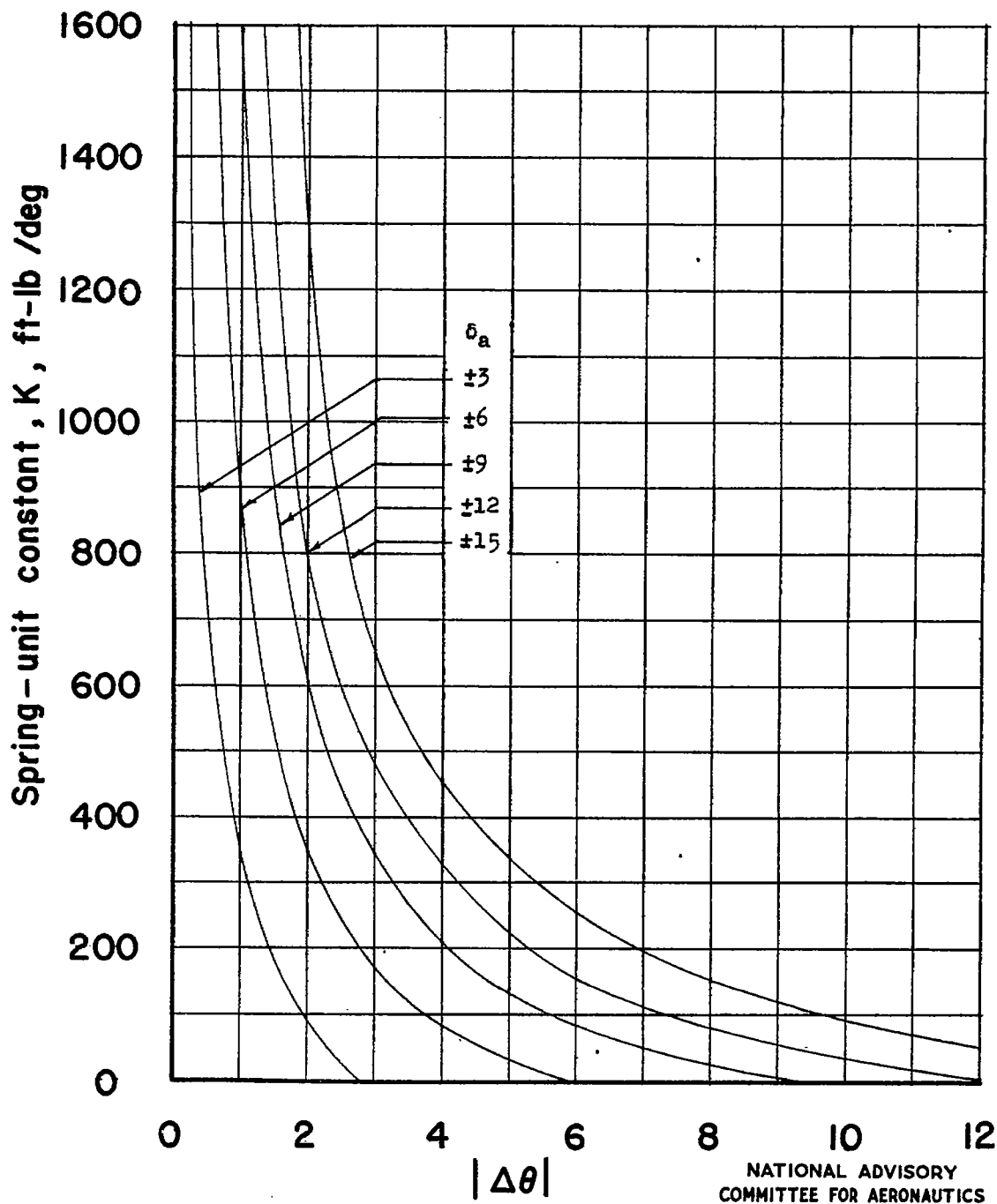
Figure 6.- The variation of the spring-unit constant required for equilibrium of the system with |\Delta\theta| for various aileron deflections at an initial angle of attack of 14^\circ of the model of the illustrative example.
