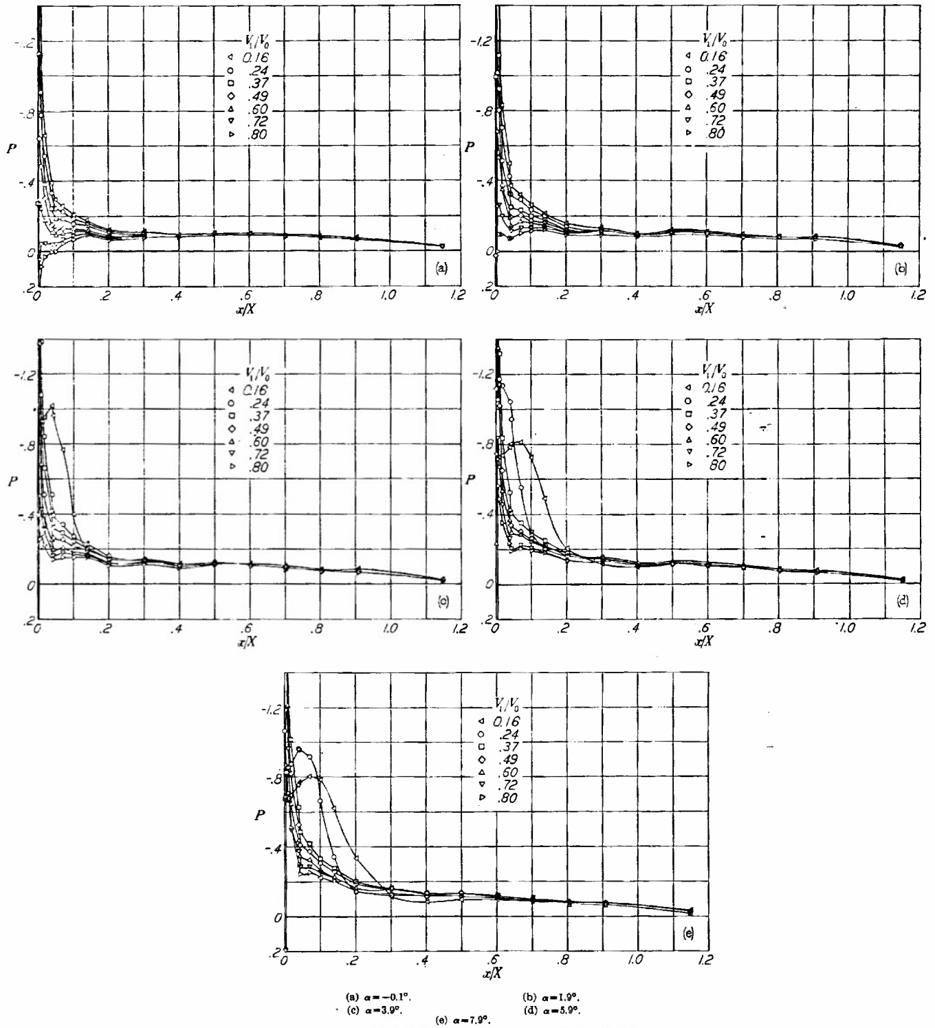
FIGURE 17.—Pressure distributions over the NACA 1-80-200 nose inlet. M_0 = 0.30 .
