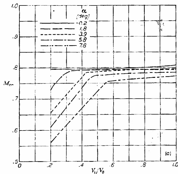
(a) NACA 1-50-200 nose inlet. (c) NACA 1-50-100 nose inlet. (b) NACA 1-50-150 nose inlet. (d) NACA 1-50-050 nose inlet. FIGURE 16.—Critical Mach numbers for the NACA 1-series nose inlets having an inlet-diameter ratio of 0.50.
