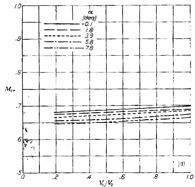
(a) NACA 1-50-200 nose inlet. (c) NACA 1-50-100 nose inlet. (b) NACA 1-50-150 nose inlet. (d) NACA 1-50-050 nose inlet. FIGURE 16.—Critical Mach numbers for the NACA 1-series nose inlets having an inlet-diameter ratio of 0.50.
