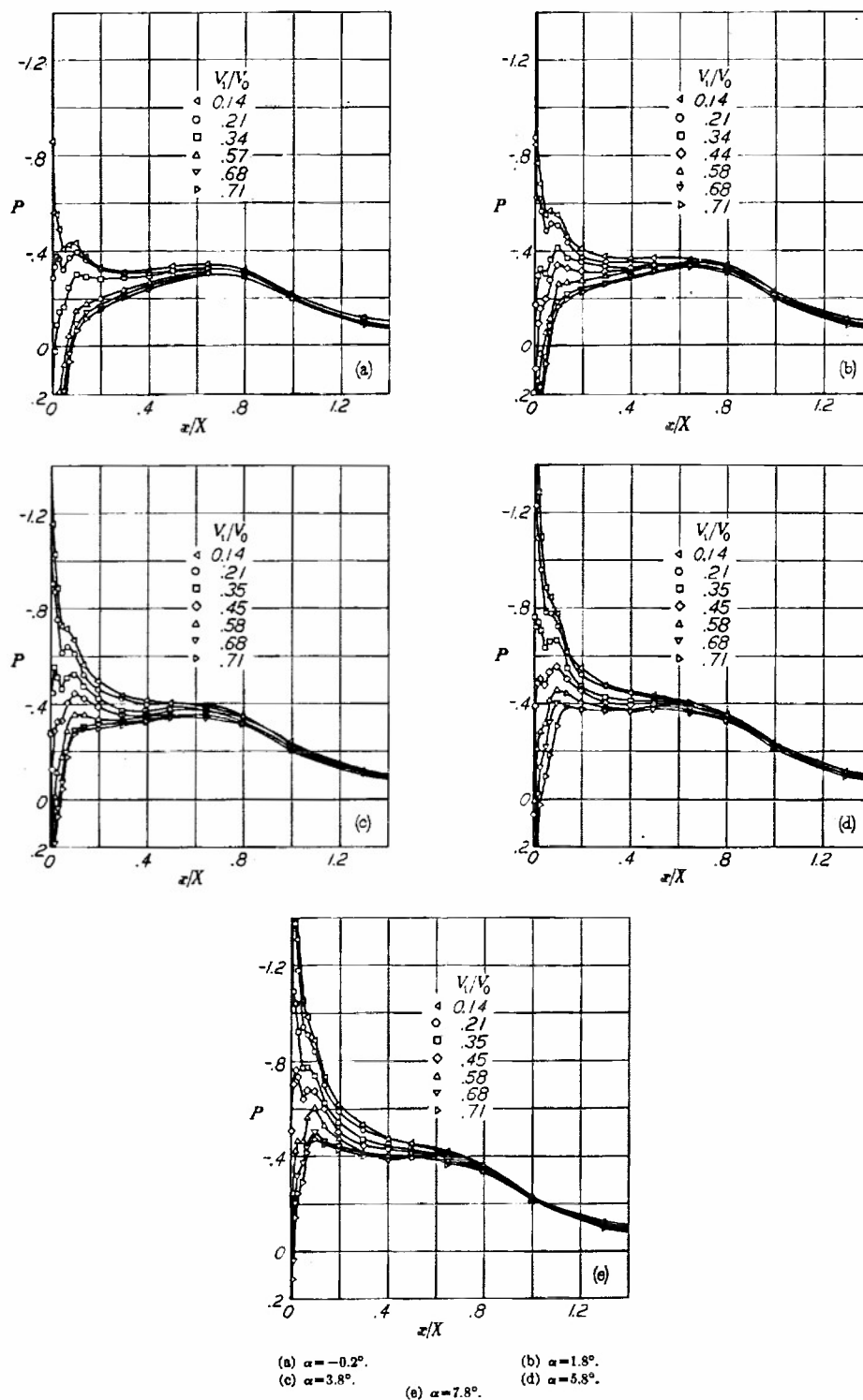
FIGURE 20.—Pressure distributions over the NACA 1-60-075 nose inlet. M_0 = 0.40 .
