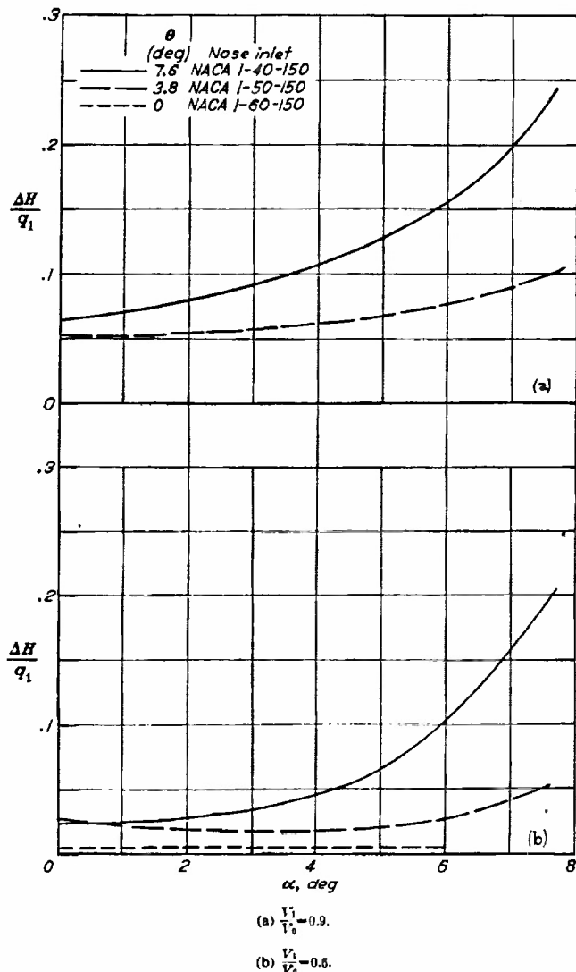
FIGURE 51.—Variation of internal total-pressure loss with angle of attack. \frac{x}{D} = 1.5 ; M_0 = 0.40
