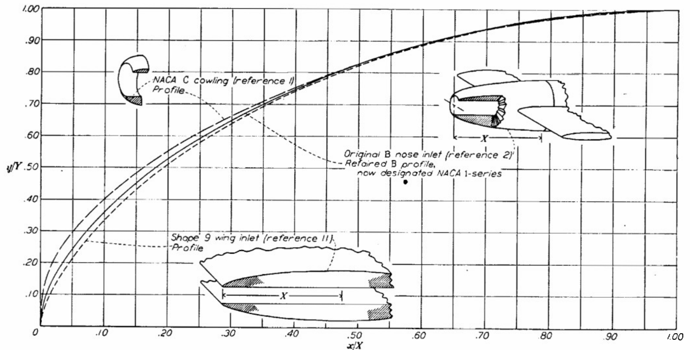
FIGURE 3.—Comparison of nondimensional profiles and proportions of three high-critical-speed air inlets from references 1, 2, and 11.
