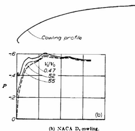
FIGURE 38.—Pressure distributions over NACA D 1 and D 2 cowlings. (Data from references 5 and 6.) \alpha = 0^\circ .
