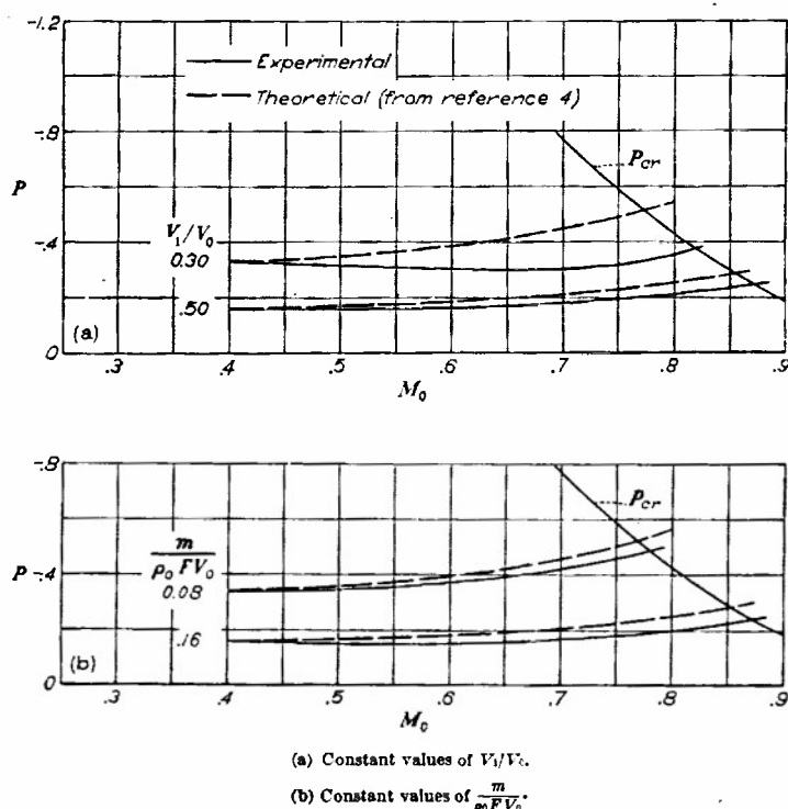
FIGURE 42.—Variation of peak negative pressure coefficient with Mach number for the NACA 1-50-150 nose inlet. \alpha = 0.2^\circ .
