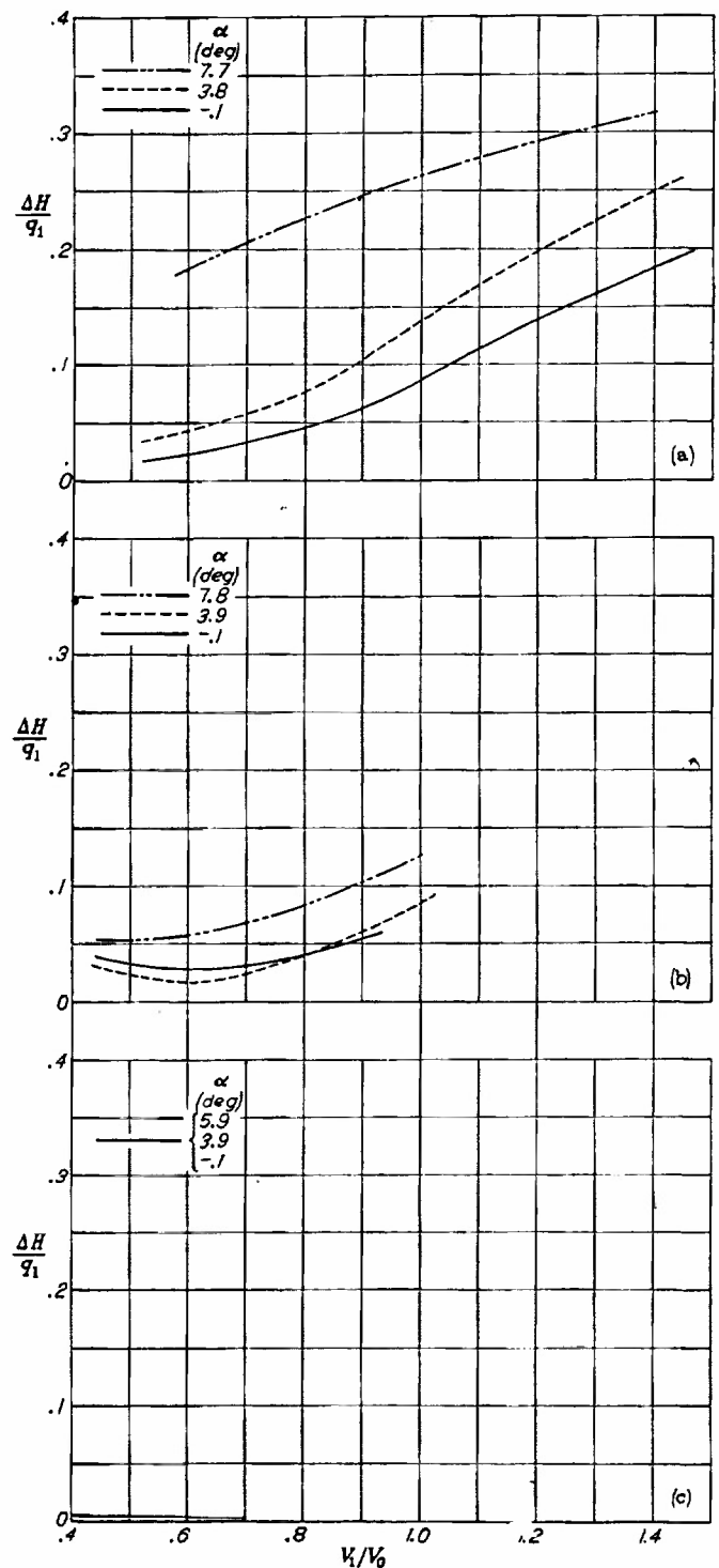
(a) NACA 1-40-150 nose inlet ( \theta = 7.6^\circ ). (b) NACA 1-50-150 nose inlet ( \theta = 3.8^\circ ). (c) NACA 1-60-150 nose inlet ( \theta = 0^\circ ). FIGURE 49.—Variation of internal total-pressure loss with inlet-velocity ratio for nose inlets of X/D = 1.5 . M_0 = 0.40 .
