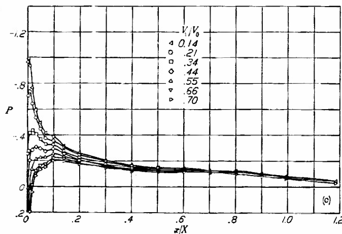
FIGURE 58.—Pressure distributions over the modified nose inlets tested. NACA 1-60-150 nose inlet included for comparison; \alpha=0^\circ .
