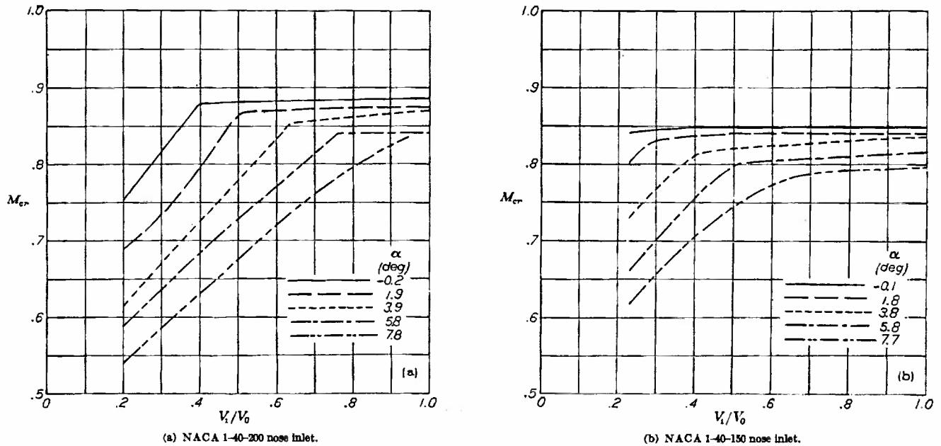
FIGURE 11.—Critical Mach numbers for the NACA 1-series nose inlets having an inlet-diameter ratio of 0.40.
