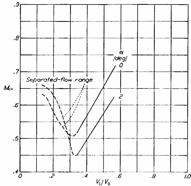
FIGURE 46.—Critical Mach numbers for the NACA 1-70-150 nose inlet. Separated-flow range included.
