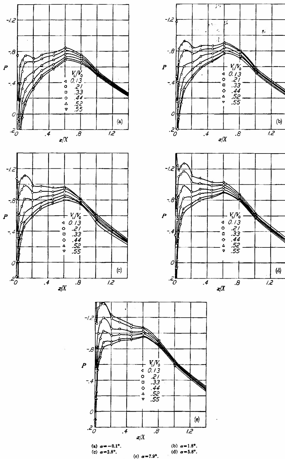
FIGURE 34.—Pressure distributions over the NACA C cowling. M_1=0.40 .
