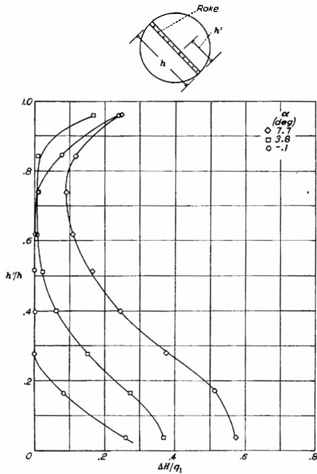
FIGURE 48.—Typical profile of internal total-pressure loss at rake station. NACA 1-40-150 nose inlet: V_1/V_c = 0.93 ; M_0 = 0.40 ; \theta = 7.6^\circ .
