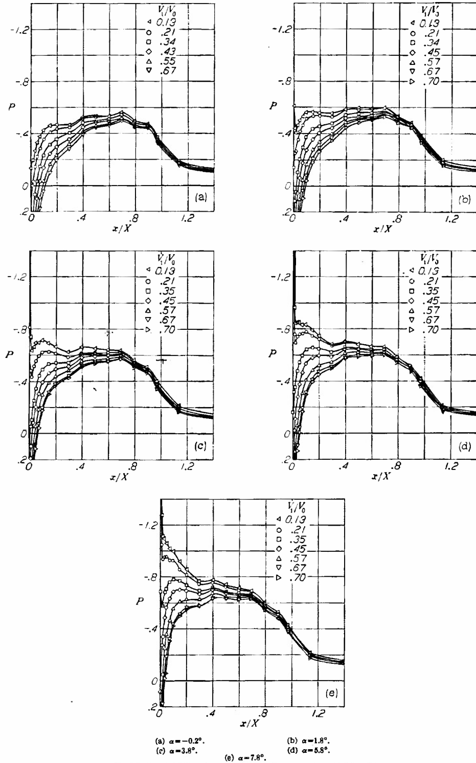
FIGURE 21.—Pressure distributions over the NACA 1-60-050 nose inlet. M_2 = 0.40 .
