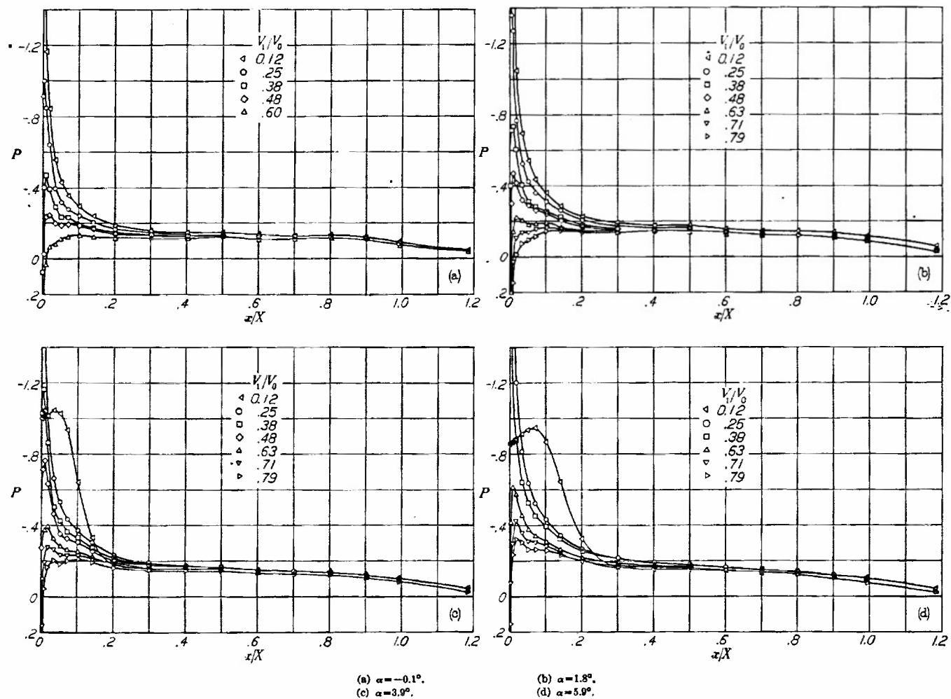
FIGURE 18.—Pressure distributions over the NACA 1-80-150 nose inlet. M_0 = 0.30 .
