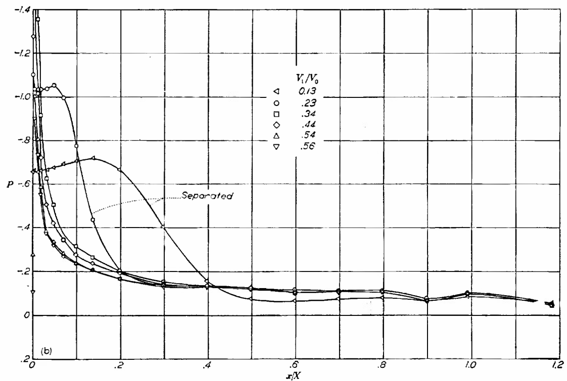
(a) \alpha = -0.1^\circ . (b) \alpha = 1.8^\circ . FIGURE 23.—Pressure distributions over the NACA 1-70-150 nose inlet. M_0 = 0.40 .
