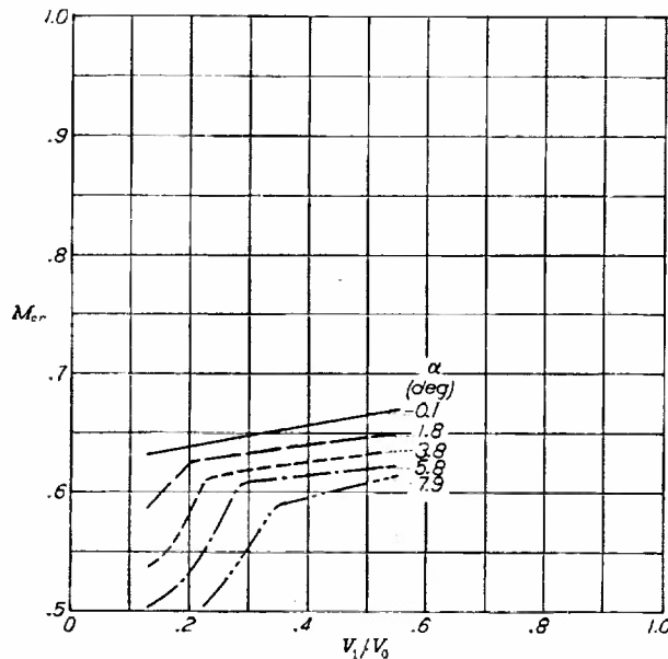
FIGURE 35.—Critical Mach numbers for the NACA C cowl.
