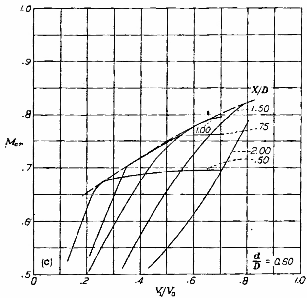
(c) \alpha = 4^\circ (nominal). FIGURE 28.—Concluded.
