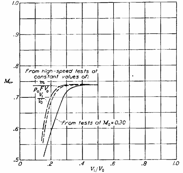
FIGURE 45.—Critical Mach numbers obtained from tests at M_0 = 0.30 (fig. 27 (e)) and from tests at high speed (fig. 43) for the NACA 1-70-050 nose inlet. \alpha = 0.1^\circ .
