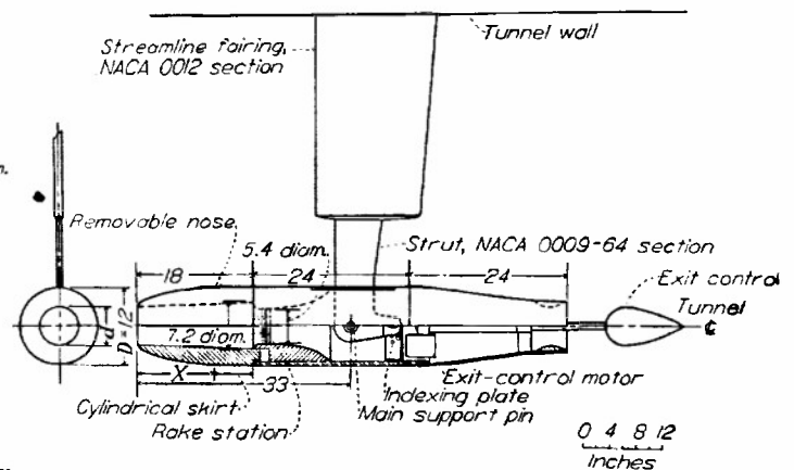
FIGURE 8.—Model installation and details
