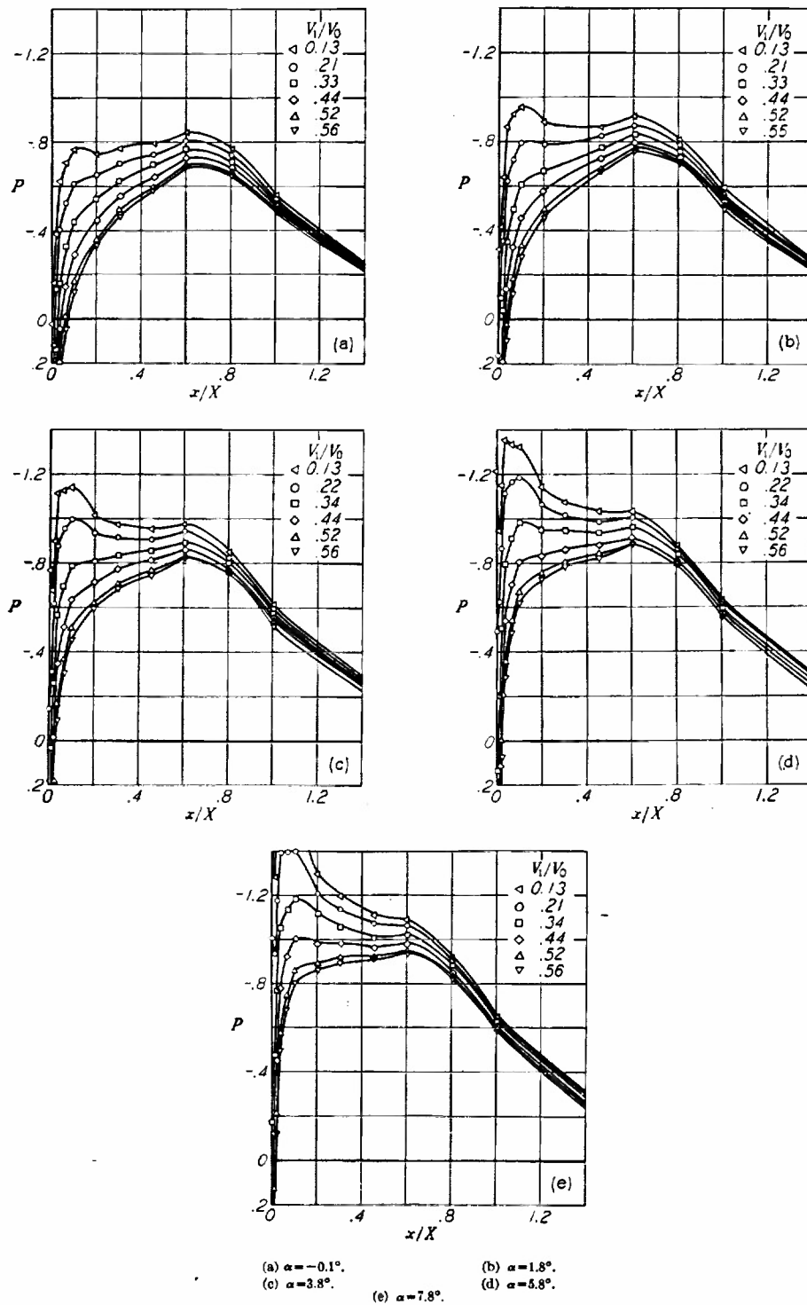
FIGURE 55.—Pressure distributions over the NACA C cowl with increased lip radius. M_0=0.40 .
