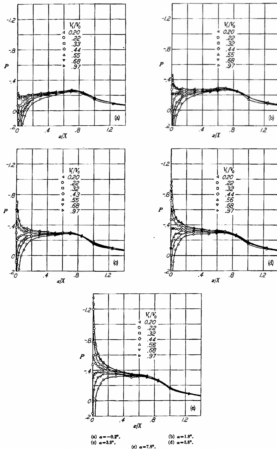
FIGURE 14.—Pressure distributions over the NACA 1-50-100 nose inlet. M_1 = 0.40 .
