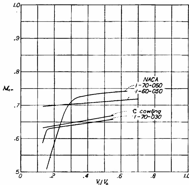
FIGURE 36.—Comparison of critical Mach number characteristics of NACA C cowl and 1-series nose inlets. \alpha=0^\circ .
