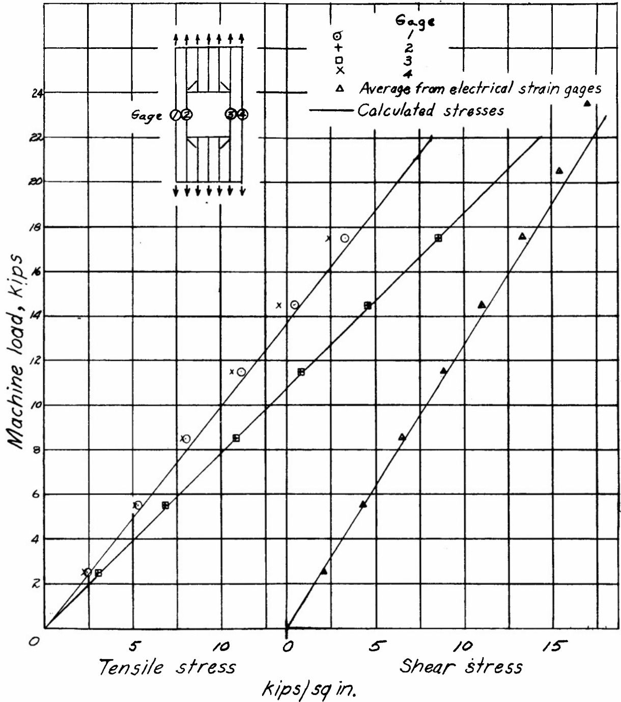
Figure 15.- Stresses in small panel number 9. Panel load is equal to \frac{7}{8} machine load.
