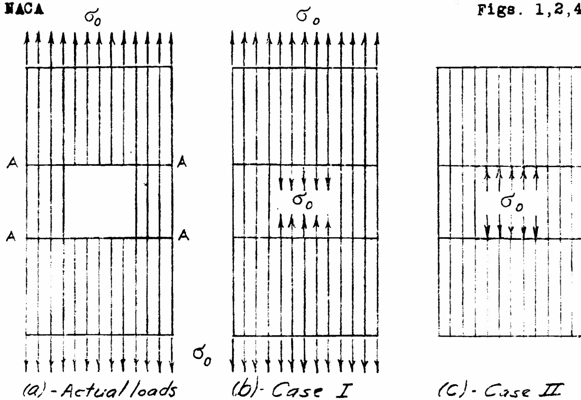
Figure 1. - Panel with cut-out.
