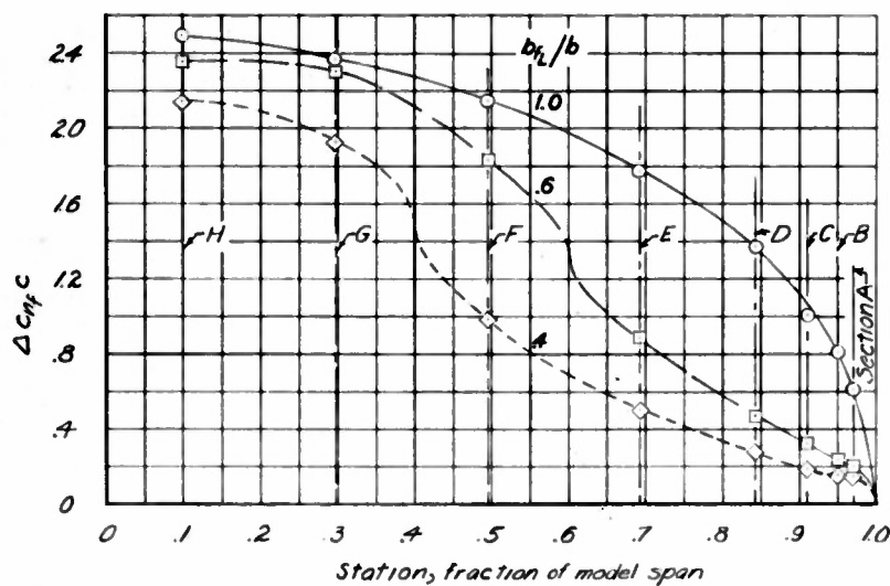
Figure 18. - Variation of the incremental spanwise loading caused by a 0.40c-chord lift flap of various spans. \delta_L = 60^\circ .
