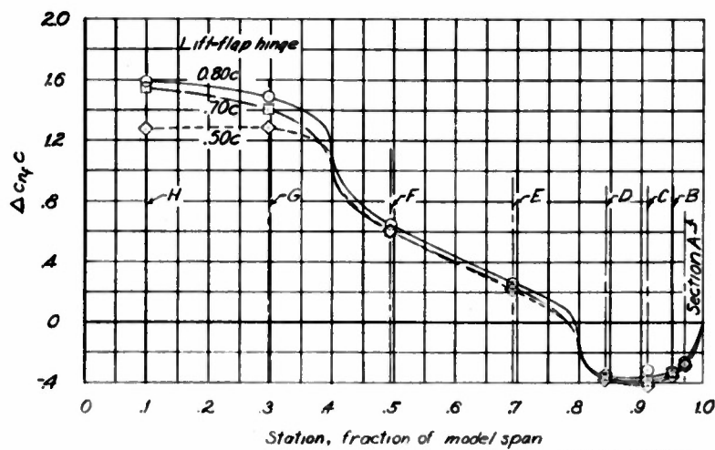
Figure 19. - Variation of the incremental spanwise loading caused by varying the hinge location of a 0.20-c-chord lift flap with a 0.20-c-chord trim flap hinged in the normal position. b_L = 0.40 b ; b_T = 0.20 b ; \delta_L = 60^\circ ; \delta_T = 60^\circ .
