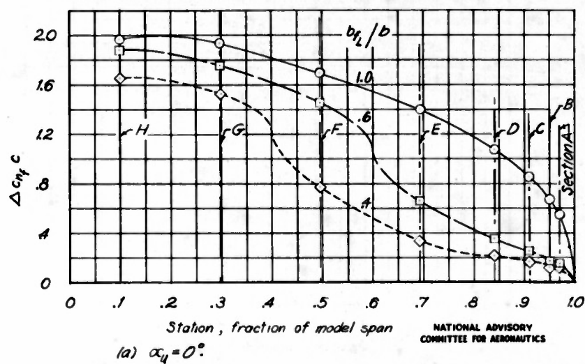
Figure 17. - Variation of the incremental spanwise loading caused by a 0.20c-chord lift flap of various spans. \delta_f = 60^\circ .
