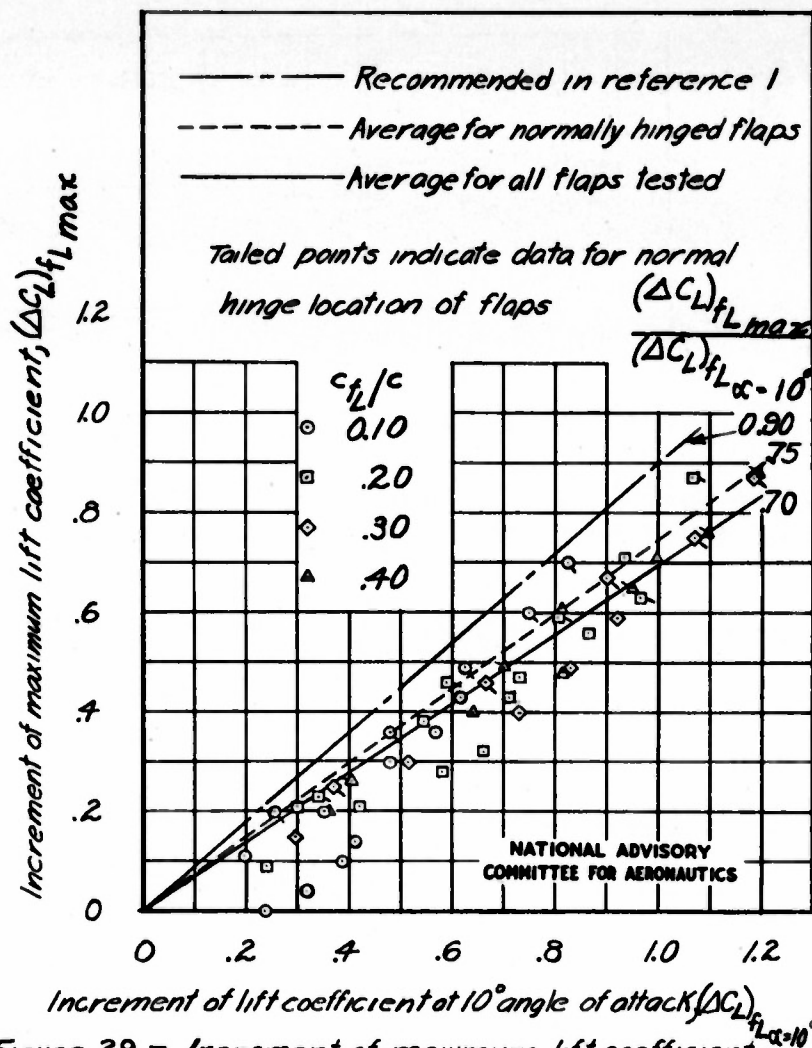
Figure 29. - Increment of maximum lift coefficient against increment of lift coefficient at 10° angle of attack for all flaps tested.
