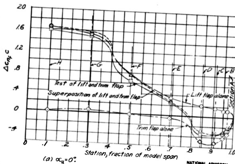
Figure 21. - Comparison of the incremental spanwise loading obtained from tests of a lift flap and a trim flap with that obtained by a superposition of the loadings obtained with each flap tested separately. Hinge location normal; C_L = 0.20c ; c_{H_L} = 0.20c ; b_L = 0.40b ; b_{H_L} = 0.20b ; \delta_L = 60^\circ ; \delta_{H_L} = 60^\circ .
