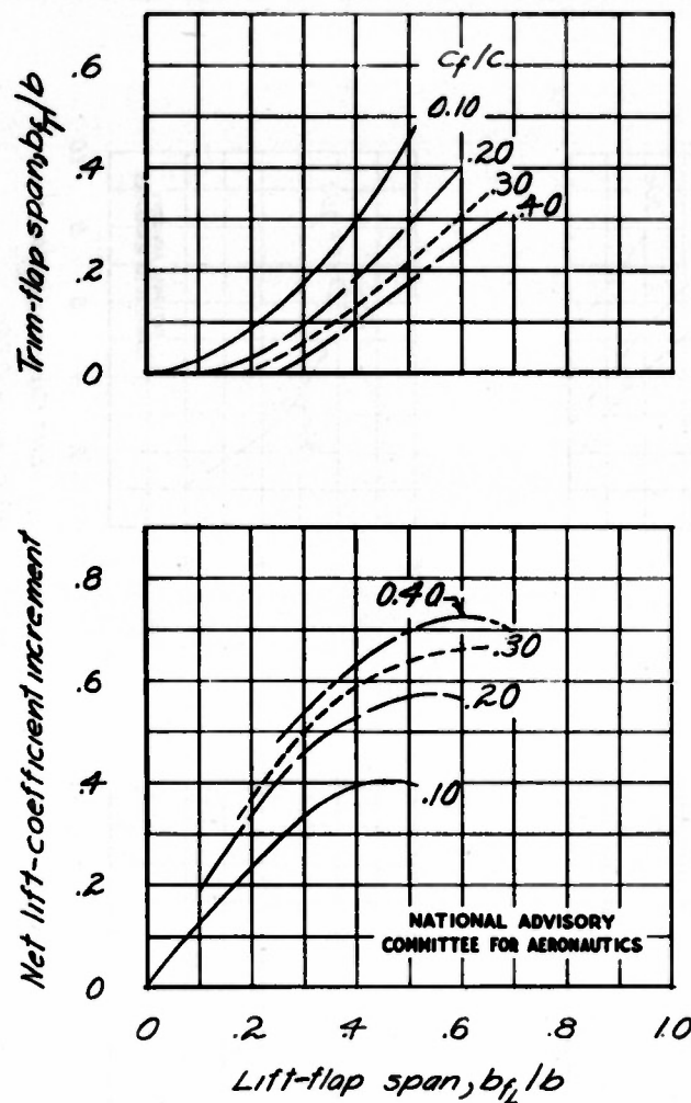
Figure 24. - Effect of lift-flap span on the net lift-coefficient increment and trim-flap span for various-chord lift and trim flaps. \alpha = 10^\circ ; \Delta C_m = 0 ; \delta_{t_f} = 60^\circ ; \delta_{l_f} = 60^\circ .
