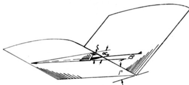
(b) Vee tail in sideslip; \alpha = 0^\circ . If \beta is small, \alpha_N = \beta \sin \Gamma .
