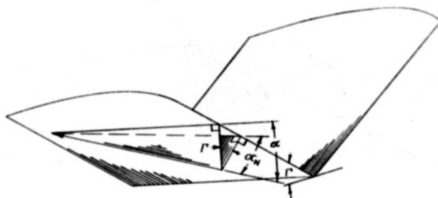
(a) Vee tail in pitch; \beta = 0^\circ . If \alpha is small, \alpha_N = \alpha \cos \Gamma .
