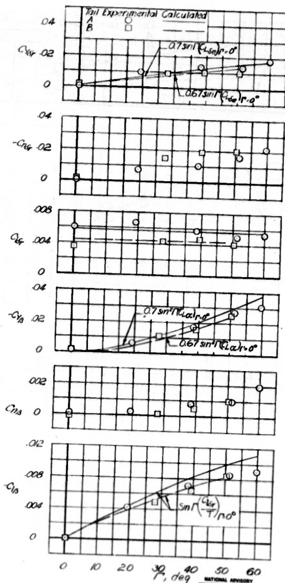
Figure 11. - Variations of rolling-moment, yawing-moment, and lateral-force parameters with dihedral angle. \alpha = \delta = 0^\circ .
