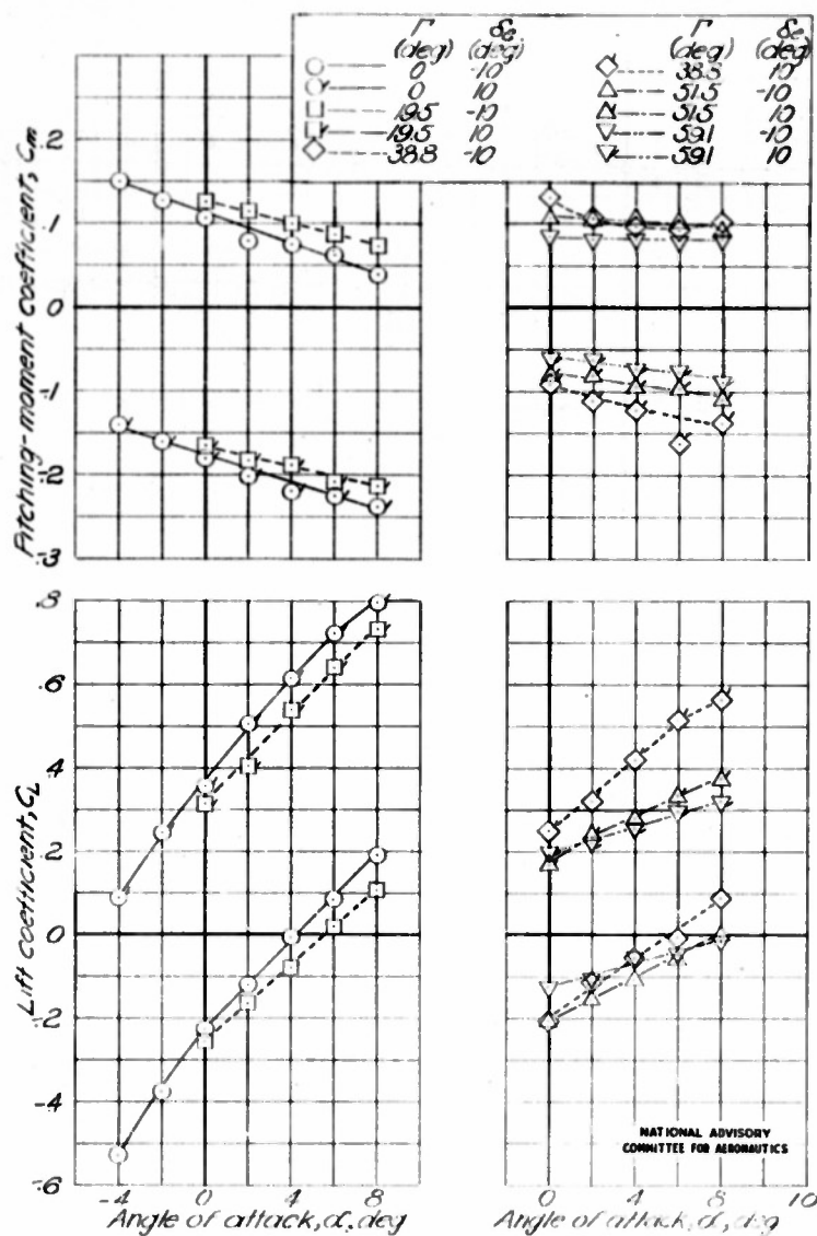
Figure 5—Elevator effectiveness of tail A with various dihedral angles, \delta_r , 0°.
