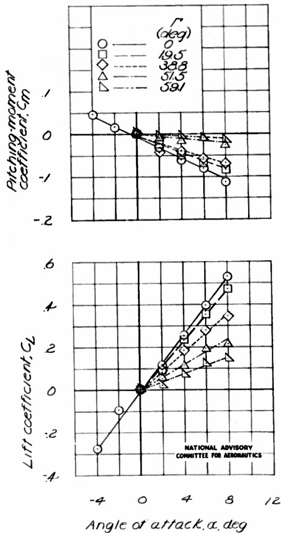
Figure 4.-Lift and pitching-moment characteristics of tail A with various dihedral angles. \delta_e = \delta_r = \psi = 0^\circ .
