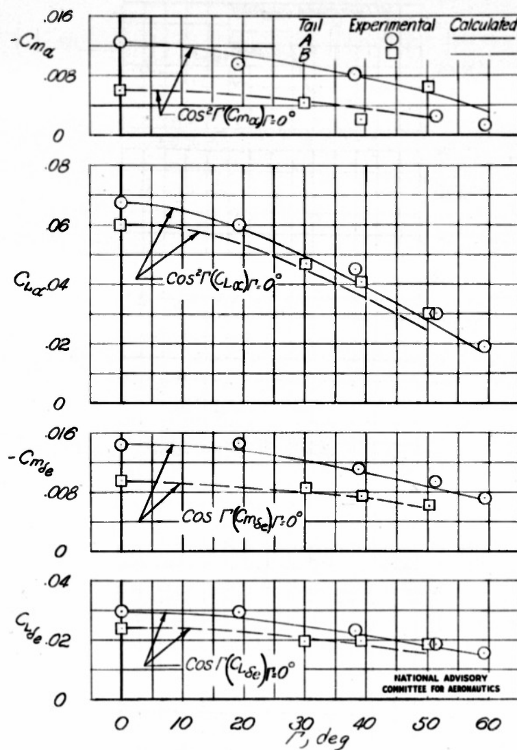
Figure 10.- Variation of lift and pitching-moment parameters with dihedral angle. \alpha = \delta = \Gamma = 0^\circ
