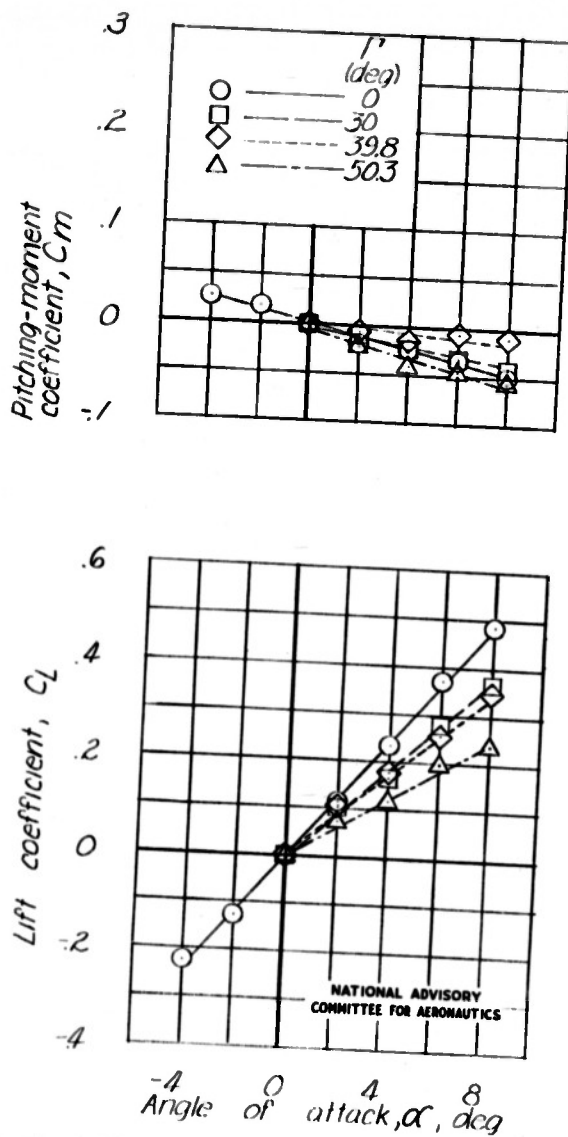
Figure 7.- Lift and pitching-moment characteristics of tail B with various dihedral angles. \delta_C = \delta_T = \psi = 0^\circ .
