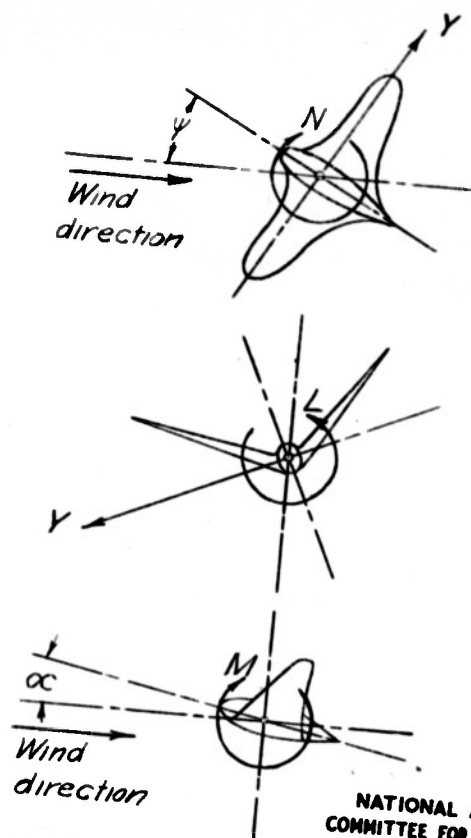
Figure 2.-The stability system of axes. This system of axes is defined as an orthogonal system in which the Z-axis is in the plane of symmetry and perpendicular to the relative wind, the X-axis is in the plane of symmetry and perpendicular to the Z-axis, and the Y-axis is perpendicular to the plane of symmetry. Arrows indicate positive directions of moments and forces.
