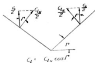
(c) Vee tail in pitch.
