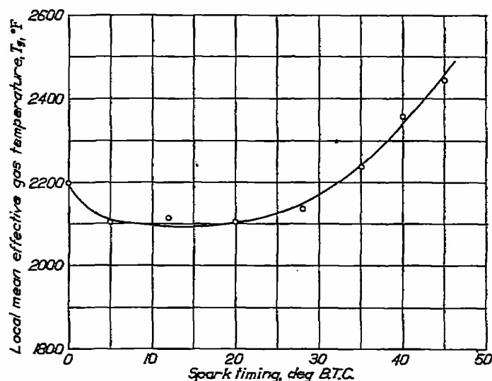
FIGURE 9.—Effect of spark timing on local mean effective gas temperature. Engine speed, 2200 rpm; indicated horsepower, 97; fuel-air ratio, 0.06; cooling-air pressure drop, 16 inches of water; combustion-air temperature, 150° F. (Data from reference 2, fig. 9.)
