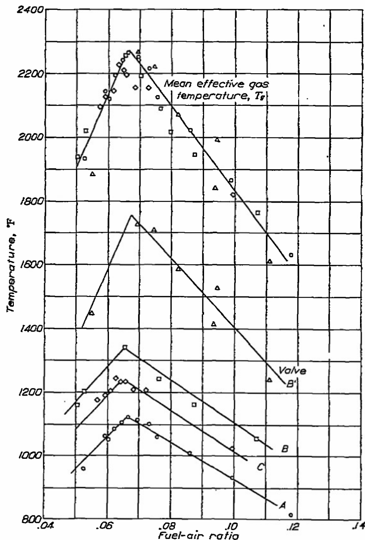
FIGURE 8.—Variation of mean effective gas temperature and valve temperature with fuel-air ratio. Engine speed, 2200 rpm; indicated horsepower, 117; combustion-air temperature, 110° F; cooling-air pressure drop, 16 inches of water; spark timing, 22¼° B. T. C.
