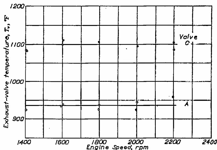
FIGURE 12.—Variation of exhaust-valve temperature with engine speed. Indicated horsepower, 71.5; fuel-air ratio, 0.072; combustion-air temperature, 150^{\circ}\text{F} ; cooling-air pressure drop, 16 inches of water.
