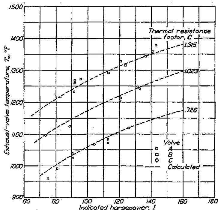
FIGURE 11.—Comparison of calculated and experimentally determined exhaust-valve temperatures in air-cooled cylinder. Engine speed, 2200 rpm; fuel-air ratio, 0.072; combustion-air temperature, 150^{\circ}\text{F} ; cooling-air pressure drop, 16 inches of water.
