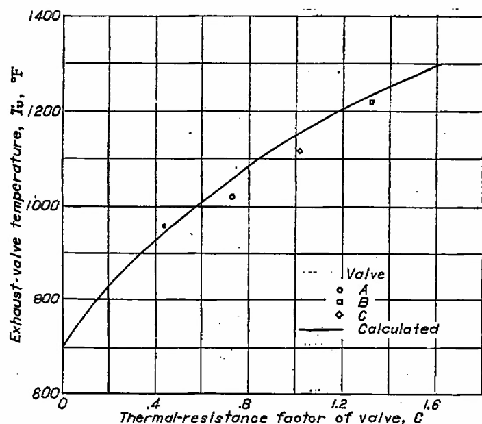
FIGURE 10.—Effect of thermal-resistance factor on exhaust-valve temperature. Engine speed, 2300 rpm; indicated horsepower, 129; fuel-air ratio, 0.09; combustion-air temperature, 156^{\circ}\text{F} ; rear-spark-plug-bushing temperature, 425^{\circ}\text{F} .
