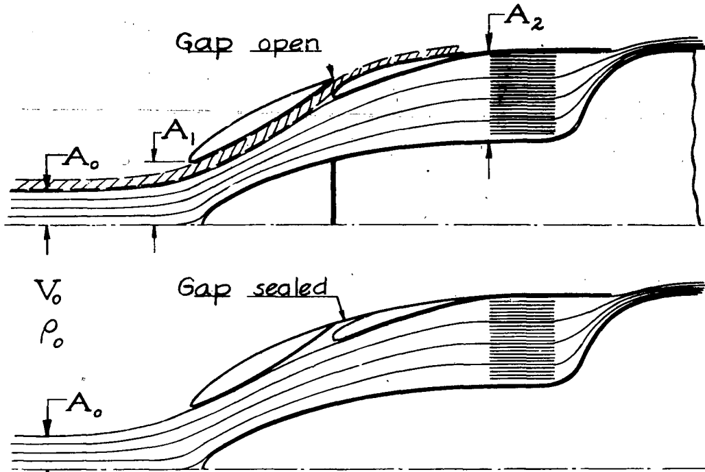
Figure 2. - Comparison of flows with open and sealed gaps.
