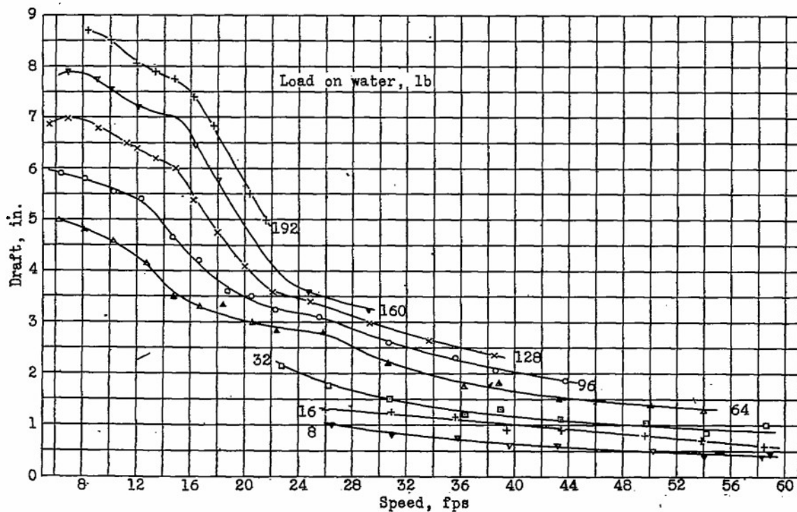
Figure 17.- Model 66. Variation of draft with speed, \tau = 9^\circ .
