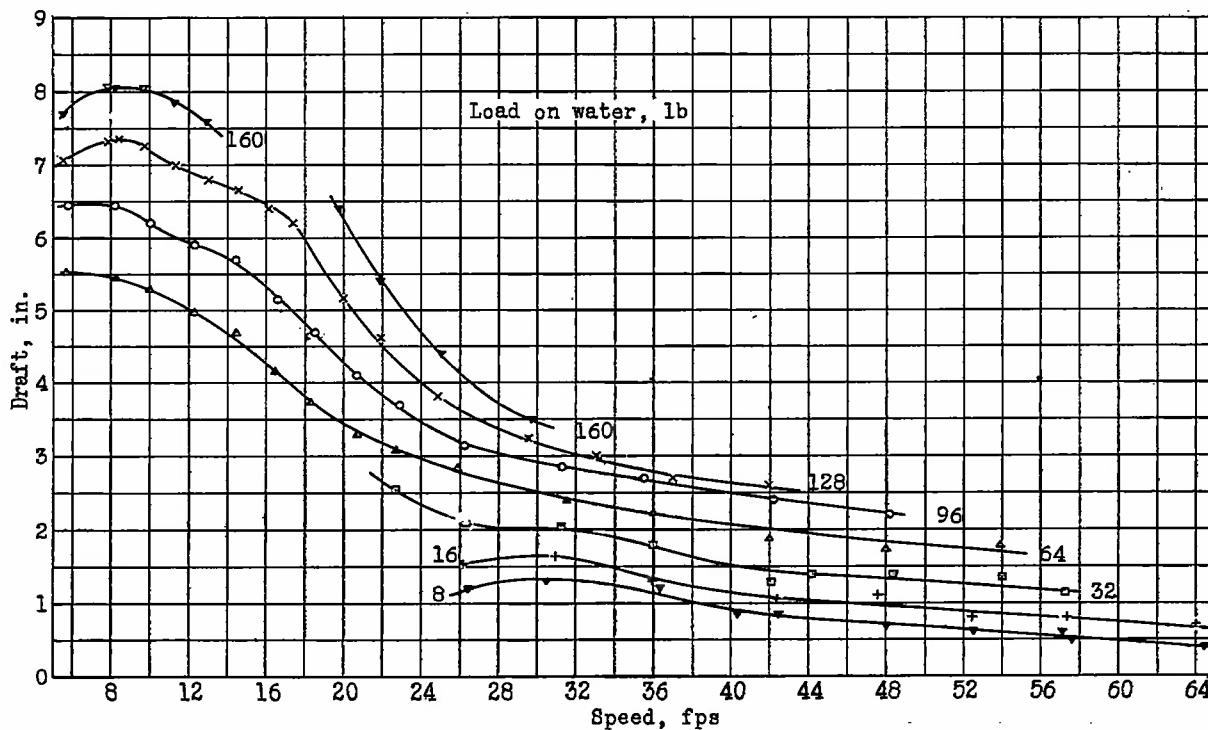
Figure 15.- Model 66. Variation of draft with speed, \tau = 5^\circ .
