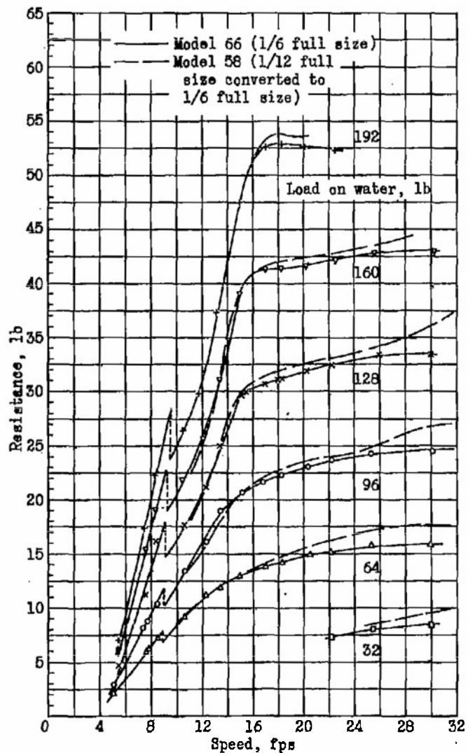
Figure 20.- Models 66 and 58. Variation of resistance with speed, free-to-trim.
