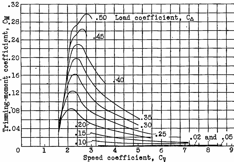
Figure 25.- Model 66. Variation of trimming-moment coefficient at best trim with speed coefficient.
