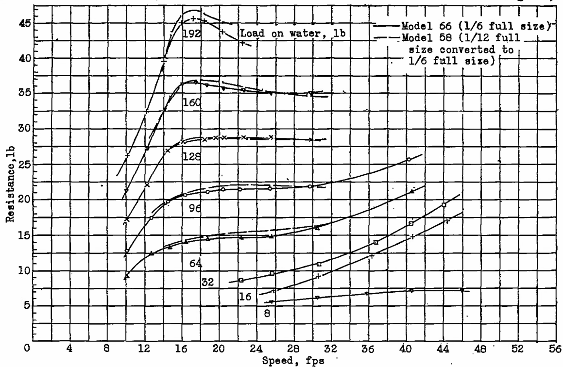
Figure 6.- Models 66 and 58. Variation of resistance with speed, \tau = 11^\circ .
