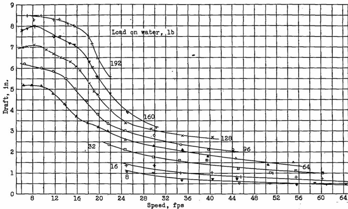
Figure 16.- Model 66. Variation of draft with speed, \tau = 7^\circ .
