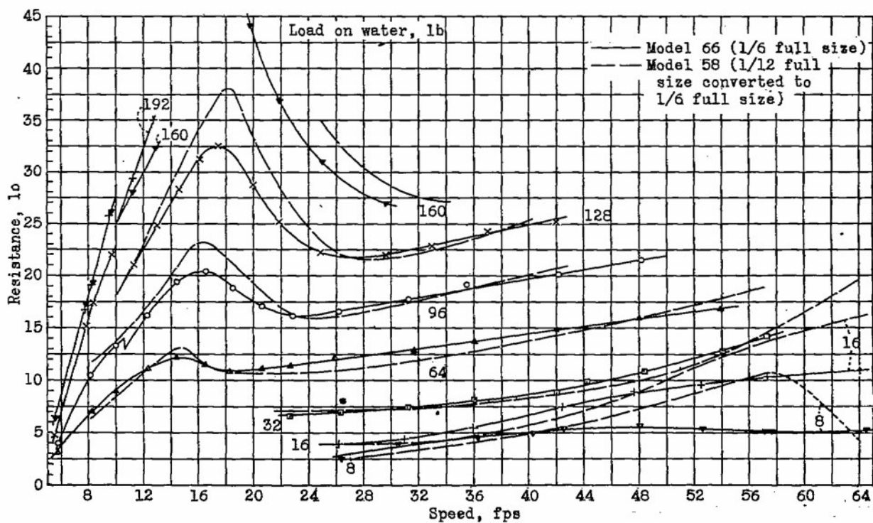
Figure 3.- Models 66 and 58. Variation of resistance with speed, \tau = 50^\circ .
