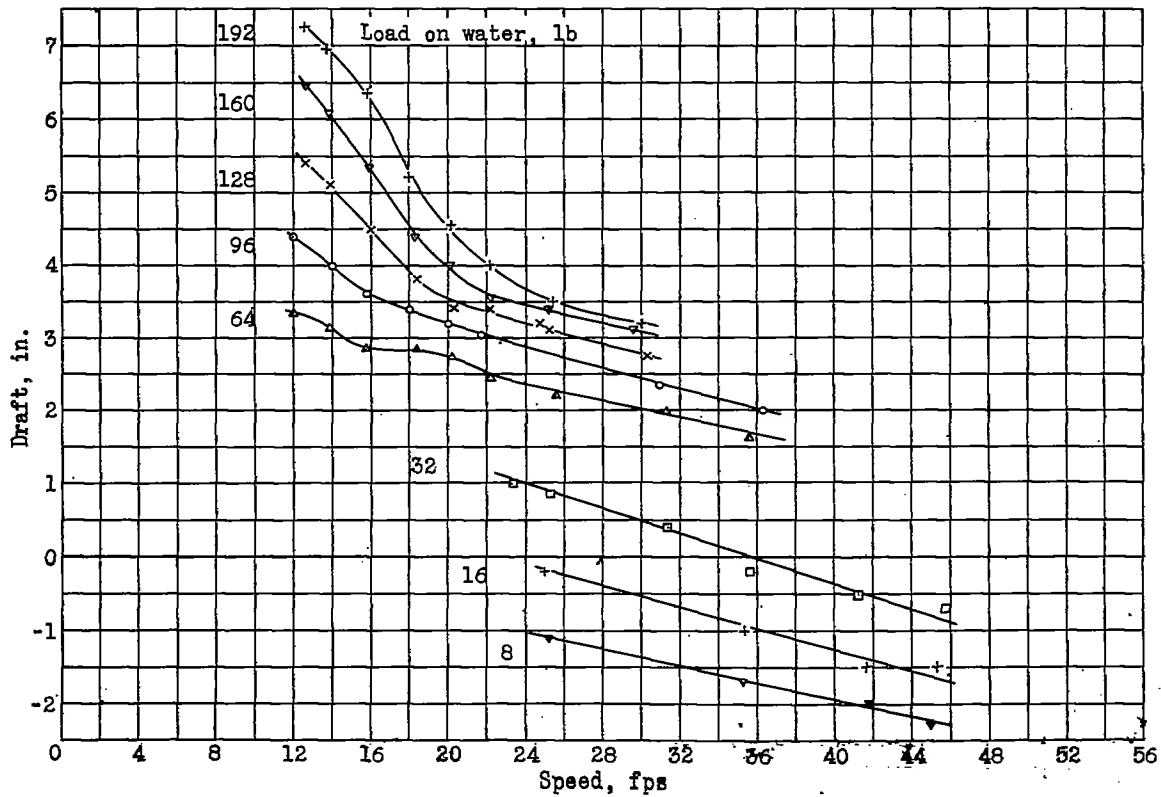
Figure 19.- Model 66. Variation of draft with speed. \tau = 13^\circ .
