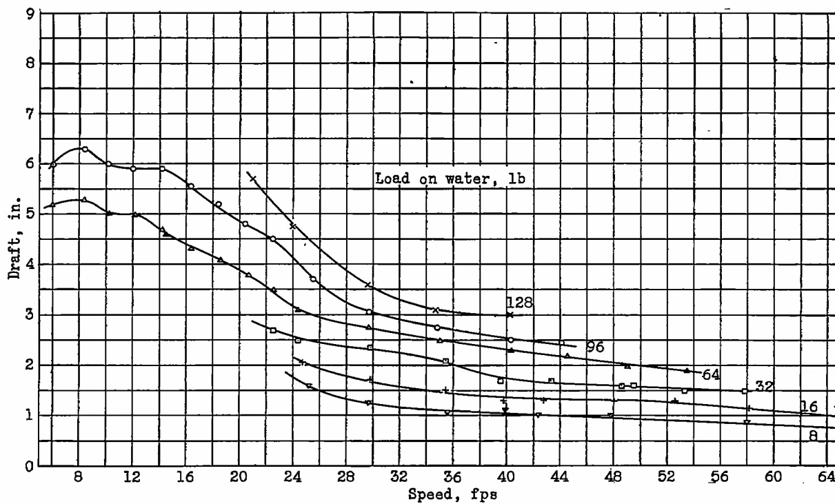
Figure 14.- Model 66. Variation of draft with speed, \tau = 3^\circ .
