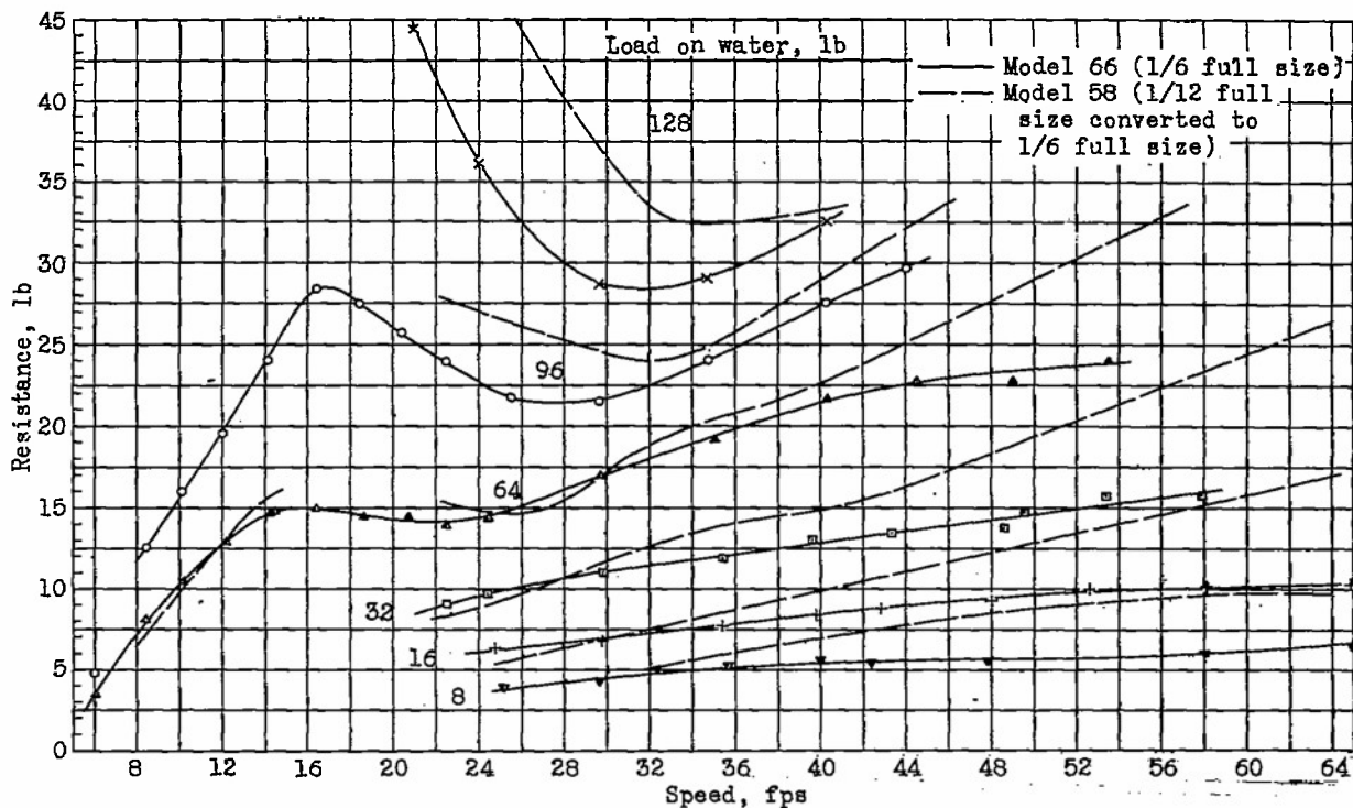
Figure 2.- Models 66 and 58. Variation of resistance with speed, \tau = 30^\circ .
