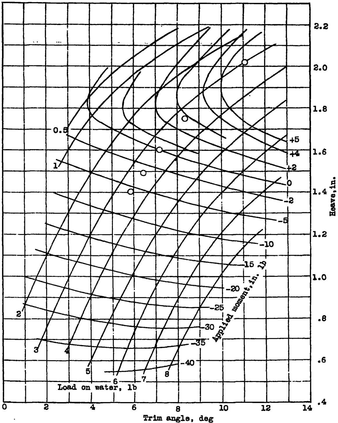
Figure 3.- Steady-motion test data Model No. 204-9. V_m = 15.89 fps
