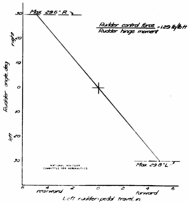
Figure 5. - Variation of rudder angle with rudder-pedal position. Calibrated on the ground with no load on the control surfaces.
