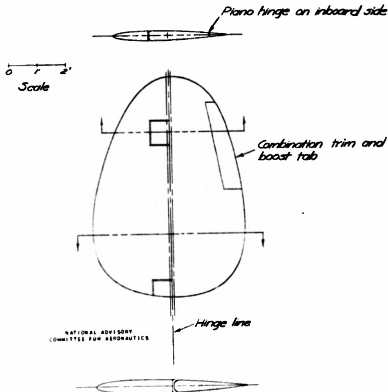
Figure 3. - Sketch of vertical tail surface of the airplane.
