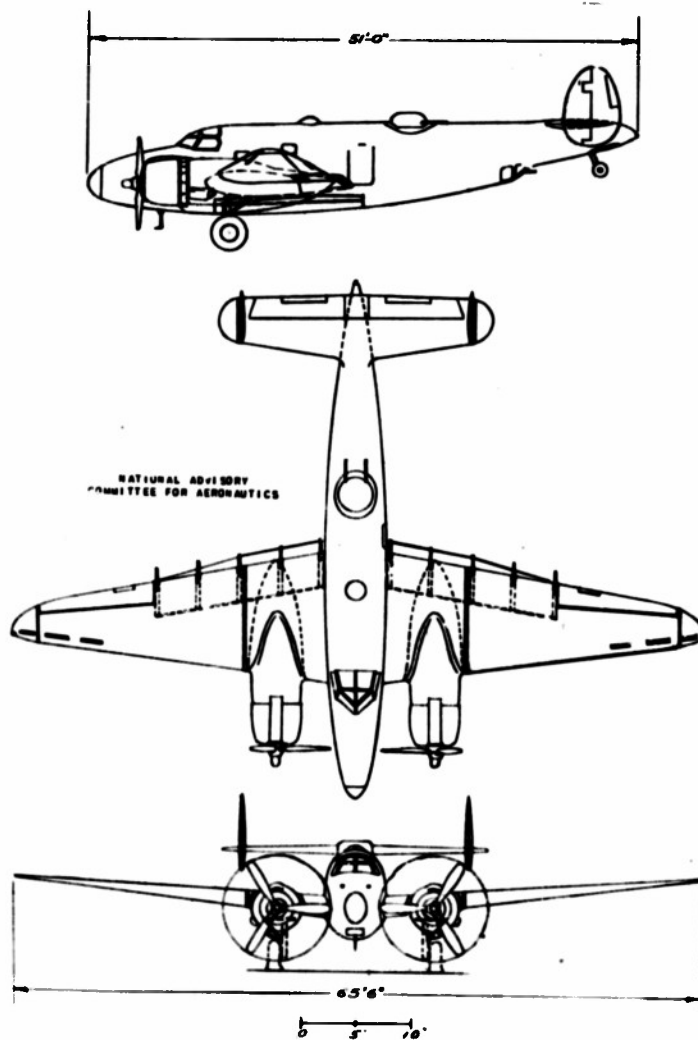
Figure 2.- Three-view drawing of the airplane
