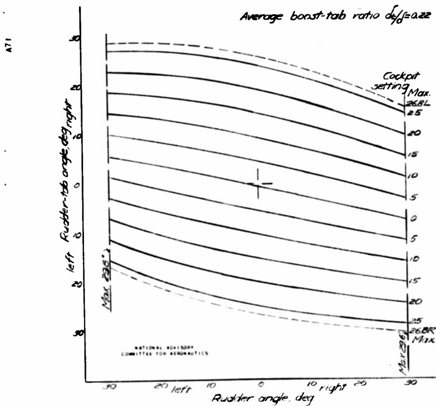
Figure 6. - Variation of rudder-tab angle with rudder angle for different rudder-tab cockpit settings
