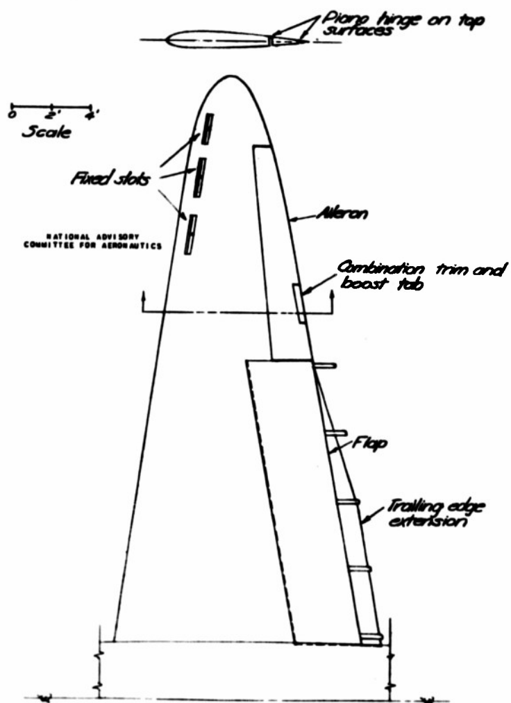
Figure 4 - Sketch of right wing of the airplane
