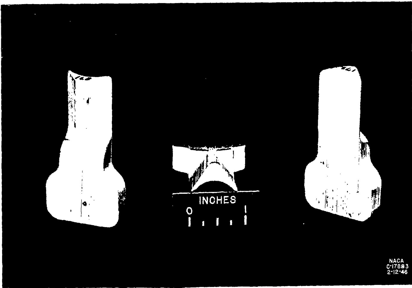
Figure 7. - Second-design blades.
