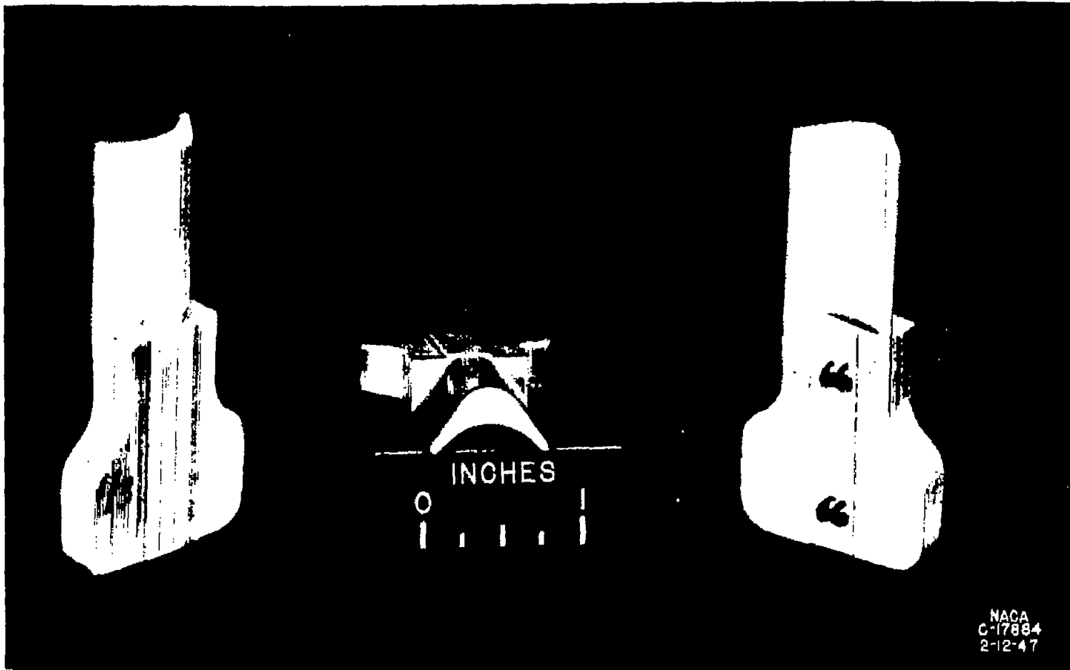
Figure 1. - First-design blades.
