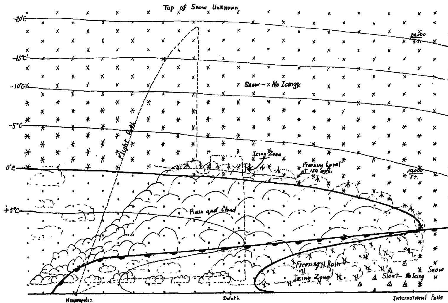
FIGURE 2.- CROSS SECTION OF WARM FRONT CLOUD SYSTEM OVER MINNESOTA ON MARCH 16, 1943 AT ABOUT 9:30 AM. NATIONAL ADVISORY COMMITTEE FOR AERONAUTICS
