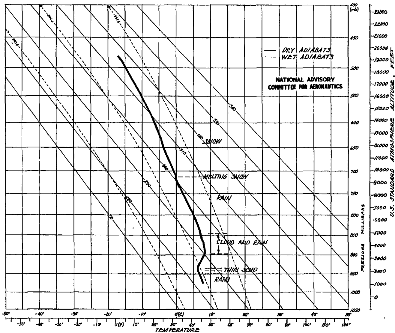
FIGURE 5- DATA OBTAINED FROM AIRPLANE OBSERVATIONS DURING ASCENT BETWEEN MINNEAPOLIS & DULUTH, MINN. ON MARCH 15, 1945 FROM 8:25 TO 9:20 AM.
