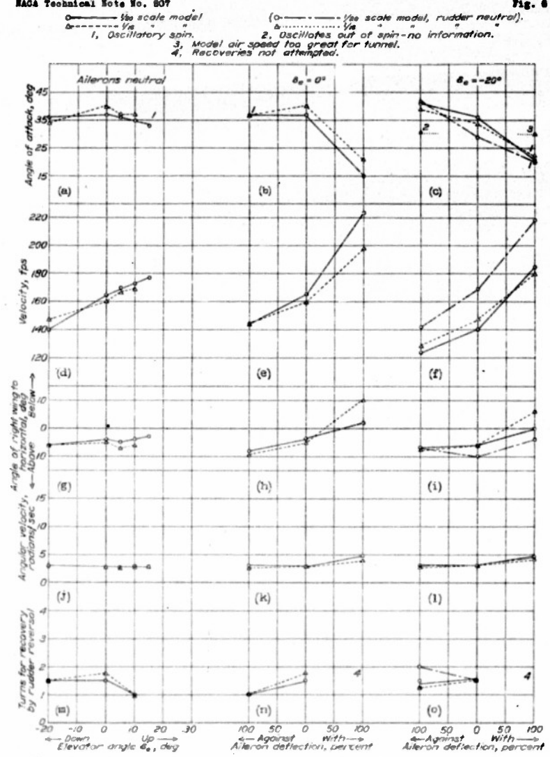
Figure 6.- Effect of scale on two models in the NACA 16-foot free-spinning wind tunnel. Modified load( I_y and I_z increased 30 percent I_y ); rudder 30° with spin; right spine.
