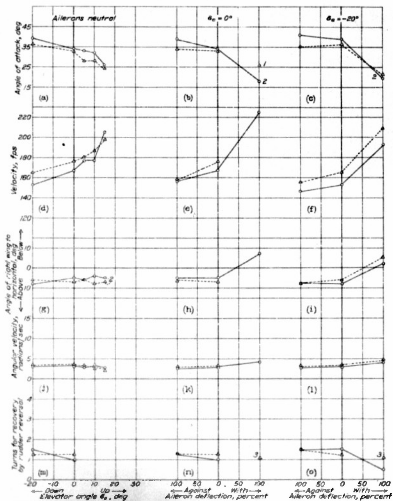
Figure 8.- Effect of scale on two models in the NACA 15-foot free-spinning wind tunnel. Modified load ( I_y and I_z increased 30 percent I_y ); auxiliary fin 2 is in place; rudder 30° with spin; right spine.
