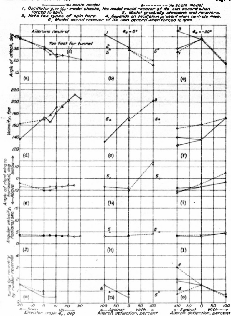
Figure 4.- Effect of scale on two models in the NACA 15-foot free-spinning wind tunnel. Normal load; auxiliary fin 1 in place; rudder 30^\circ with spin; right spins.
