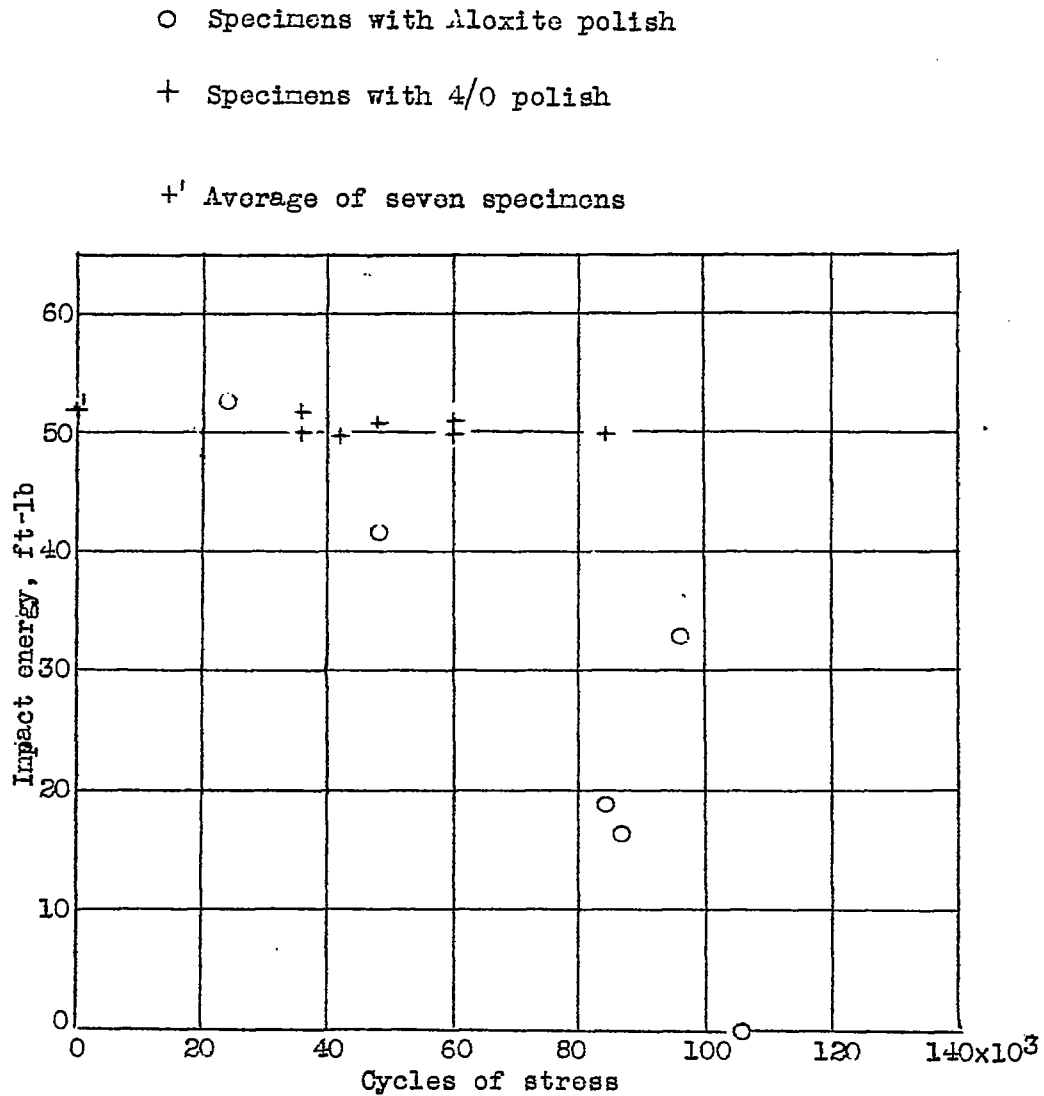
Figure 5.- Impact energy absorbed at room temperature in tensile impact tests of specimens of normalized S.A.E. X4130 steel (batch 1) fatigue-stressed by axial loading in the Haigh machine from 28,800 pounds per square inch compression to 63,000 pounds per square inch tension for various numbers of cycles. Minimum diameter, 0.200 inch.
