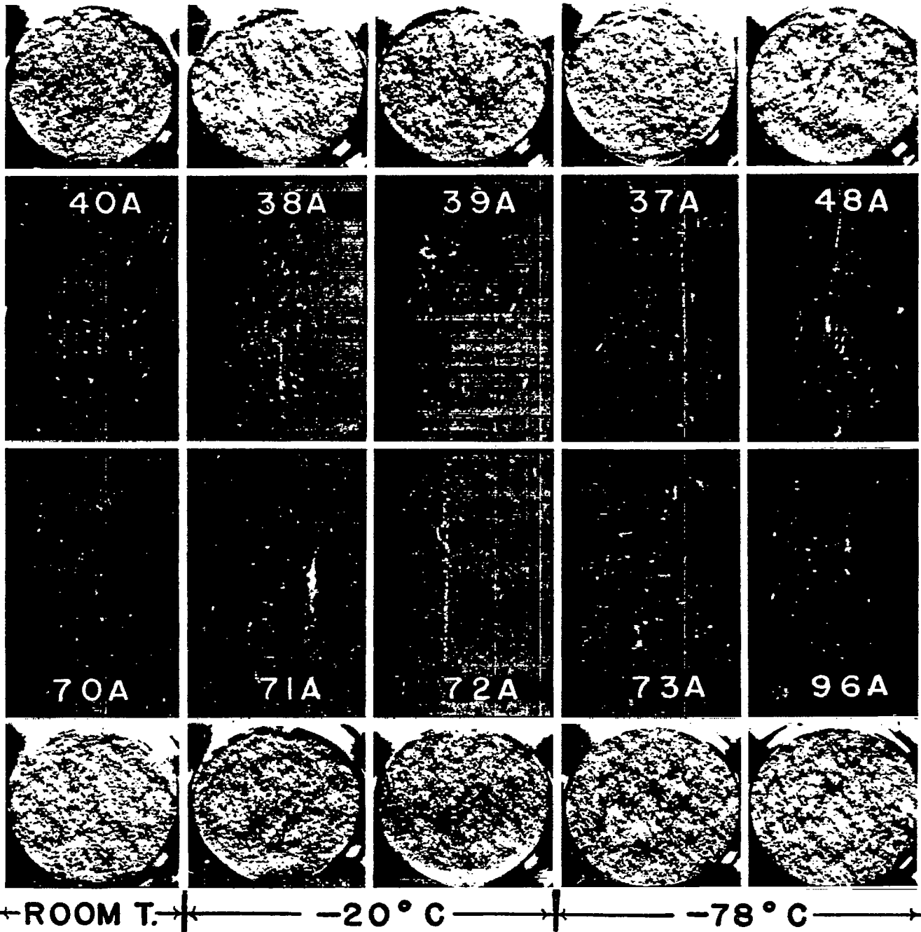
Figure 23.- Notched fatigue specimens of normalized S.A.E. x4130 steel (batch 4) stressed at \pm 40,000 pounds per square inch as rotating cantilever beams for 50,000 cycles in the Krouse machine.
