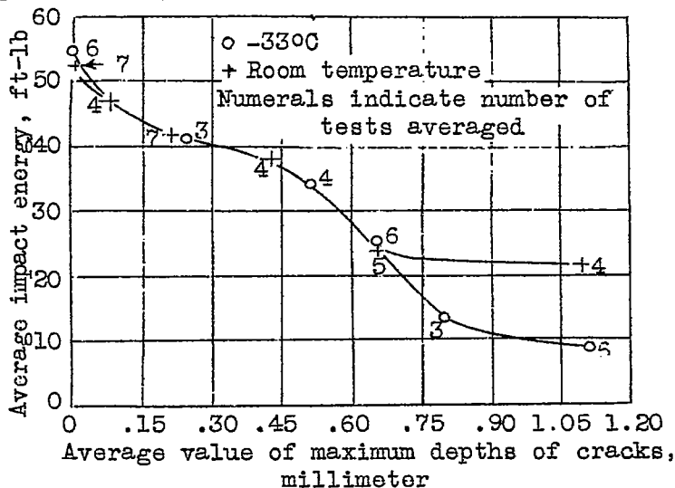
Figure 15.- Variation of average tensile impact energy with average maximum depth of the fatigue crack in fatigued specimens of normalized S.A.E. X4130 steel (batches 3,6, and 9) fatigue-stressed under axial loading in the Haigh machine.
