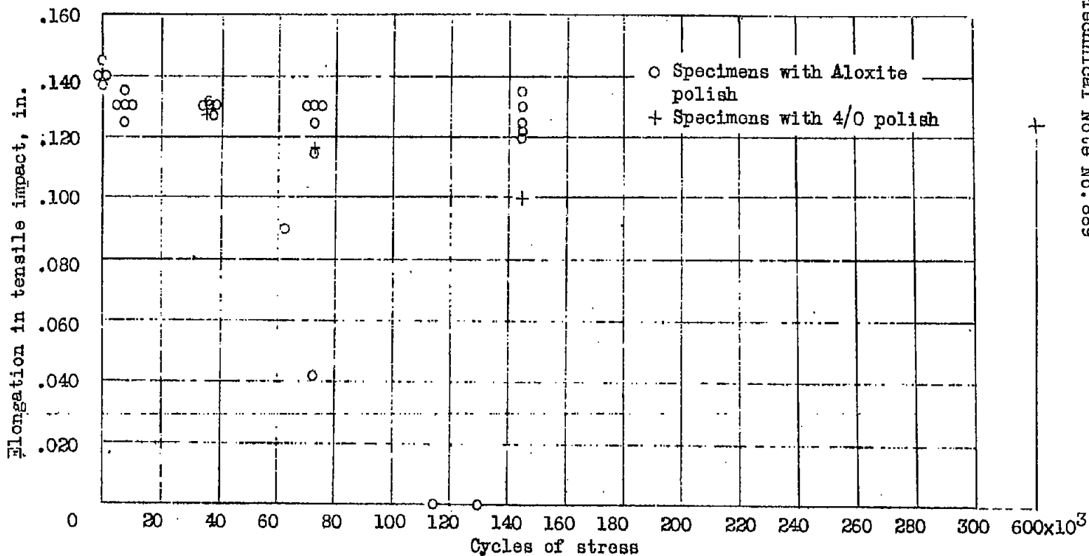
Figure 7.- Elongation in 2-inch gage length during tensile impact tests at -33^{\circ}\text{C} of specimens of normalized S.A.E. 4130 steel (batch 9) after fatigue-stressing under axial loading in the Haigh machine in tension ranging from 10,500 to 89,500 pounds per square inch (mean stress, 50,000 lb/sq in.).
