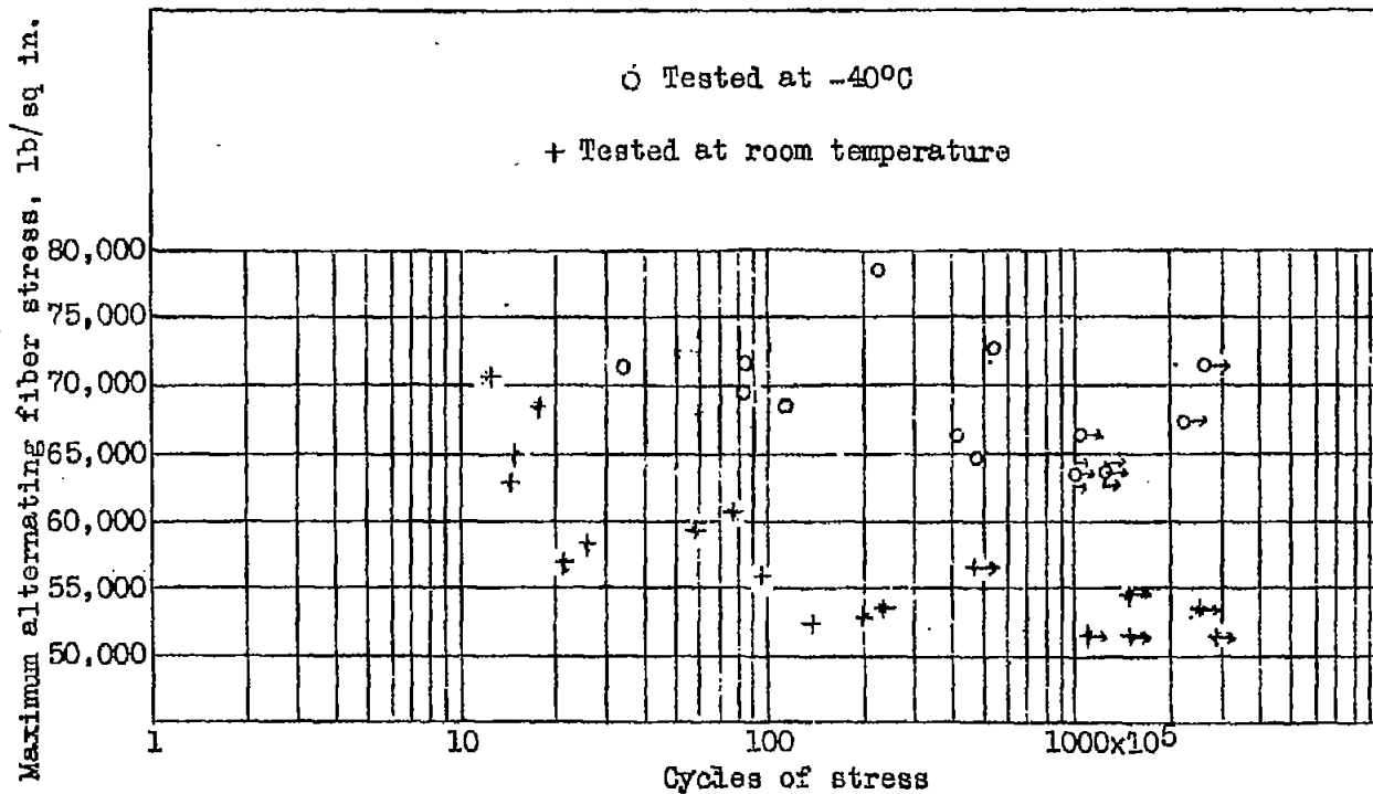
Figure 22.- Fatigue strengths for specimens of normalized S.A.E. X-4130 steel tested by repeated flexure in the Rayflex machine at room temperature and at -40^{\circ}\text{C} .
