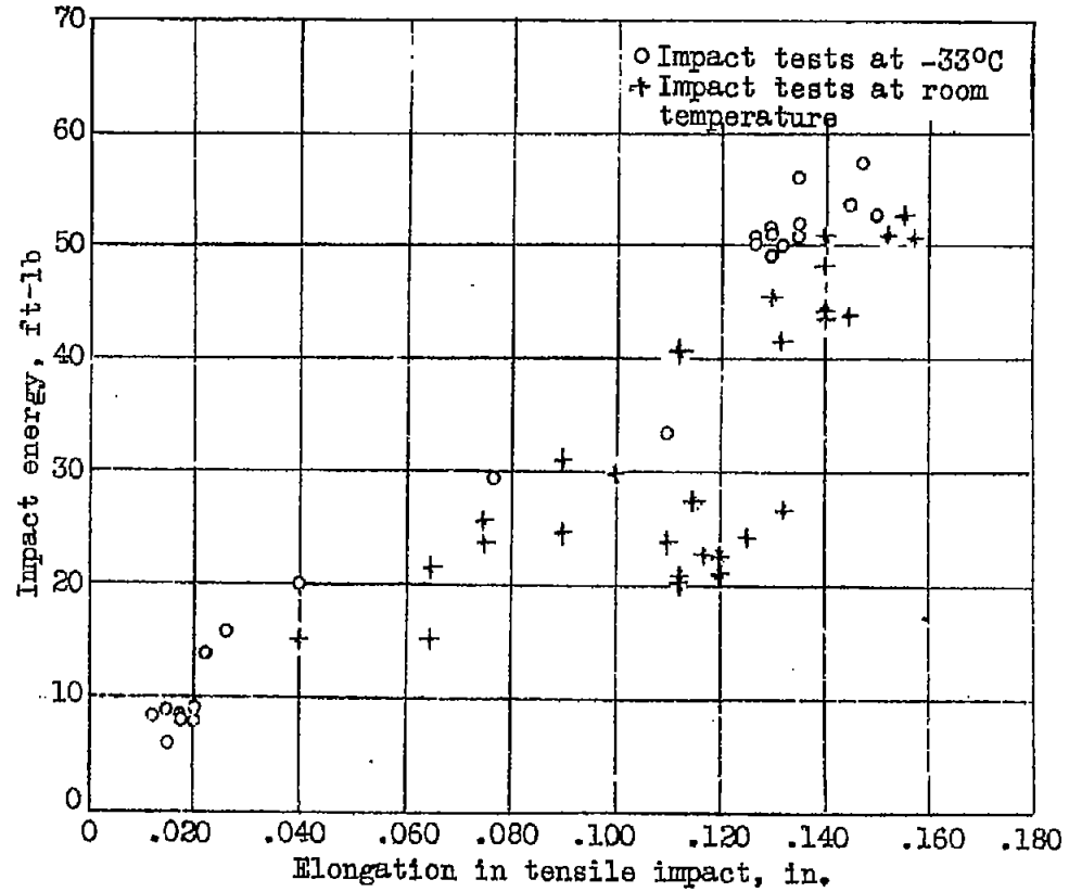
Figure 14.- Relationship between impact energy and elongation in tensile impact tests of specimens of normalized S.A.E. X4130 steel (batch 6) after fatigue-stressing under axial loading in the Haigh machine.
