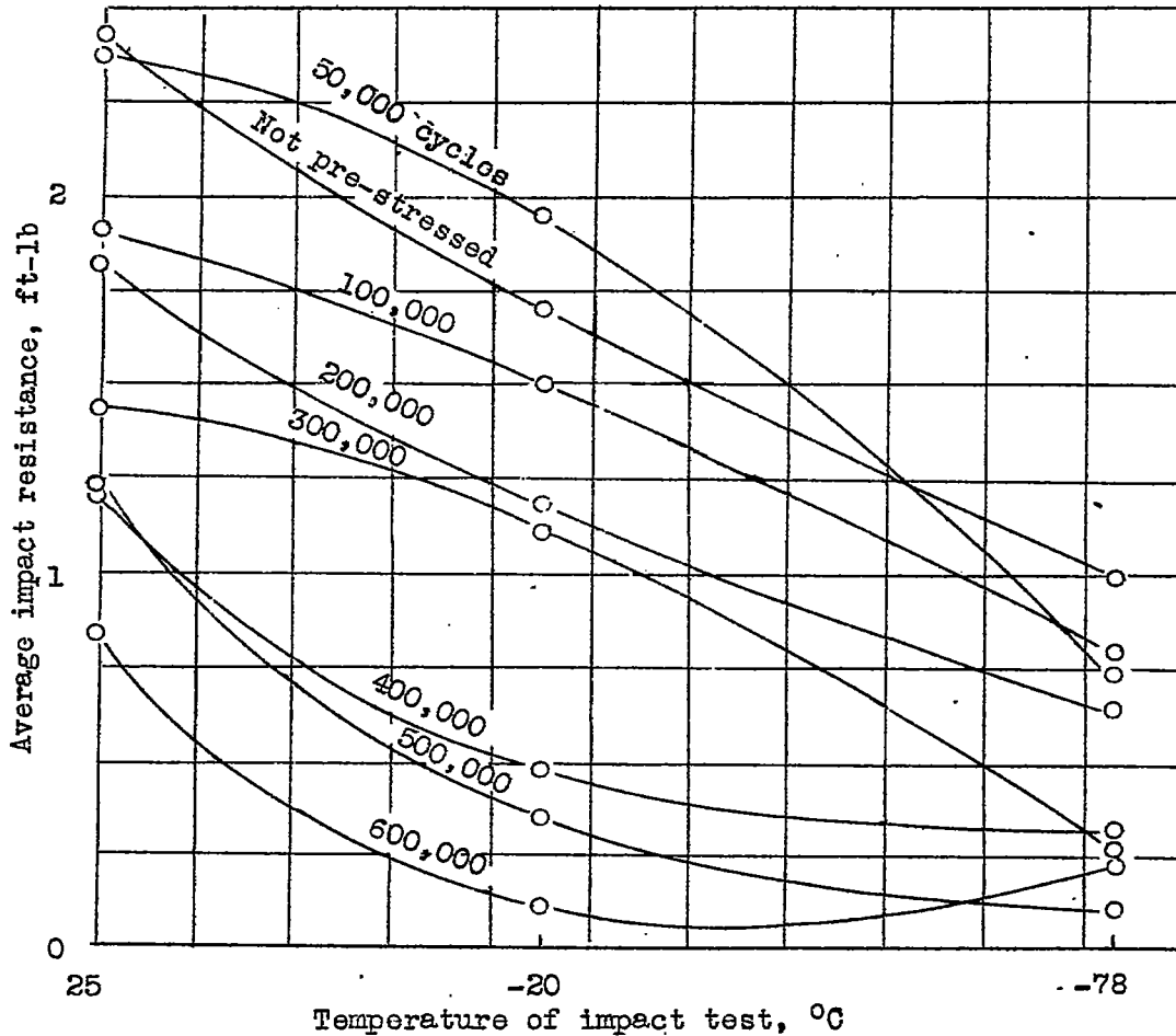
Figure 1.- Effect of temperature on the average transverse impact resistance of notched specimens of normalized S.A.E. X4130 steel (batch 4) after repeated stressing as rotating cantilever beams in the Krouse machine. Nominal stress amplitude, \pm 40,000 pounds per square inch; nominal fatigue limit, 26,600 pounds per square inch. Each point on the 25°C line represents two to four specimens; all other points each represent four specimens.
