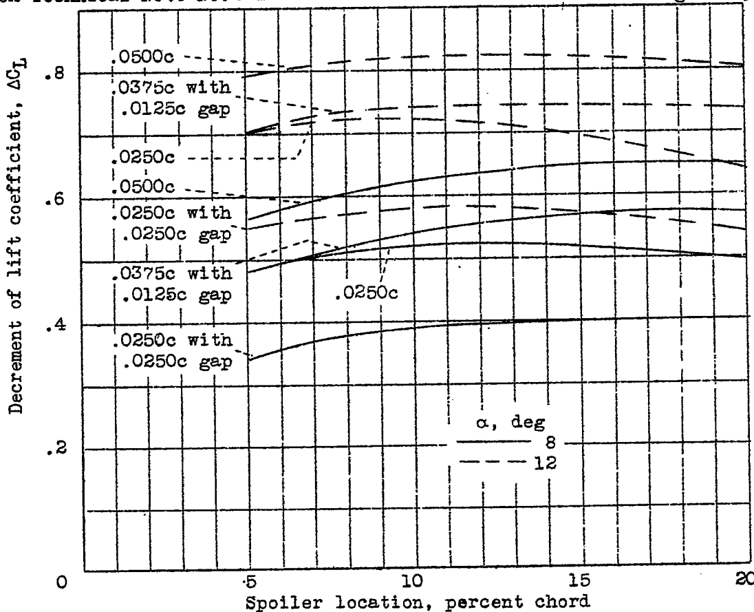
Figure 10.- Effect on lift coefficient of location of flat spoilers.
