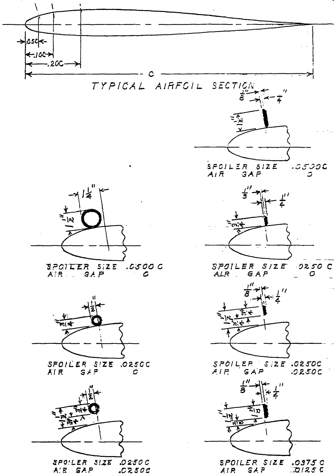
FIGURE 2 - SPOILER ARRANGEMENTS AND LOCATIONS,
