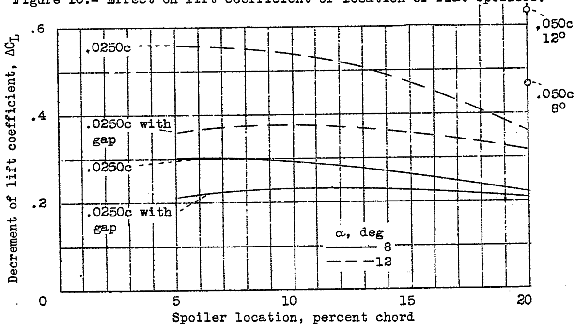
Figure 11.- Effect on lift coefficient of location of round spoilers.
