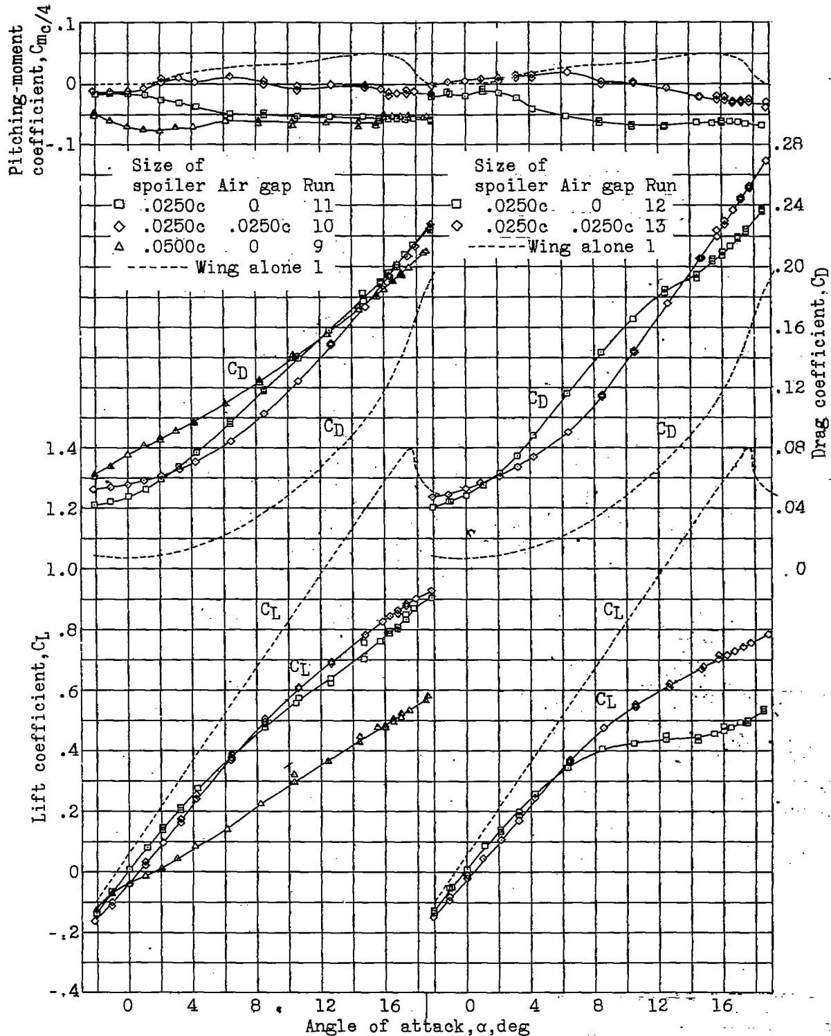
Figure 9.-20-percent-chord location. Figure 8.-10-percent-chord location. Figures 8,9.- Effects of round spoilers.
