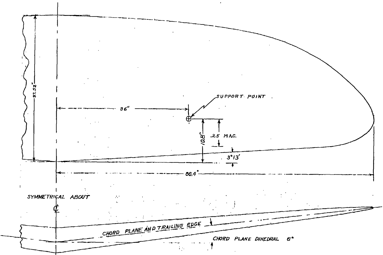
FIGURE 1. - PLAN AND ELEVATION OF WING.
