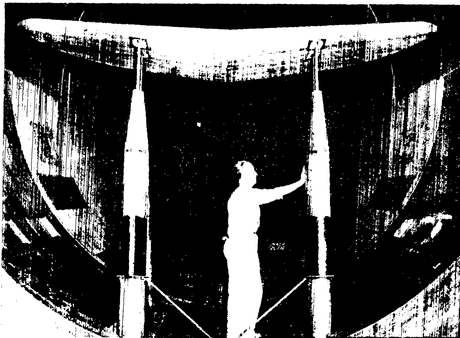
Figure 3.- Wing model mounted for test in the NACA 19-foot pressure wind tunnel.
