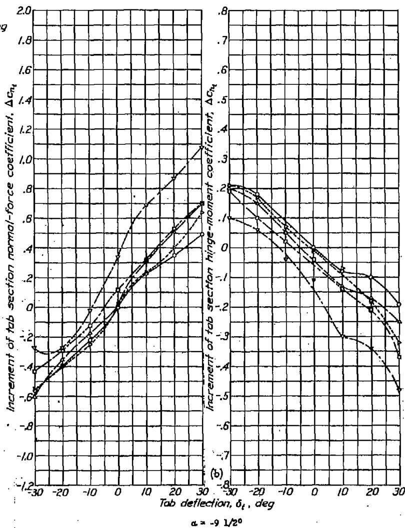
Figure 13, a to f.- Increments of tab section normal-force and hinge-moment coefficients for various deflections of an 0.80c plain flap and a 0.10c t tab.
