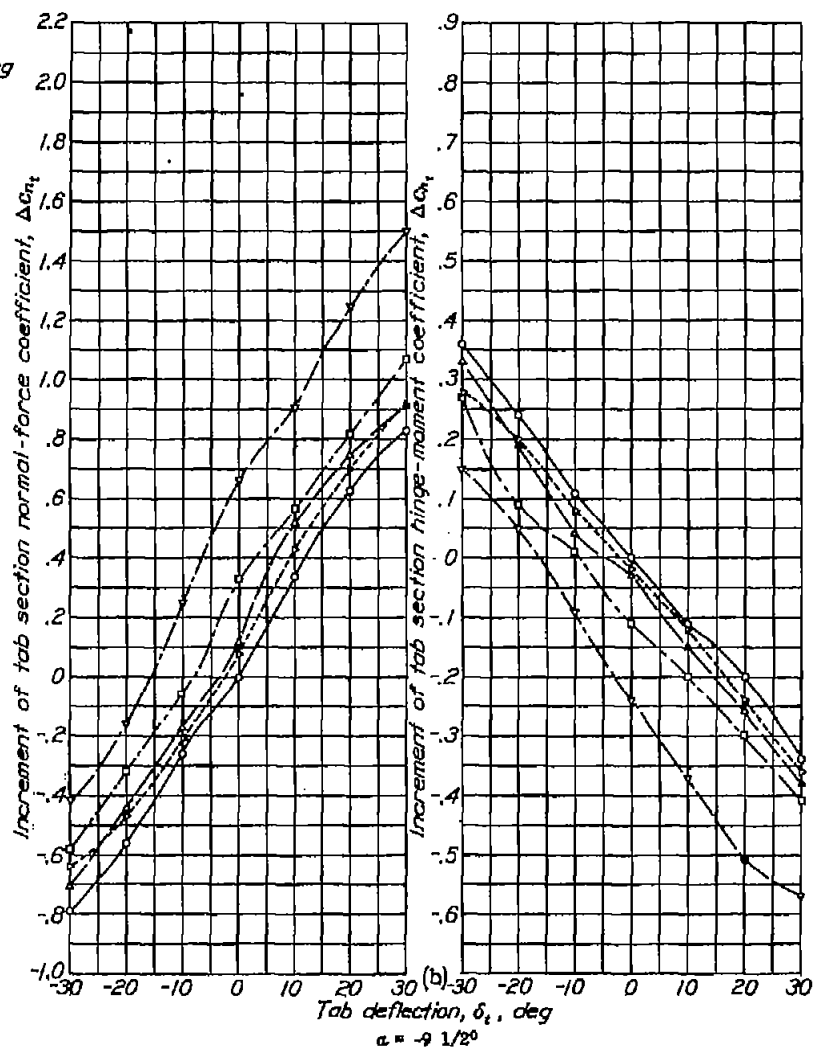
Figure 19, a to f.- Increments of tab section normal-force and hinge-moment coefficients for various deflections of a 0.80c plain flap and a 0.80c f tab.
