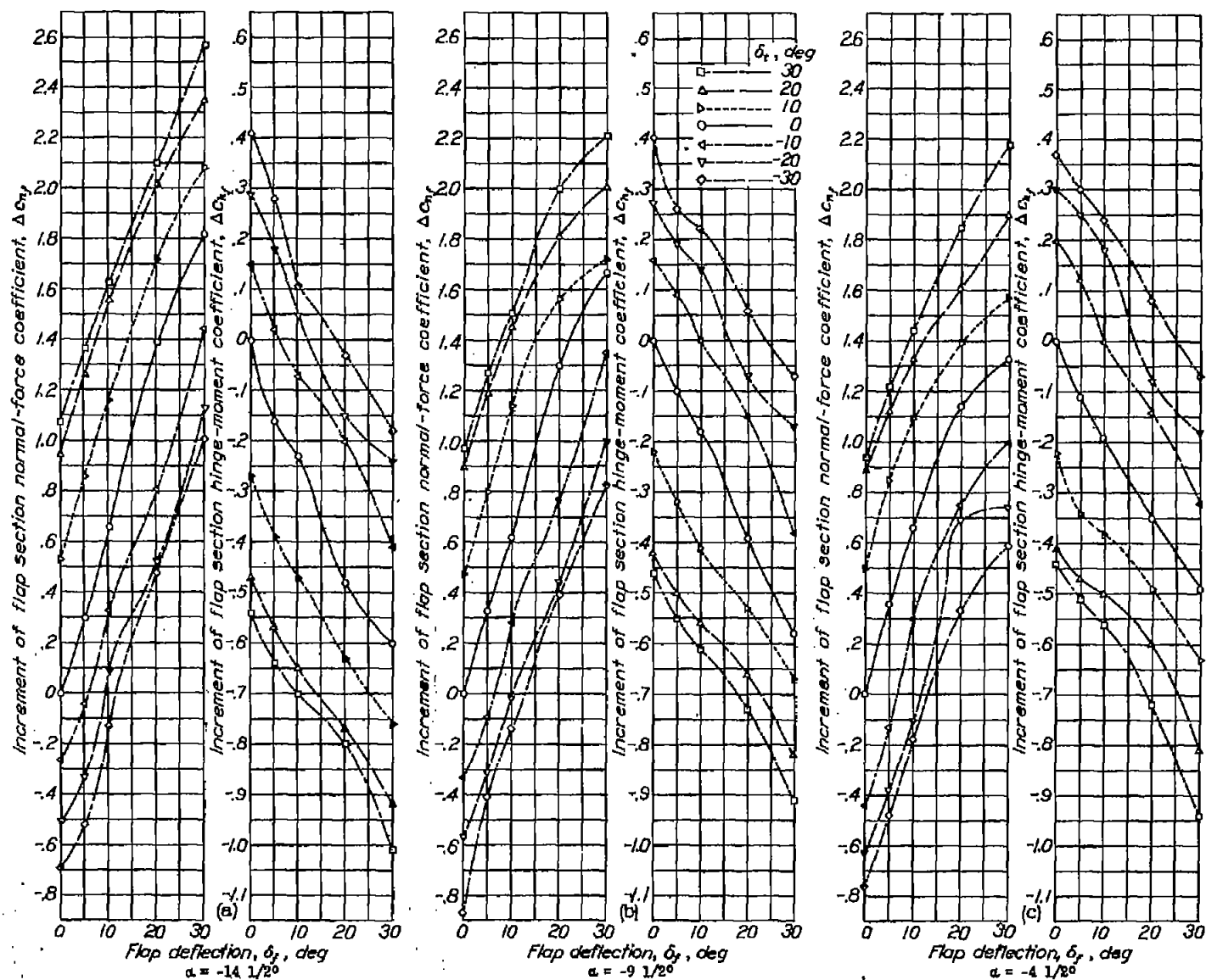
Figure 18, a to f.- Increments of flap section normal-force and hinge-moment coefficients for various deflections of a 0.80c plain flap and a 0.30c tab.
