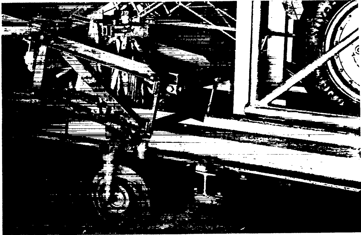
Figure 4.- Castoring wheel and frame attached to N.A.C.A. tank towing carriage.
