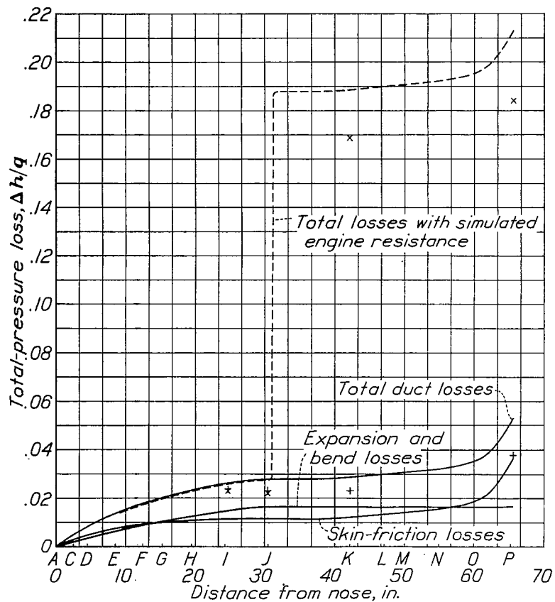
Figure 15.- Nose 2, tail 2.
