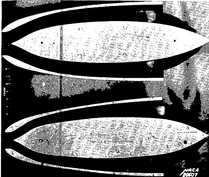
Figure 9.- Duct details showing crankcase fairing. Wall cut at 22.5-inch station. Nose 1.
