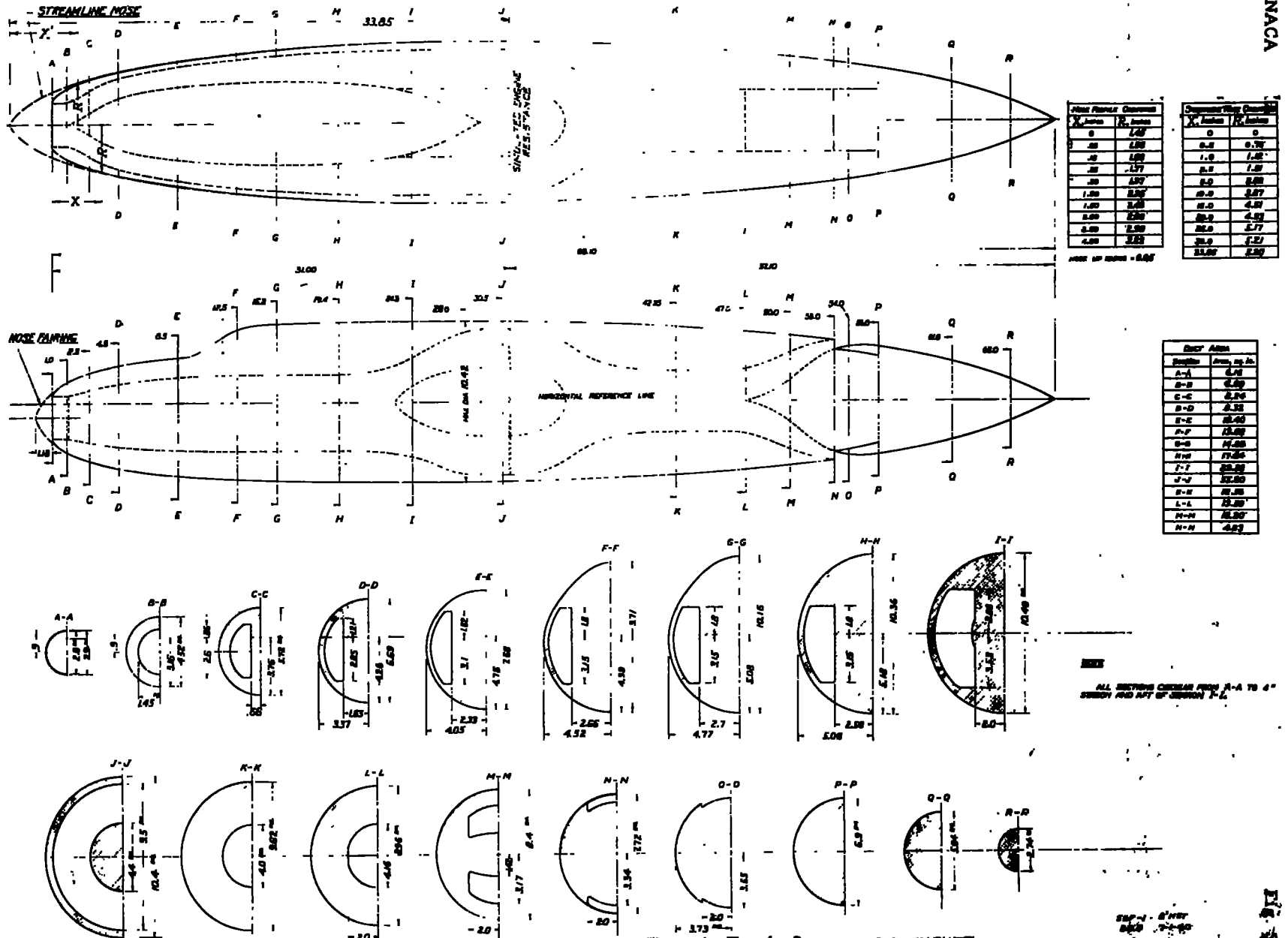
FIGURE 3-FUSELAGE DETAILS. NOSE 1, TAIL 1. DIMENSIONS IN INCHES
