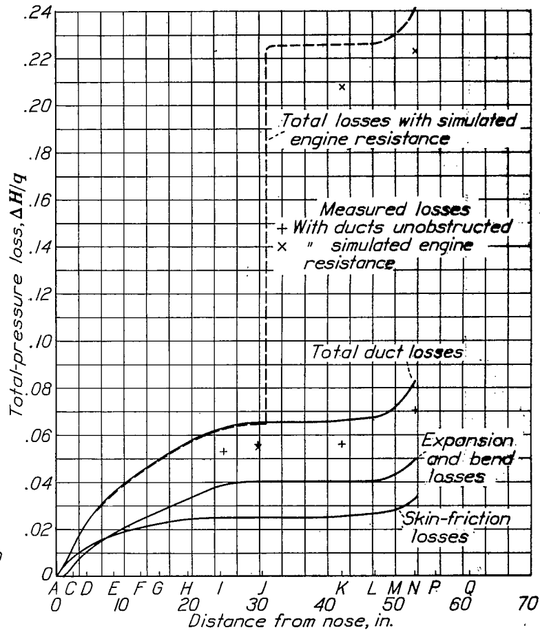
Figure 14.- Nose 1, tail 1.
