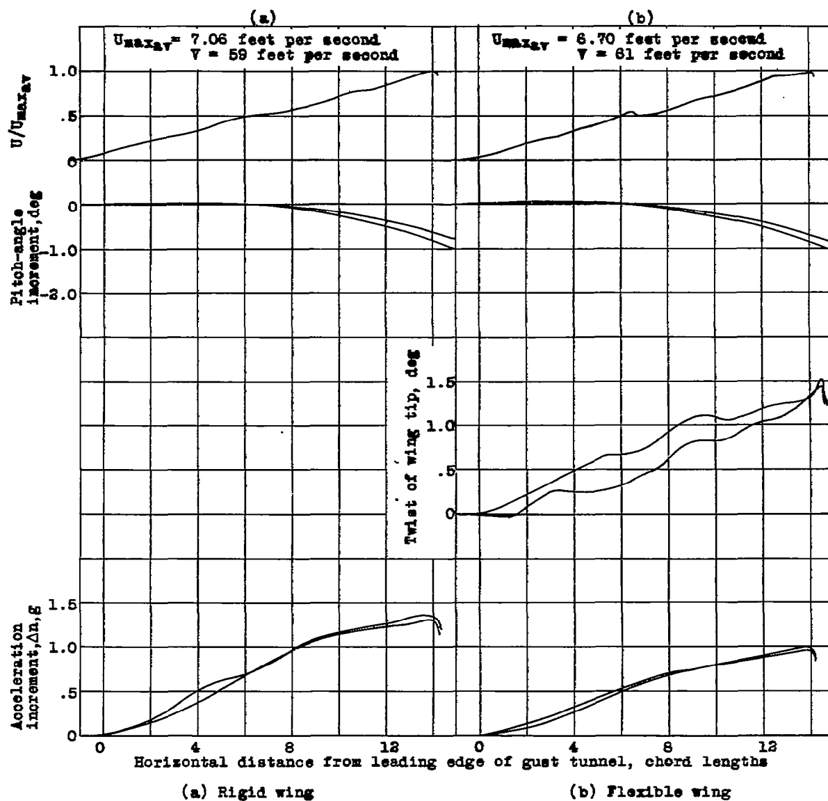
Figure 11.- Histories of events in a 15-chord-length gust.
