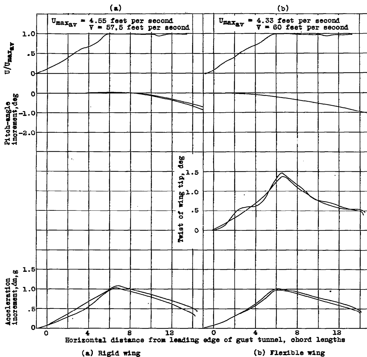
Figure 10.- Histories of events in a 8.8-chord-length gust.
