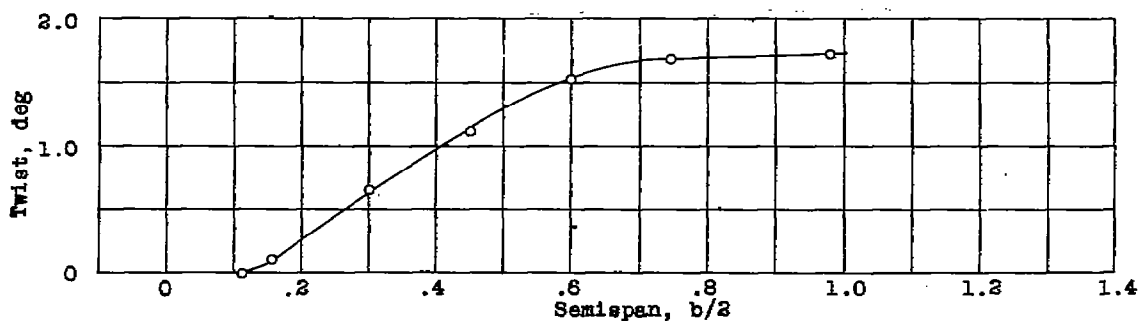
Figure 5.- Wing-twist increment. Load-factor increment, 1.0; flexible wing.
