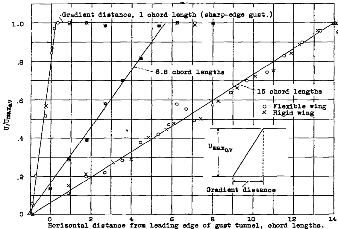
Figure 1.- Velocity distribution through jet.
