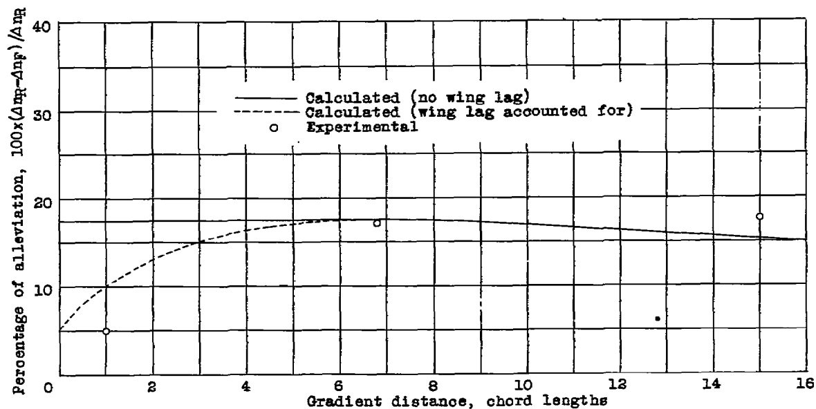
Figure 13.- Variation of wing effectiveness with gradient distance.
