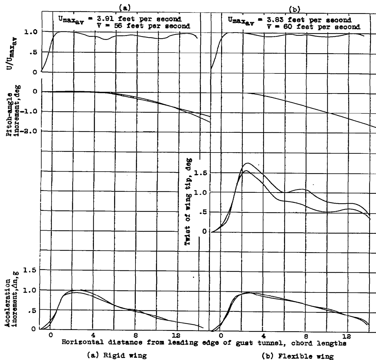
Figure 9.- Histories of events in a 1-chord-length gust(sharp edge).
