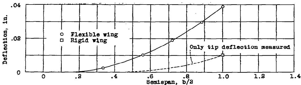
Figure 6.- Static-wing deflection curves. Load factor, 1.0.
