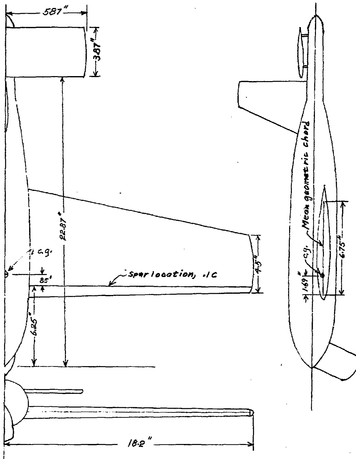
Figure 3.- Line drawing of airplane model.
