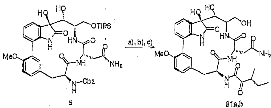
Scheme 15. Synthesis of derivatives 31a,b. a) Pd/C, \text{H}_2 , EtOH, rt; b) ( \pm )-3-methyl-2-oxopentanoic acid (21), EDC/HOAT, \text{CH}_2\text{Cl}_2/\text{DMF} , rt; c) HF/Py.
