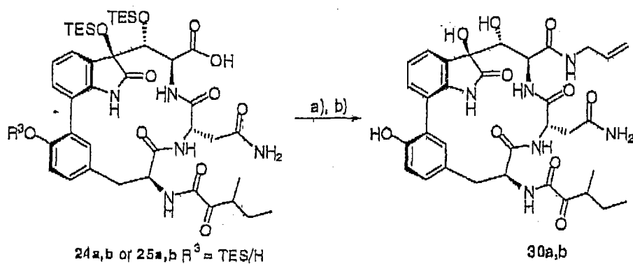
Scheme 14. Synthesis of derivatives 30a,b. a) allyl amine, EDC/HOAT, \text{CH}_2\text{Cl}_2/\text{DMF} ; b) HF/Py, THF/Py; then \text{Me}_3\text{Si-OMe} .
