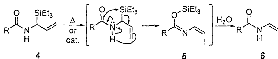
Scheme 9: Formation of cis -propenamides 6 via rearrangement-hydrolysis of \alpha -silylallyl amides 4 (R = aromatic, alkenyl, and alkyl groups).
