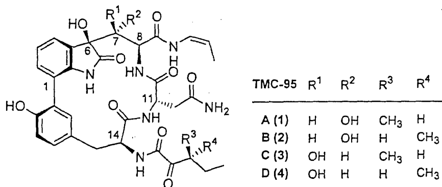
Figure 1: Structures of TMC-95A, B, C, and D (1-4).
