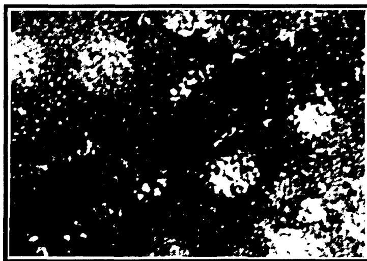
(3). ( \alpha\beta_{III} + 20 \mu\text{M VBL} + \text{Tau} )
