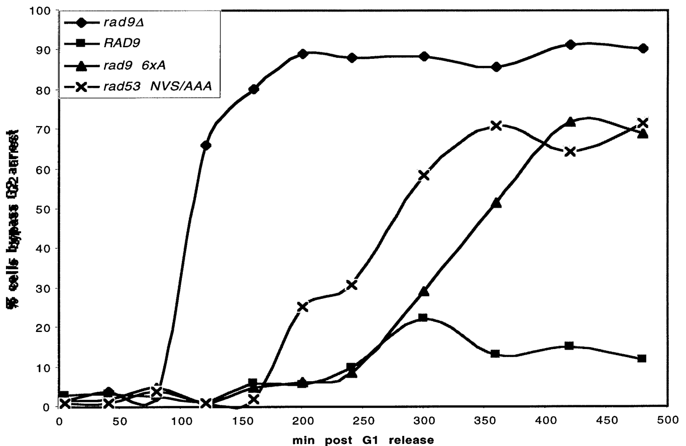
Figure 7: rad9 6xA mutants fail to maintain the G 2 cell cycle arrest after rDNA damage. Cells are synchronized in G 1 and released at 37°C. DNA damage accumulates in S phase due to the temperature sensitive cdc13-1 allele in these strains. Cells with a deficient DDC fail to maintain the G 2 arrest, proceeding with mitosis. rad9 6xA cells escape G 2 arrest with kinetics similar to the rad53 NVS/AAA FHA2 mutant cells.
