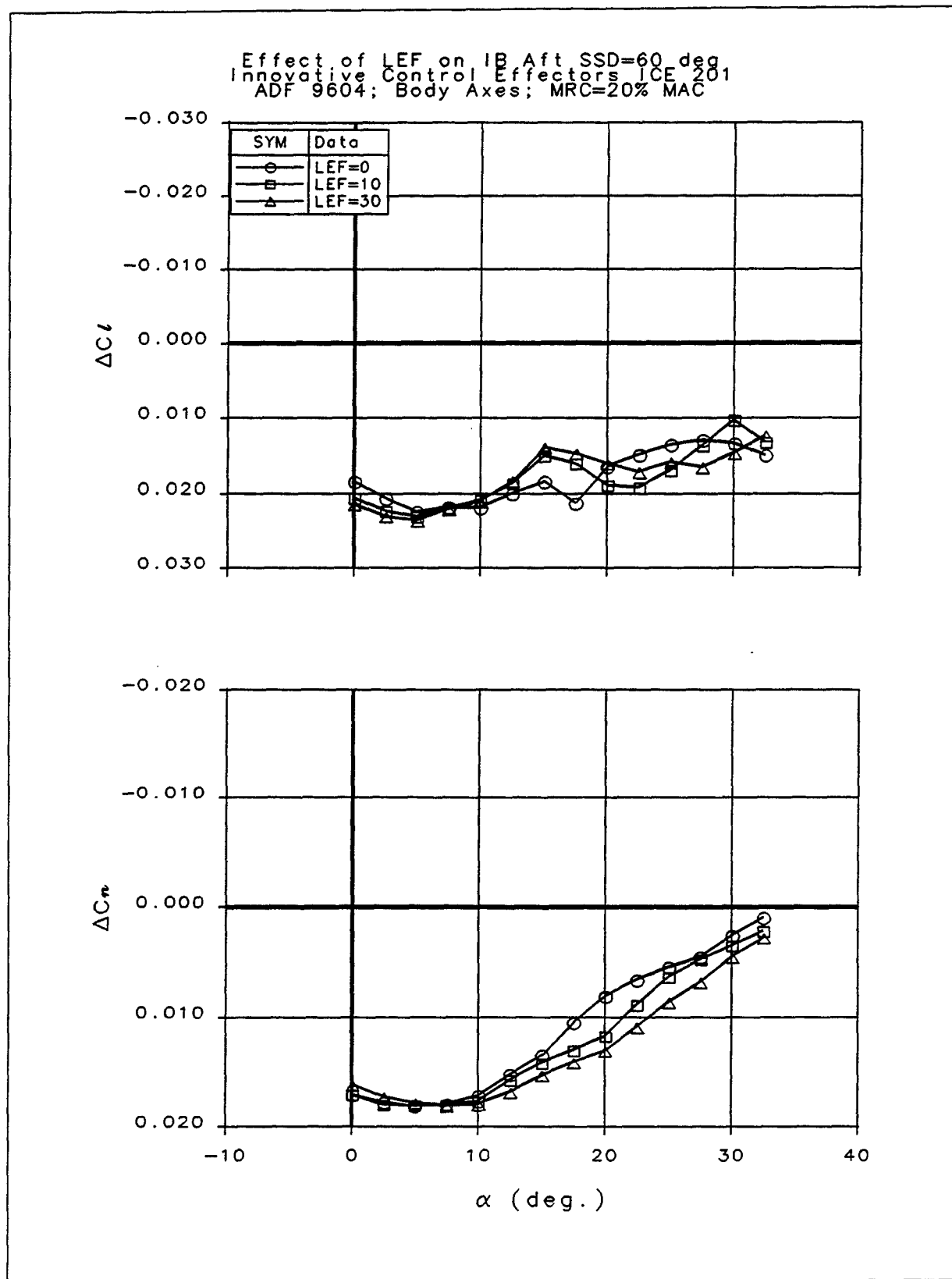
Figure 2-67: LEF Effects on SSD Control Power
