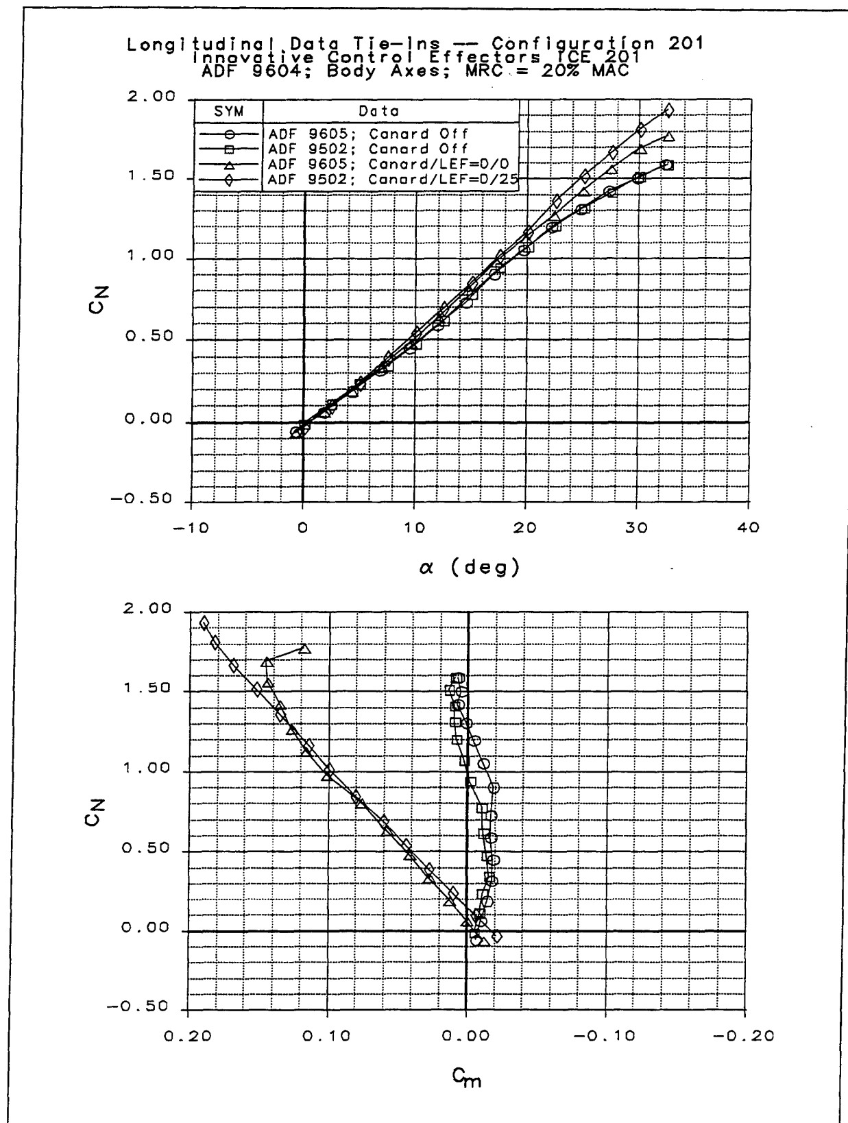
Figure 2-44: Longitudinal Characteristics of Configuration 201
