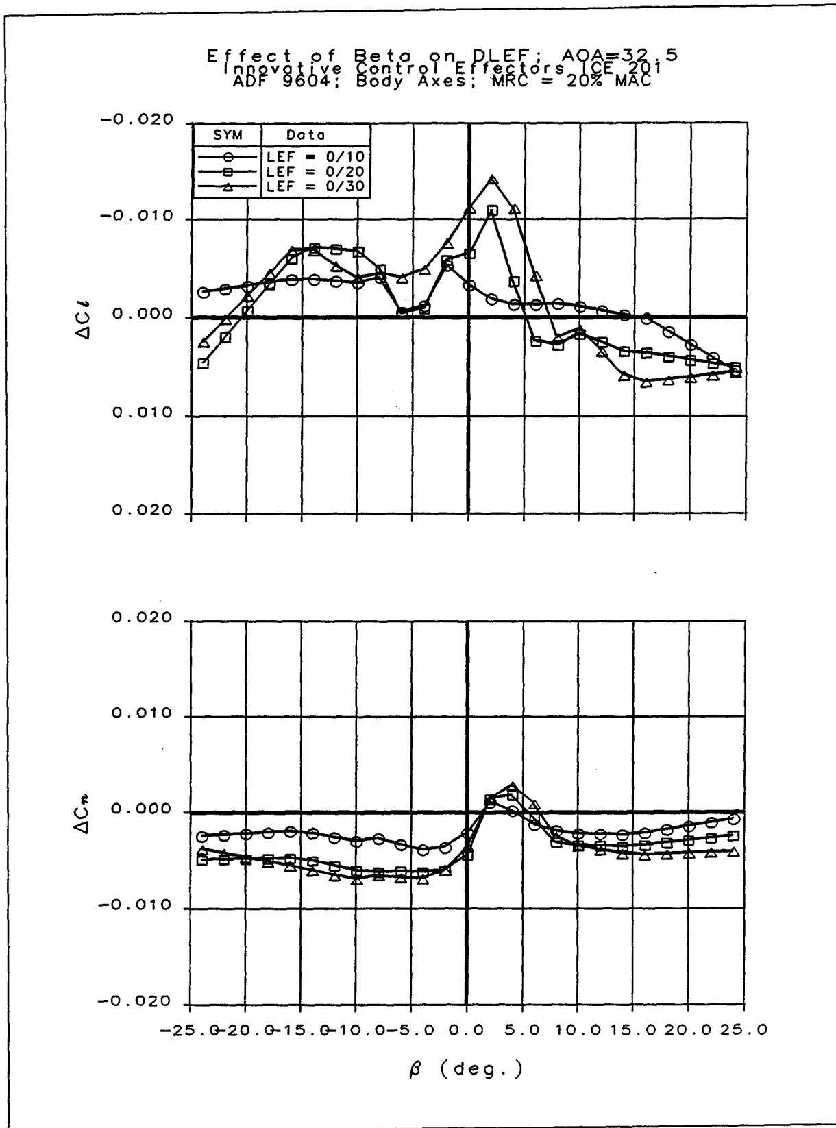
Figure 2-71: Effect of Sideslip on DLEF Effectiveness; AOA = 32.5°
