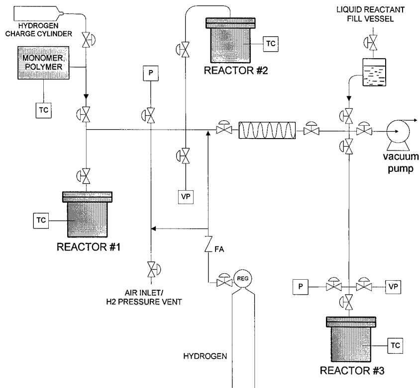
FIGURE 2 - Diagram of Activation and In Situ Polymerization Coating System (TC=thermocouple; P=pressure gage; VP=vacuum pressure gage; FA=flash arrester)
