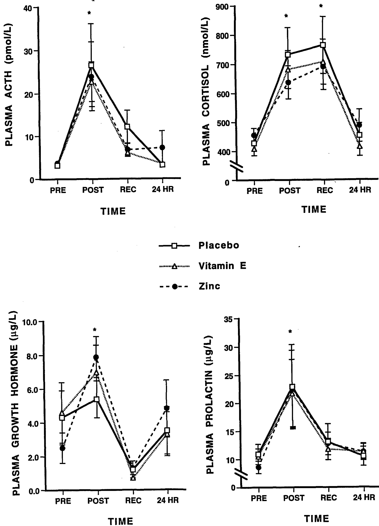
Figure 3. Plasma adrenocorticotropin hormone, cortisol, growth hormone and prolactin concentrations for zinc, vitamin E and placebo conditions. *Significant exercise effect ( p < 0.05 ).
