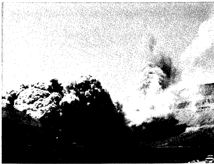
There was essentially no cloud rise. The sandbag stemming and the material scoured from the tunnel itself stayed close to the ground.
