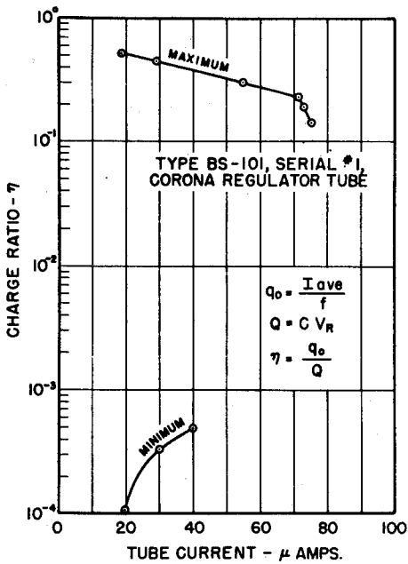
Figure 7. Maximum and Minimum Charge Ratio Limits, for Stable Operation, versus Corona Tube Current
