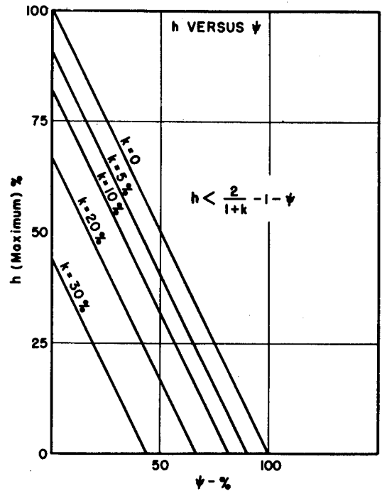
Figure 9. Design Sheet for Corona Regulator Circuit, h versus \psi .
