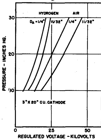
Figure 4. Firing Voltage versus Pressure for Air and Hydrogen
