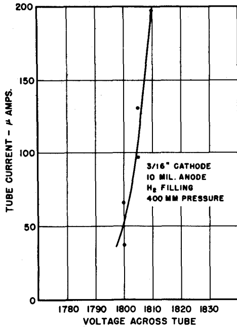
Figure 11. Discharge Characteristic of Sub-Miniature Tube.
