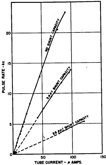
Figure 6. Pulse Rate versus Corona Tube Discharge Current
