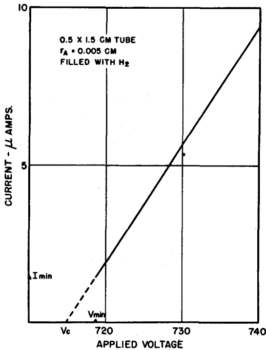
Figure 1. Corona Discharge Characteristic
