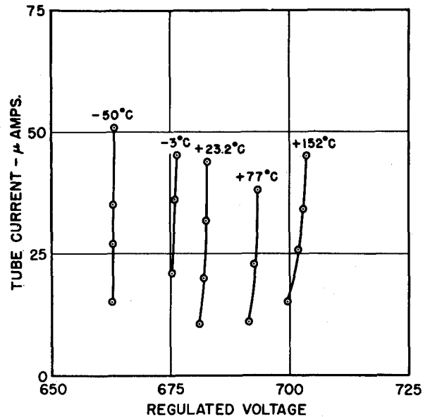
Figure 13. Temperature Influence upon Discharge Characteristic of Miniature, Type BS-101, Corona Voltage Regulator Tube
