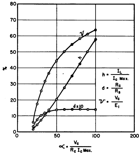
Figure 10. Corona Regulator Circuit Relationships for Maximum Efficiency. ( k = 10\% , \beta = 1\% ).
