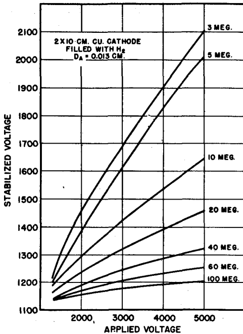
Figure 3. Effect of Series Resistance upon Stabilization
