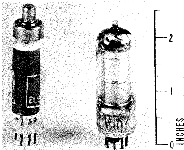
Figure 12. Miniature Type Voltage Regulators BS-101 Corona Tube and OB-2 Glow Tube.
