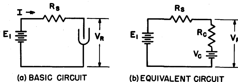
Figure 2. Corona Tube Voltage Regulator Circuit
