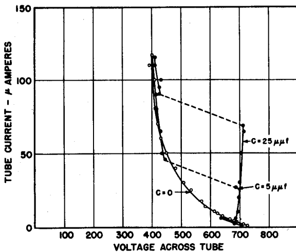
Figure 5. Continuous and Pulsed Operation of Corona Regulator Tube
