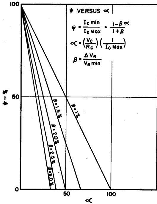
Figure 8. Design Sheet for Corona Regulator Circuit, \psi versus \alpha .
