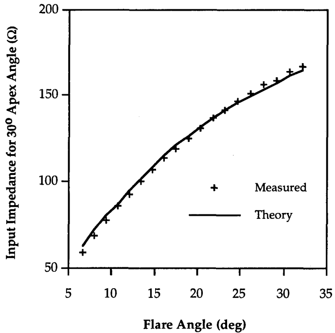
Figure 3.2: Input impedance against flare angle \theta_A for TEM horn with 30^\circ apex angle
