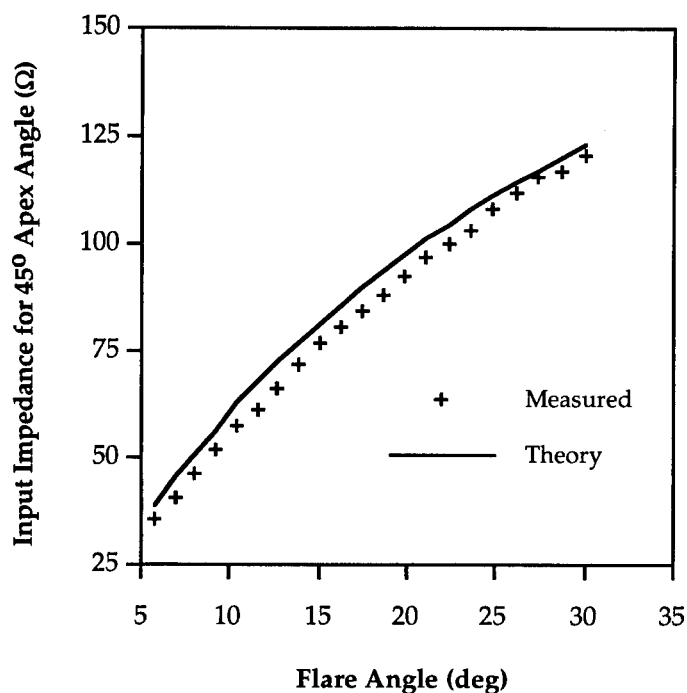
Figure 3.3: Input impedance against flare angle \theta_A for TEM horn with 45° apex angle
