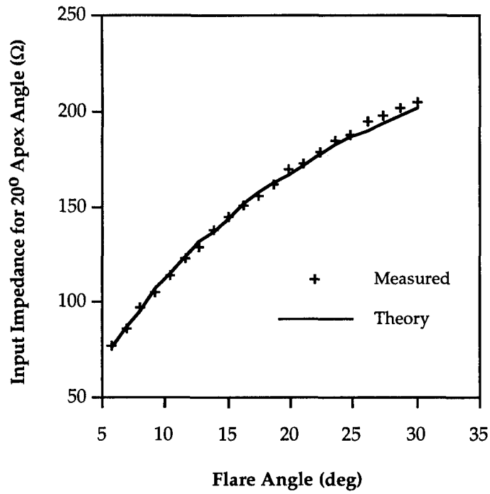
Figure 3.1: Input impedance against flare angle \theta_A for TEM horn with 20^\circ apex angle
