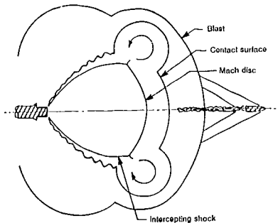
Figure 17: Schematic of muzzle flow
