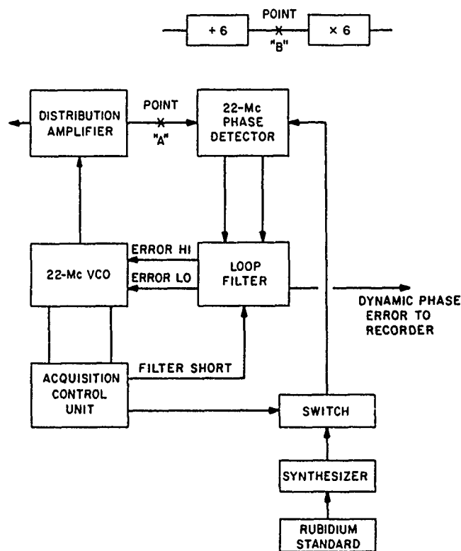
Fig. 37. Microwave link incidental phase modulation test setup
