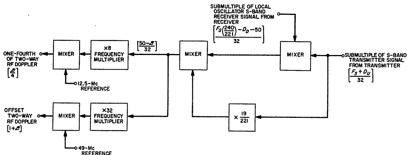
Fig. 32. Doppler extractor
