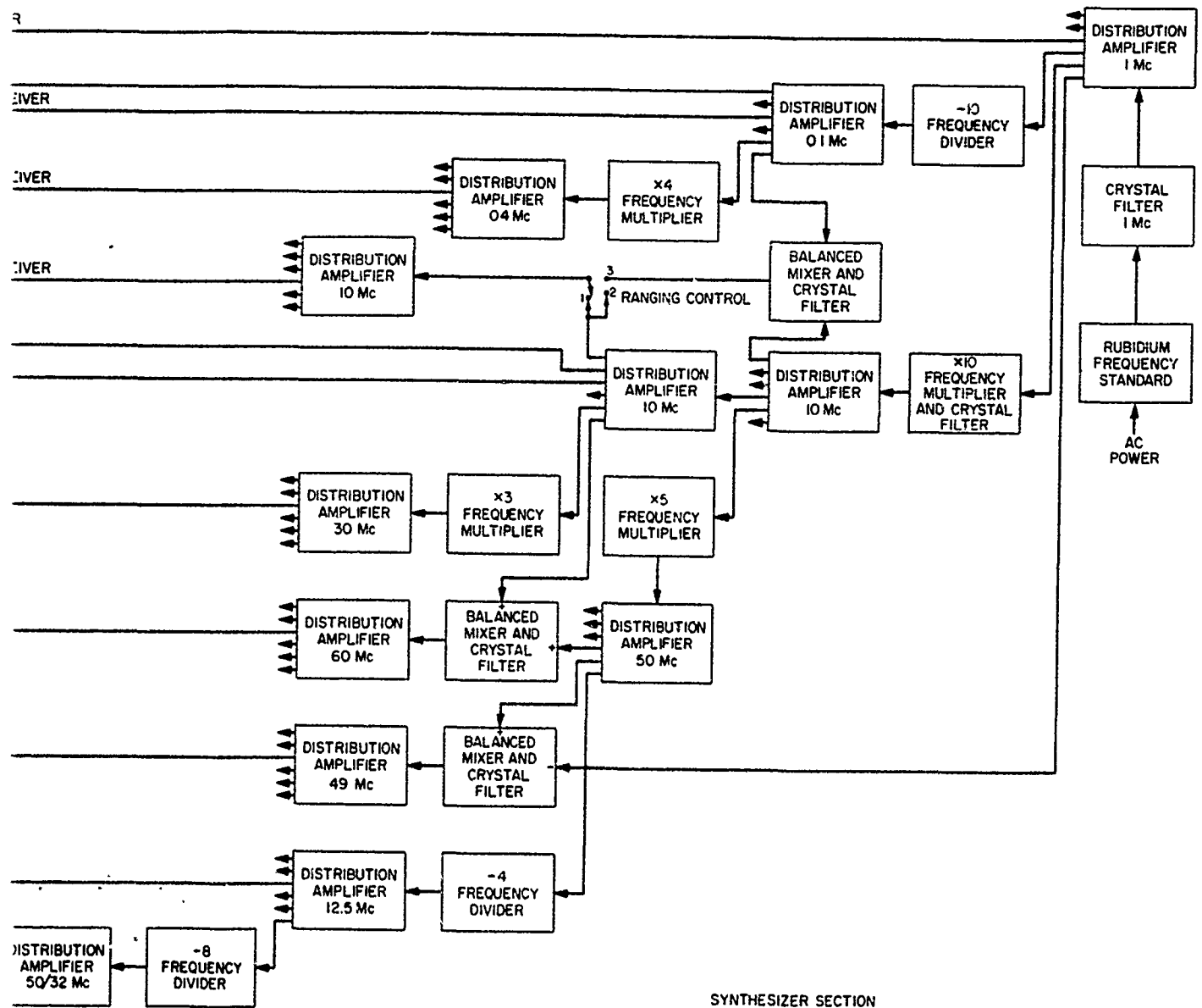
SYNTHESIZER SECTION
