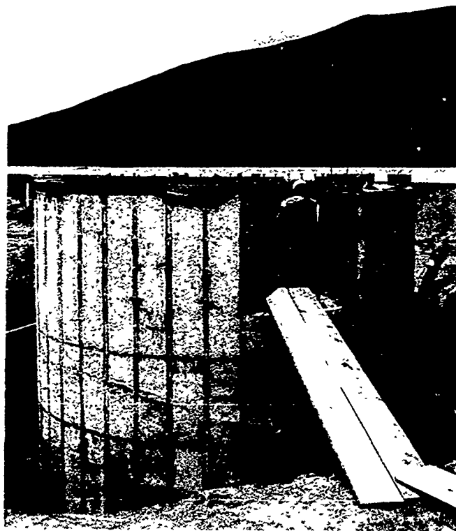
Fig. 6. View of 30-ft antenna base pedestal under construction
