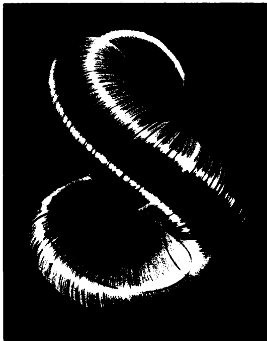
FIGURE 28-Two-Lobed "Baseball Seam" Instability Of Type V Toroidal Iso- tensoid Pressure Vessel
