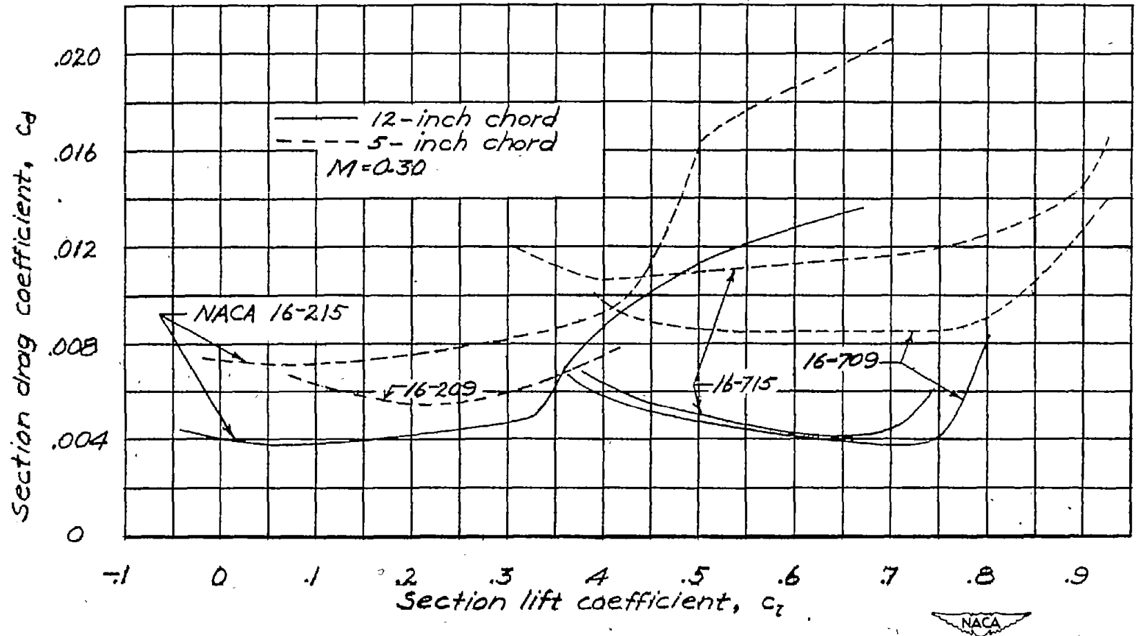
Figure 5.- Variation of drag coefficient with lift coefficient for four NACA 16-series airfoils of two different chord lengths.
