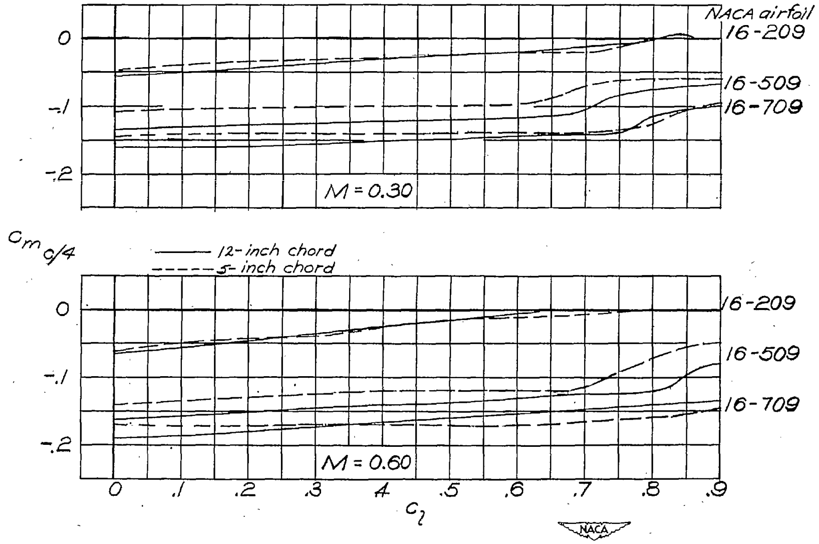
Figure 4.- Variation of moment coefficient with lift coefficient for six NACA 16-series airfoils of two different chord lengths.
