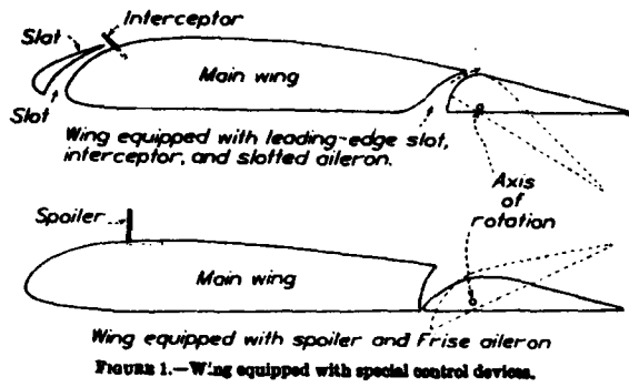
FIGURE 1.—Wing equipped with special control devices.
