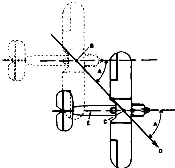
FIGURE 11.—Sideslip.
