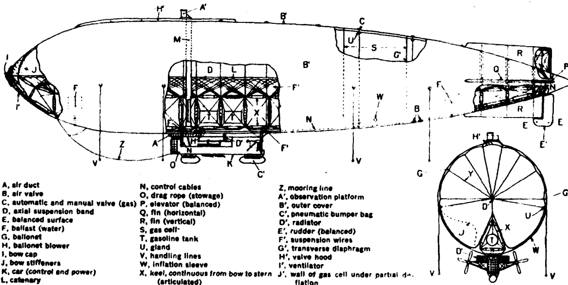
FIGURE 4.—A semirigid airship.
