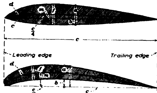
a/c, upper camber b/c, lower camber c/c, mean camber c, chord length d, mean line of the airfoil profile c/4, aerodynamic center (quarter-chord point) f, profile thickness FIGURE 2.—Dimensions of an airfoil profile.
