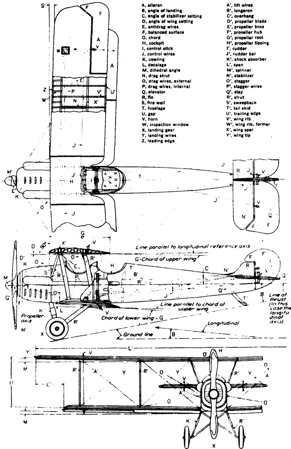
FIGURE 5 - An airplane.
