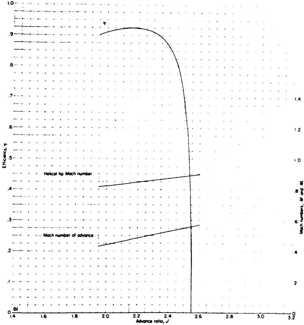
(b) Propeller efficiency.
