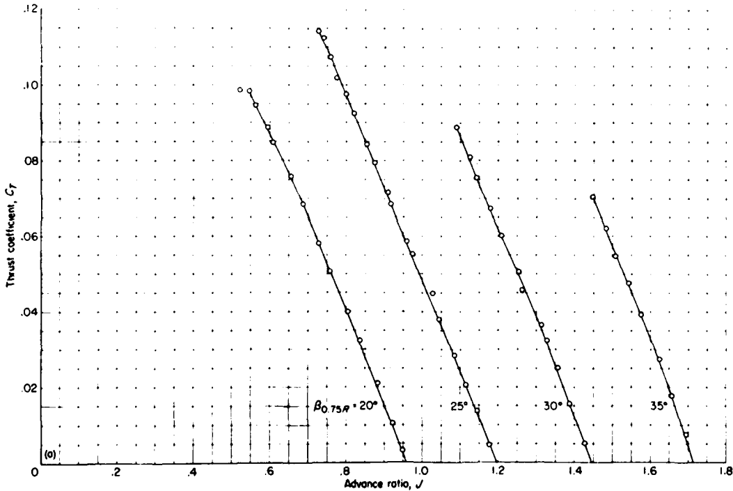
(a) Propeller thrust coefficient.
