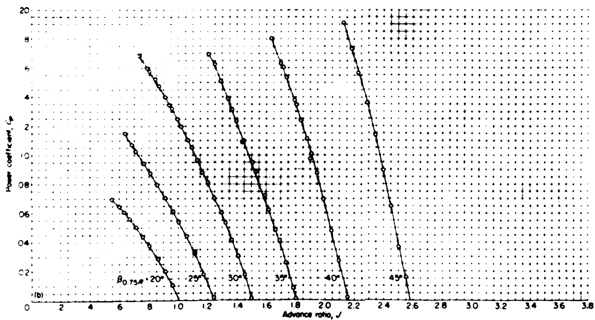
(b) Propeller power coefficient
