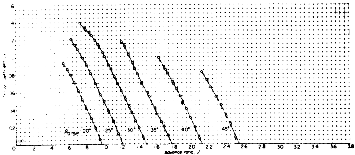
(a) Propeller thrust coefficient
