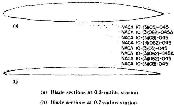
FIGURE 7.—Comparison of blade sections at two radial stations for NACA propellers having a solidity of 0.045 per blade at the 0.7-radius station.
