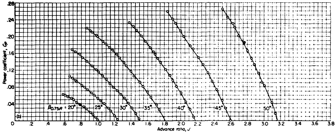
(b) Power coefficient.
