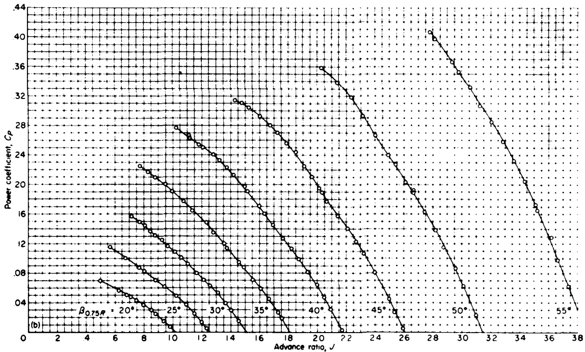
(b) Propeller power coefficient.
