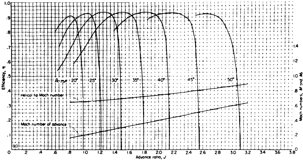
(c) Propeller efficiency.
