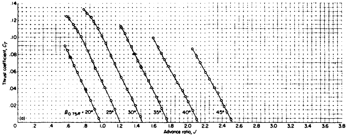
(a) Propeller thrust coefficient.
