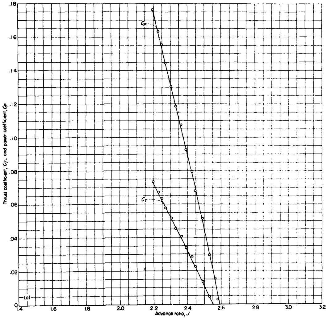
(a) Propeller thrust and power coefficients.
