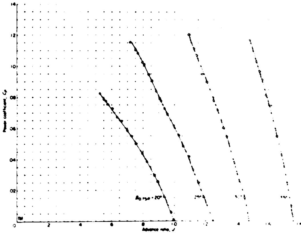
h. Propeller power coefficient
