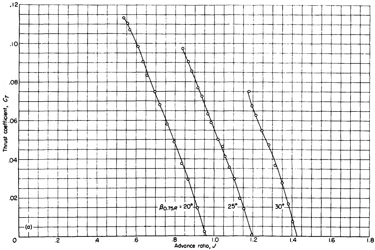
(a) Propeller thrust coefficient.
