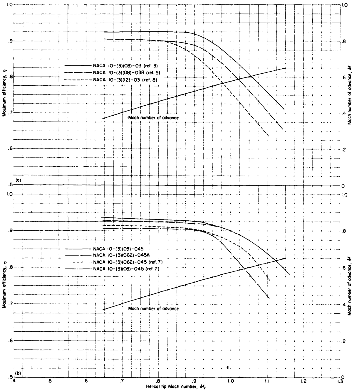
FIGURE 31.—The effect of compressibility on the maximum efficiency of NACA propellers having different blade-section thicknesses. \rho_{0.75R} = 45^\circ
