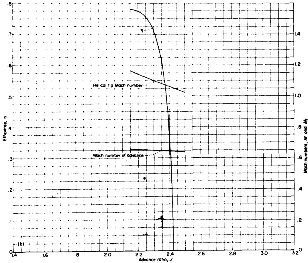
(b) Propeller efficiency.
