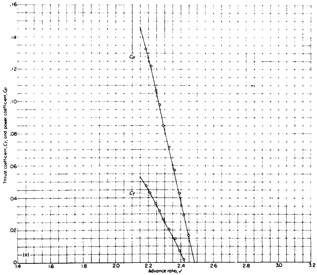
(a) Propeller thrust and power coefficients.
