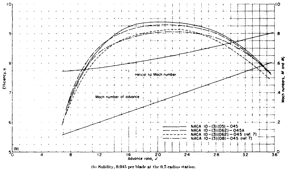
FIGURE 28.—The efficiency of NACA propellers having different blade-section thicknesses when operating at a constant power coefficient of 0.15 and a rotational speed of 1,140 rpm.
