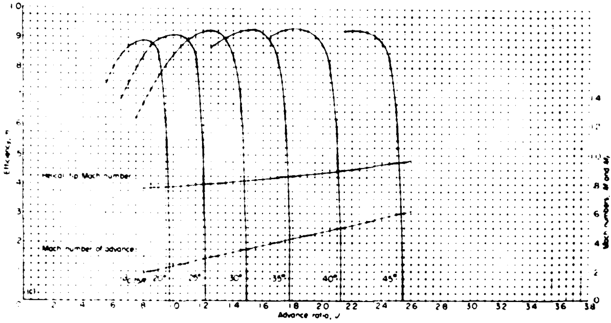
FIGURE 20. Concluded. Rotational speed, 1,000 rpm.
