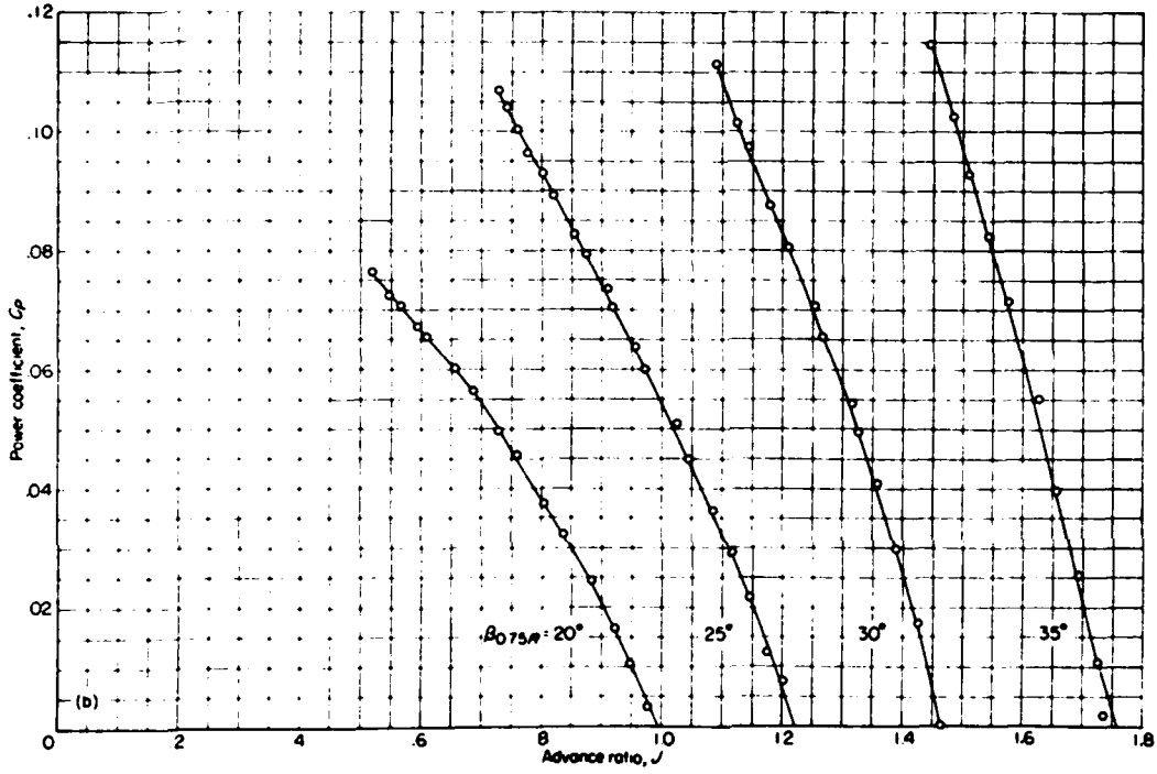
(b) Propeller power coefficient.
