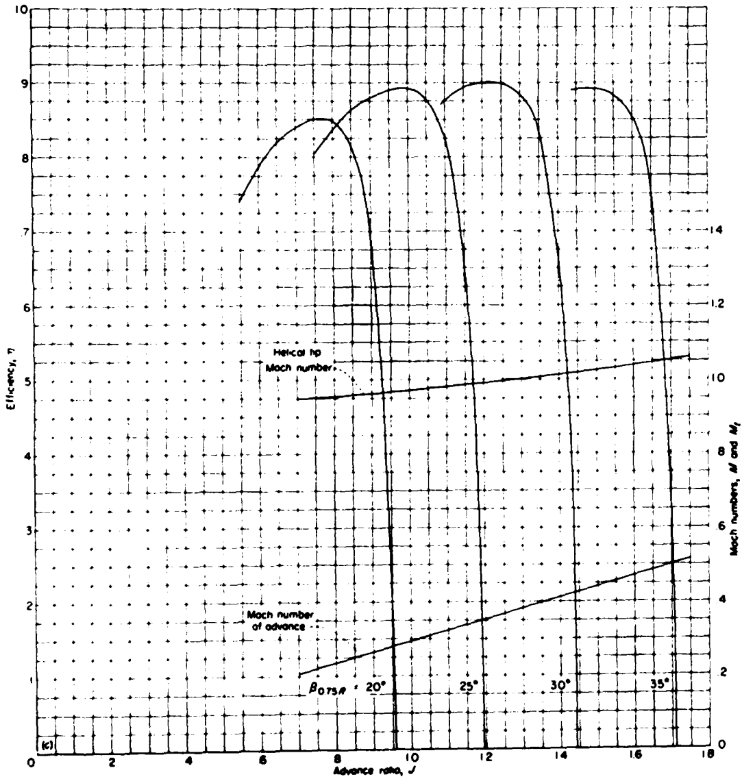
(c) Propeller efficiency.
