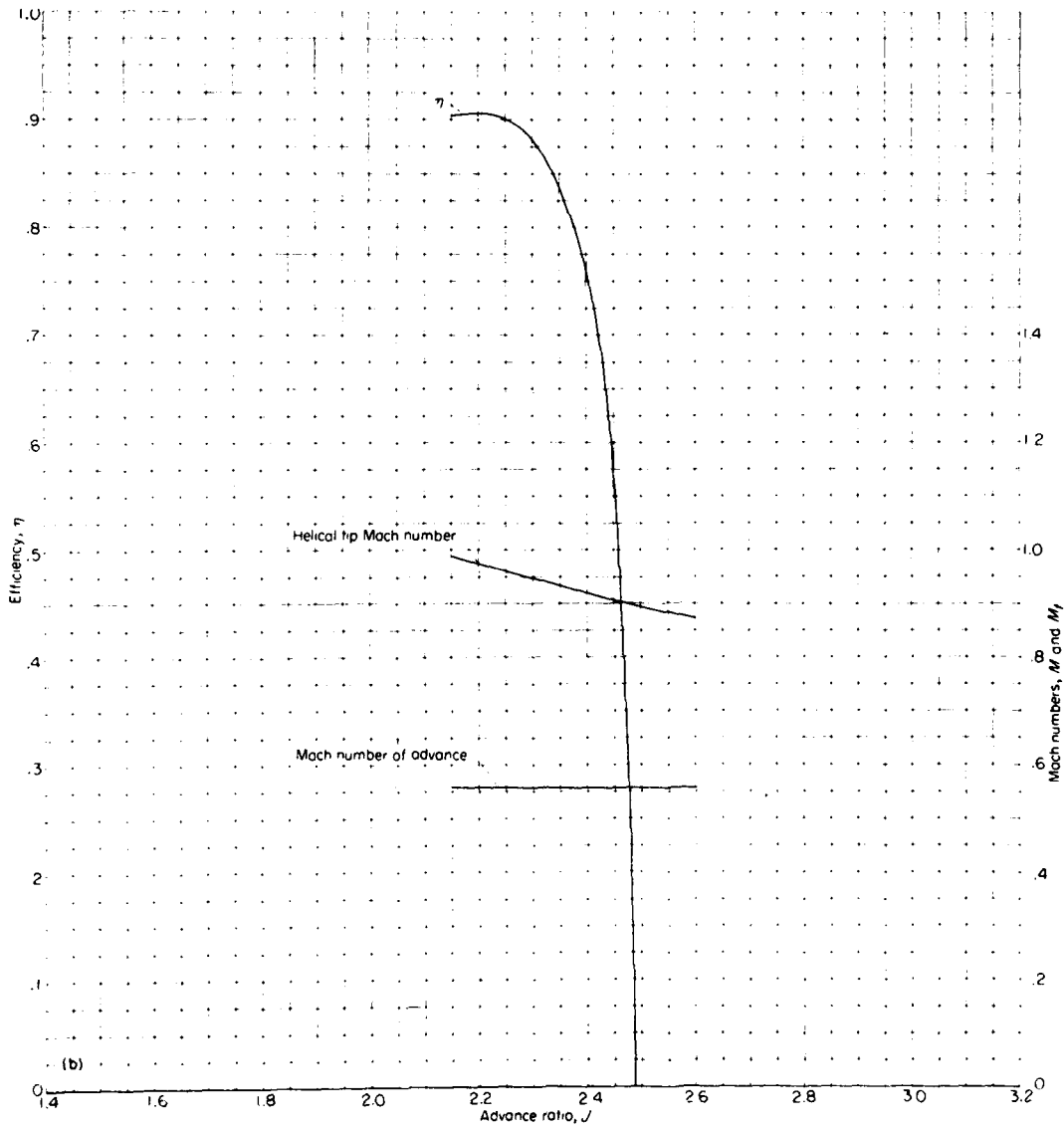
(b) Propeller efficiency.
