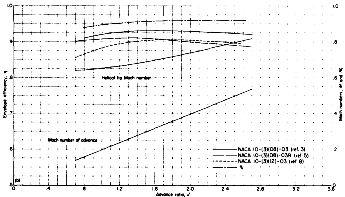
(b) 1,350 rpm.
