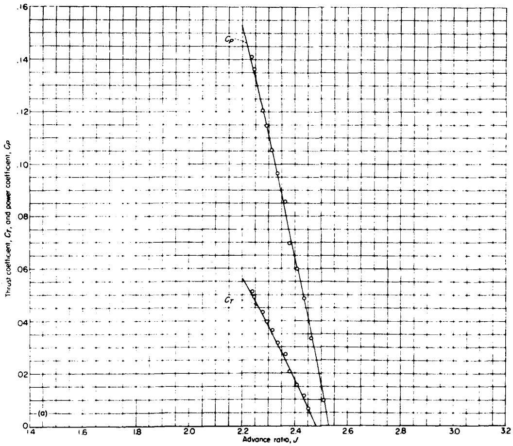
(a) Propeller thrust and power coefficients.
