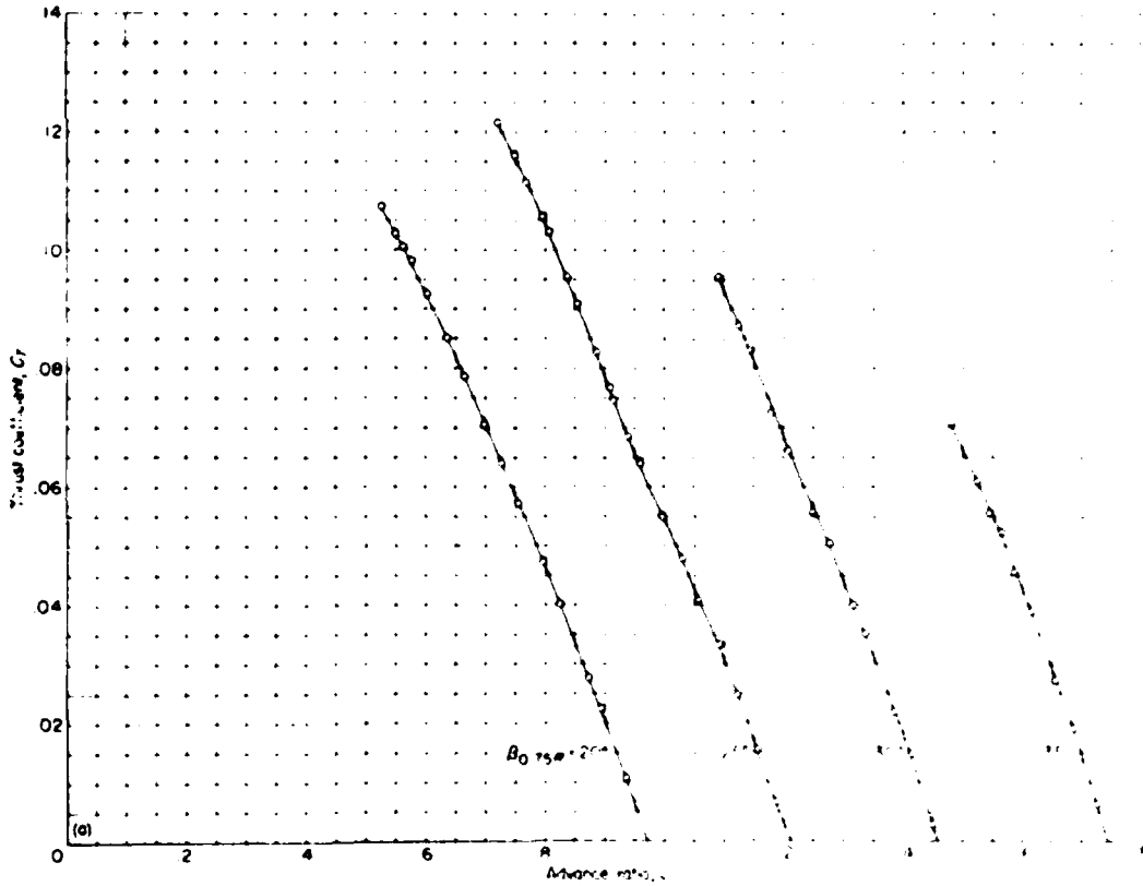
FIGURE 21. Characteristics of NACA 10 (3-05-015) propeller. Rotational speed, 2,000 rpm.
