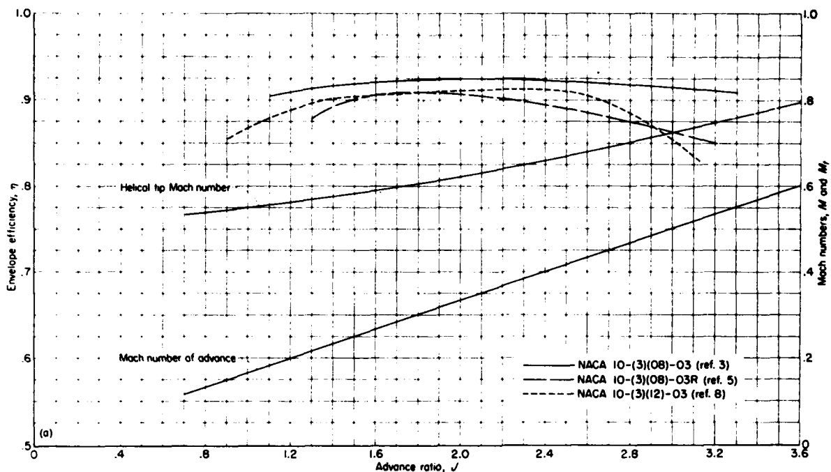
(a) 1,140 rpm.
