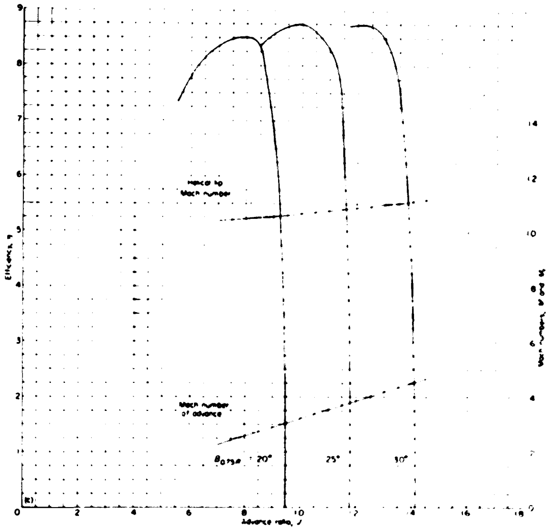
(e) Propeller efficiency.
