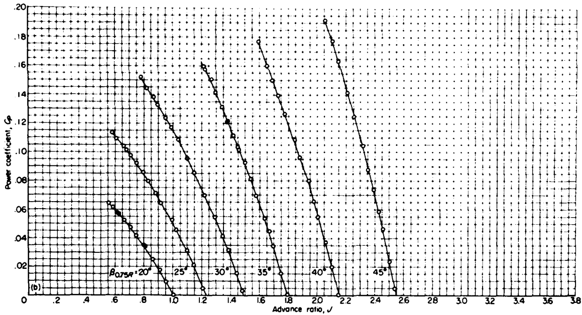
(b) Propeller power coefficient.
