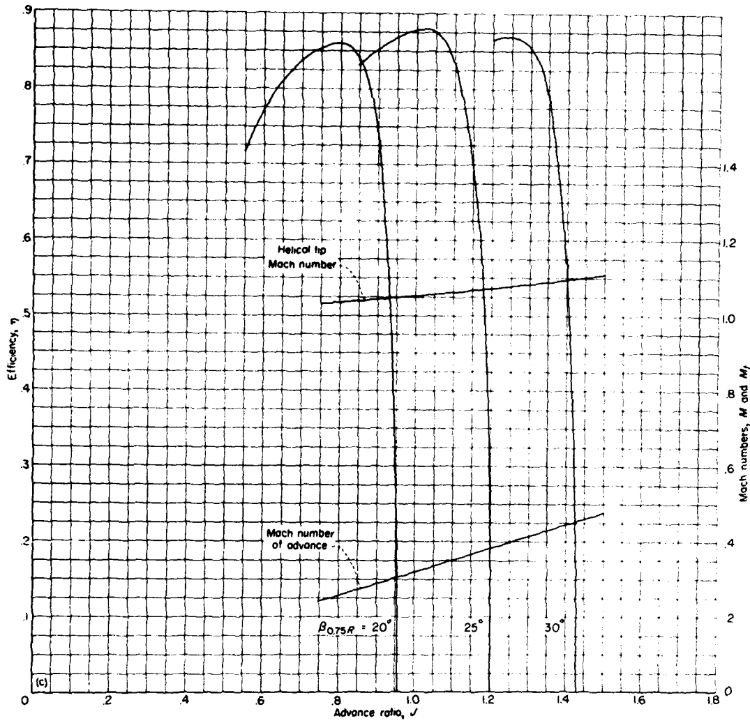
(c) Propeller efficiency.
