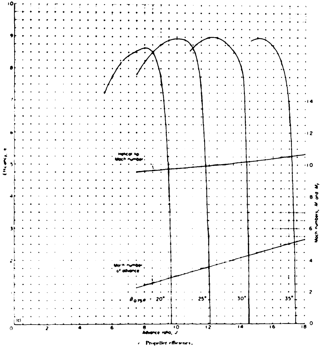
FIGURE 21 (continued) Rotational speed, 2,000 rpm.
