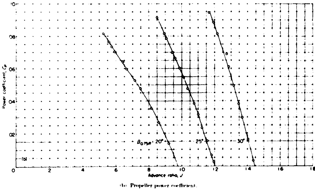
FIGURE 13. Characteristics of NACA 10 (3-062) 015A propeller. Rotational speed, 2,160 rpm
