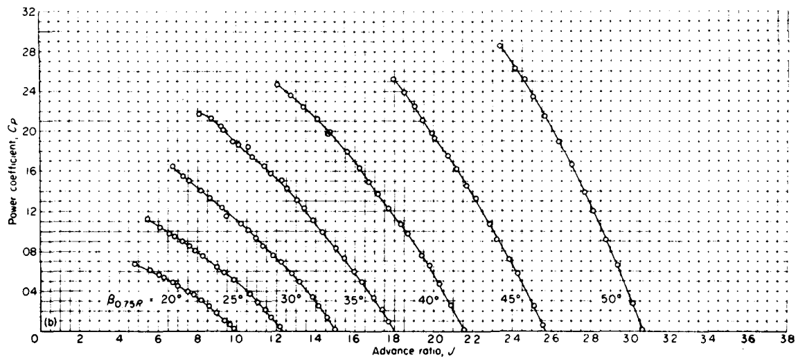
(b) Propeller power coefficient.
