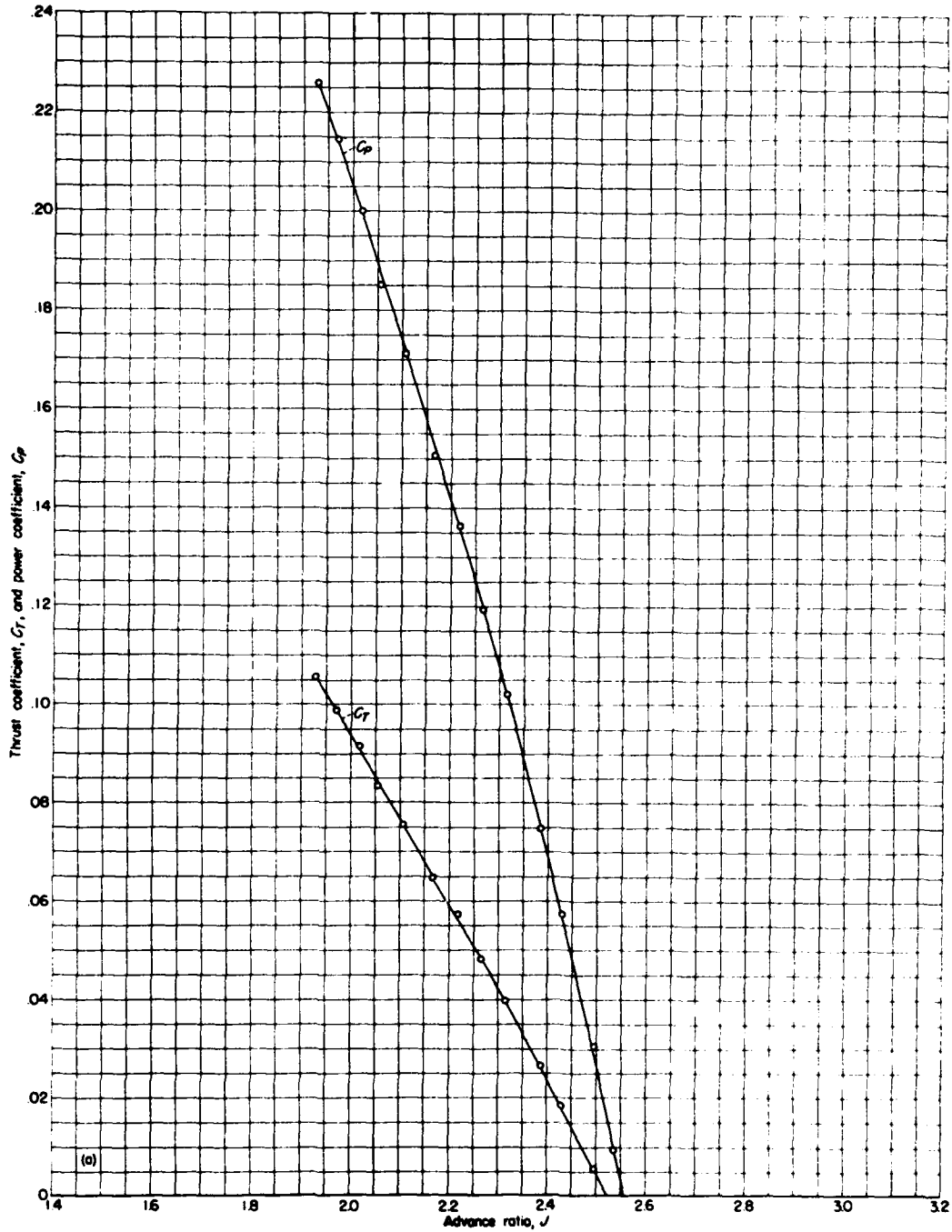
(a) Propeller thrust and power coefficients.
