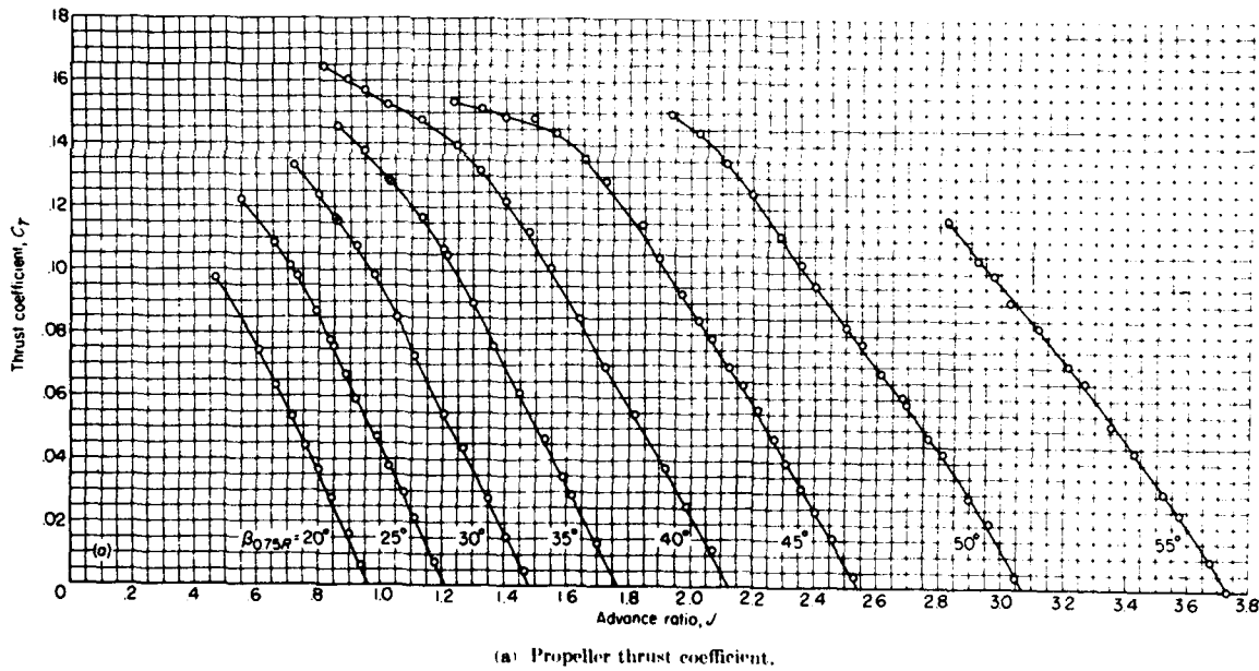
FIGURE 8.—Characteristics of NACA 10 (3)(0.32) 045A propeller. Rotational speed, 1,140 rpm.
