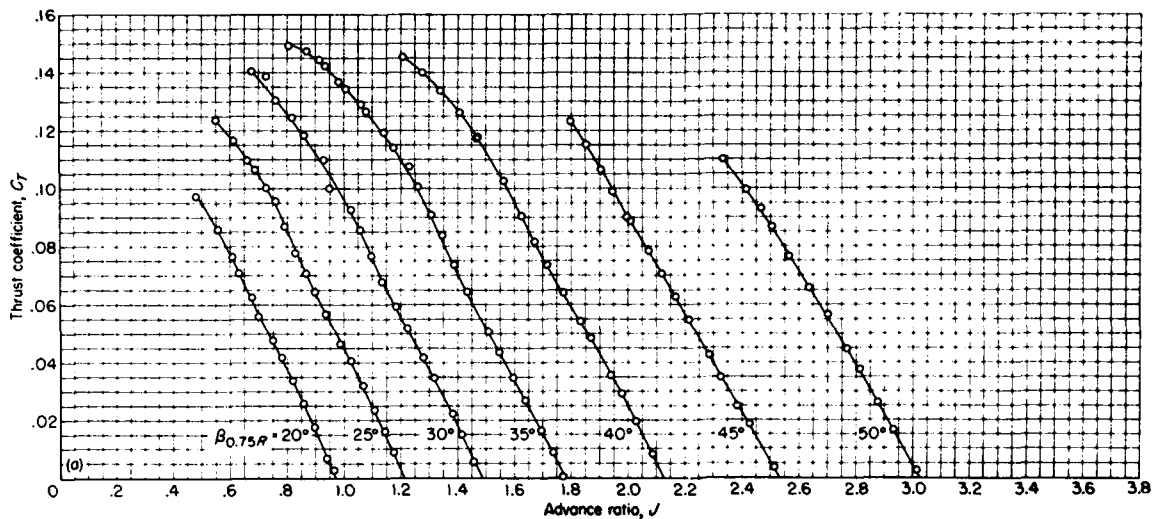
(a) Propeller thrust coefficient.
