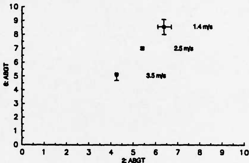
Figure 4-8. T_{\infty} - t_{\infty} ( ^{\circ}\text{C} ) Temperature Difference of 6-inch (15-cm) ABGT and 2.25-inch (5.7-cm) ABGT at Indicated Wind Speeds (Bars Indicate Range of Data)
