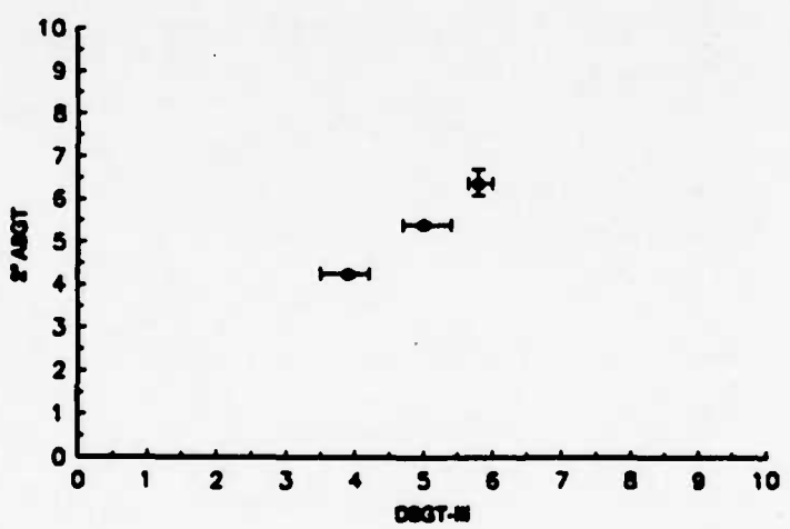
Figure 4-9. T_{avg}-t_s (°C) Temperature Difference of 6-inch (15-cm) and 2.25-inch (5.7-cm) ABGT to DBGT (Bars Represent Range of Data)
