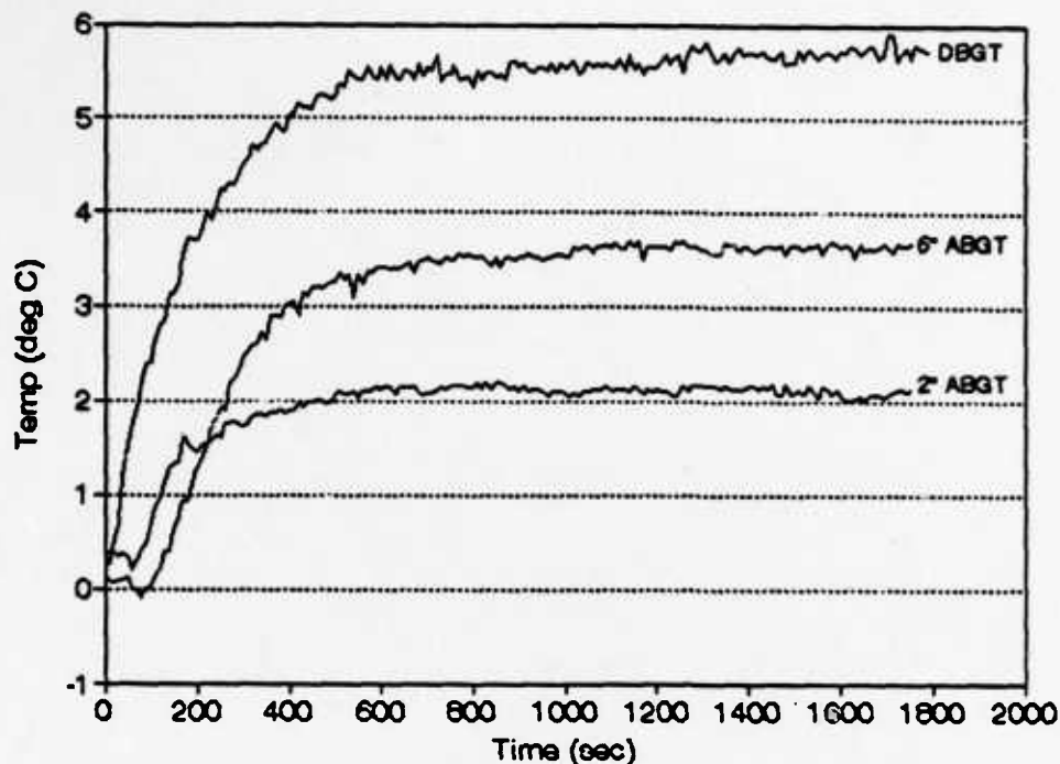
Figure 4-5. Time Response of Temperature Difference Between Selected Globe Thermometers and a Reference Dry Bulb (Thermistor) Sensor (Wind= 3.4 m/s)
