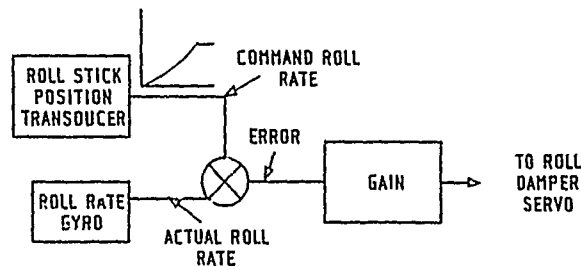
Figure 2.1 - F111C Roll Control System Schematic
