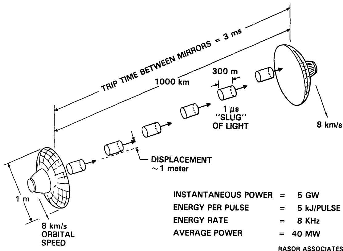
Figure 4-3 Extracting stored ionospheric energy with two orbiting mirrors
