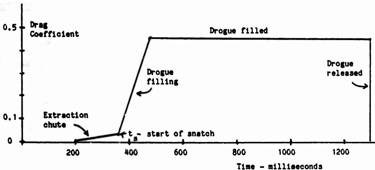
Figure 3-4 DROGUE CHUTE
