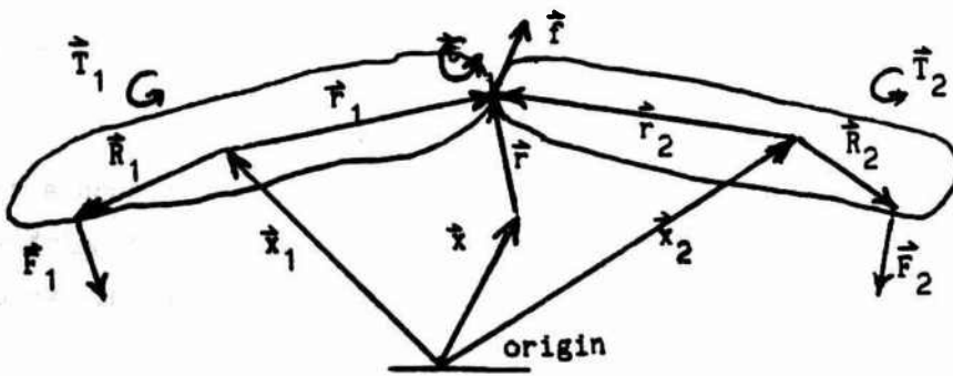
Figure 5-2 SLENDER BODY
