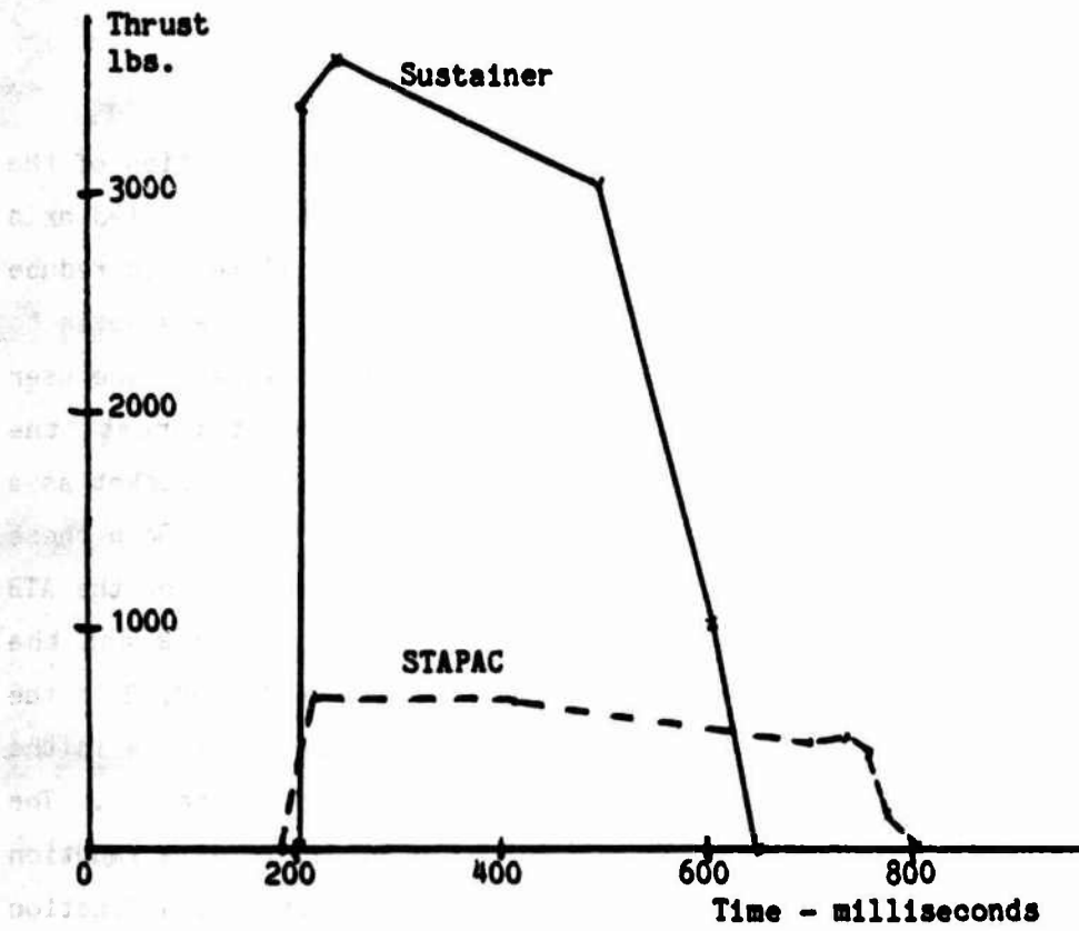
Figure 3-2 ROCKET THRUST
