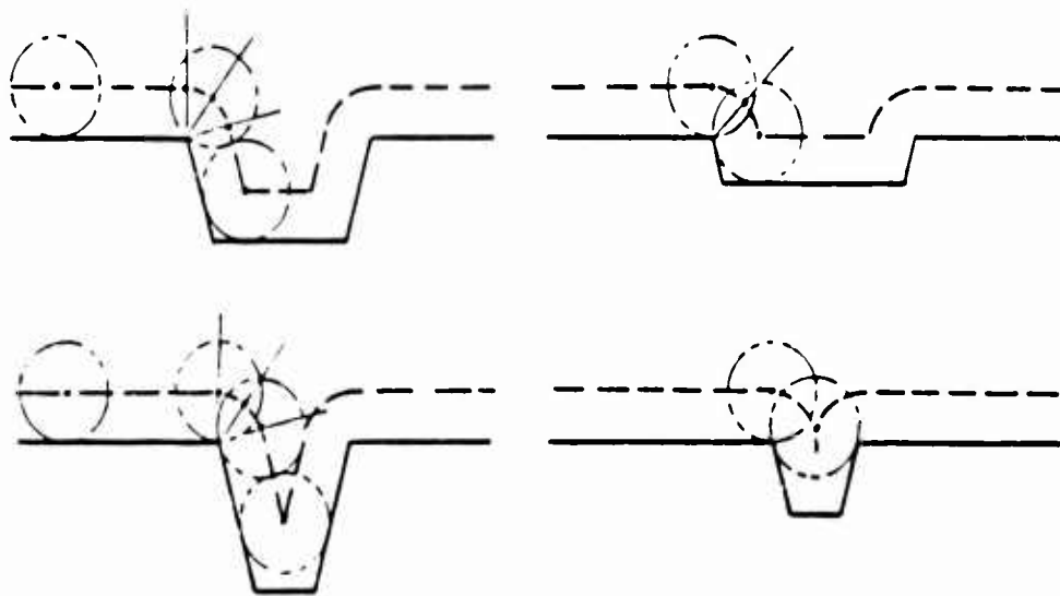
FIGURE 11.A.4 - Hub Profiles Across Ditches
