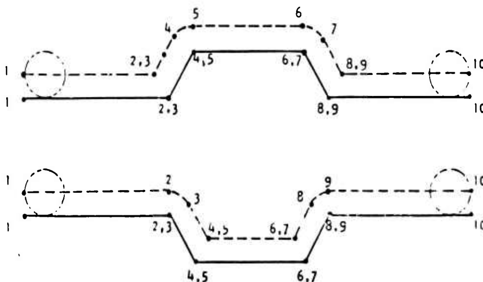
FIGURE II.D.1 -- Obstacle and Hub Profile Breakpoint Indices
