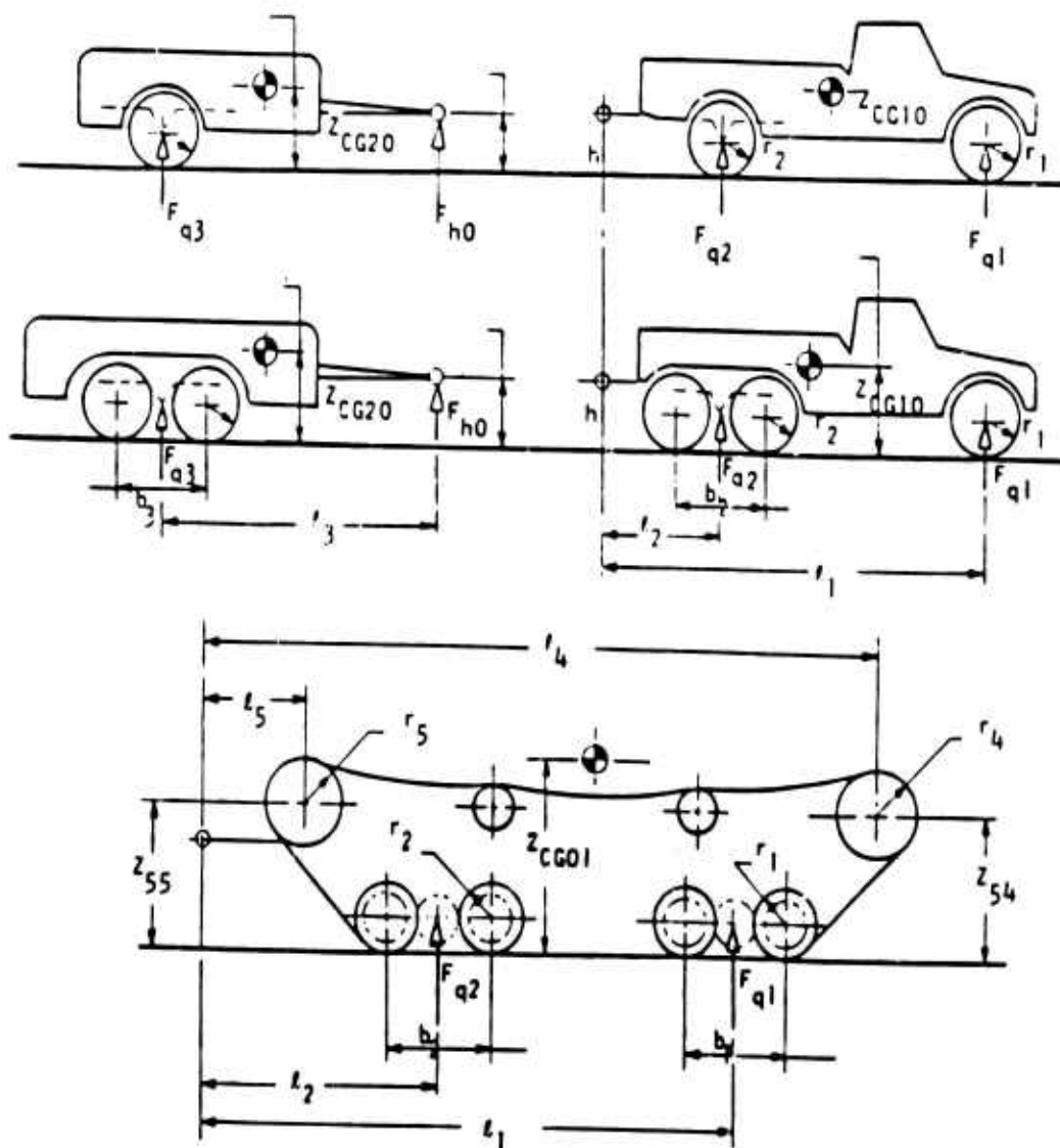
FIGURE 11.A.5 -- Vehicle Parameters
