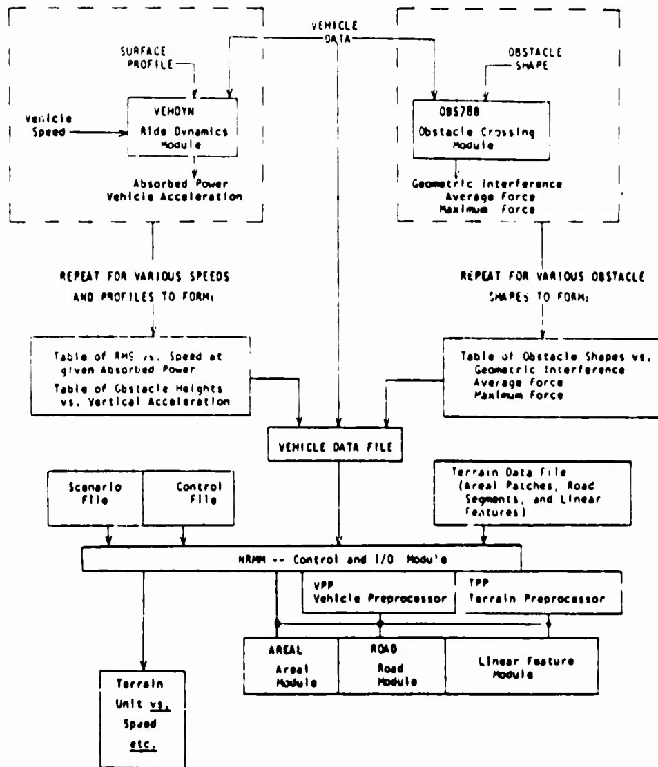
FIGURE 1.0.1 - GENERAL ORGANIZATION OF THE INITIAL NATO REFERENCE MOBILITY MODEL
