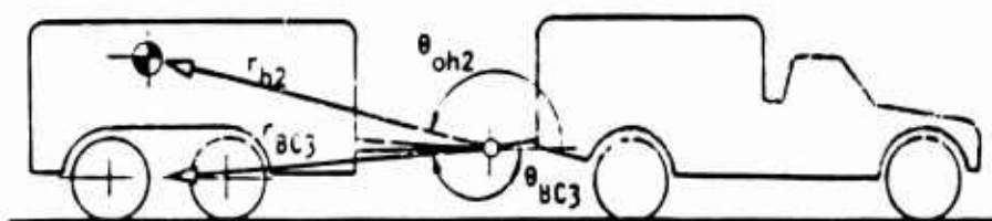
FIGURE 11.C.4 -- Trailer CG and Suspension Support Location
