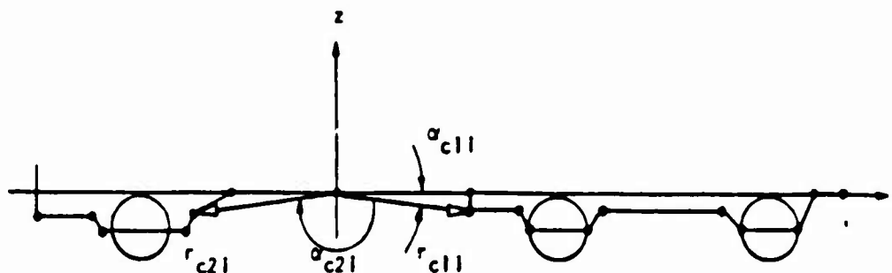
FIGURE 11.C.6 -- Specification of Vehicle Bottom Profile Breakpoints
