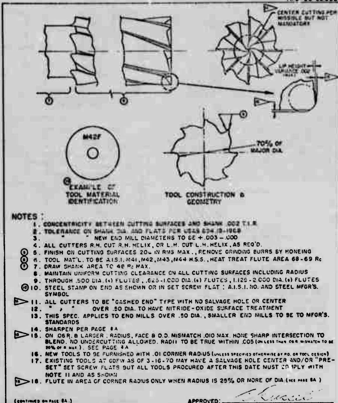
FIGURE C-8 CUTTING TOOL SPECIFICATION - 4, 6 & 8 FLUTE END MILLS
