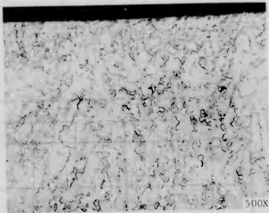
FIGURE J-12 SPECIMEN 16A, Ti-6Al-4V BETA ANNEALED, 0.05" RADIAL DEPTH OF CUT, 3 1/4" PER MINUTE FEED RATE
