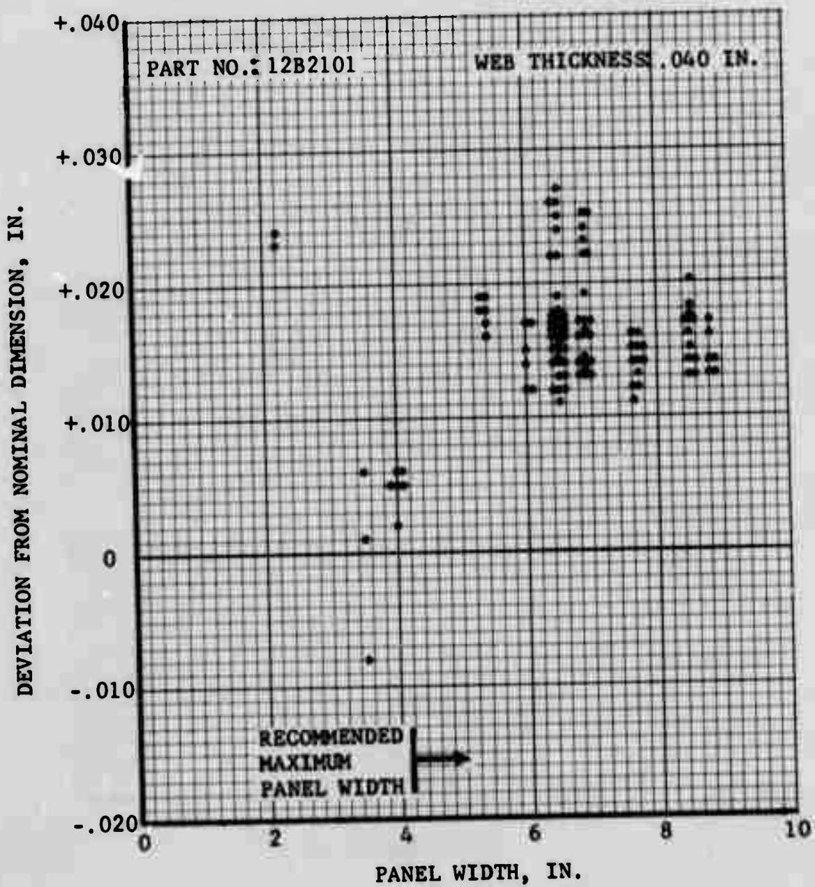
FIGURE B-3 WEB DIMENSIONAL DEVIATION OCCURRENCES VS. STIFFENER SPACING FOR NOMINAL WEB THICKNESS = 0.040
