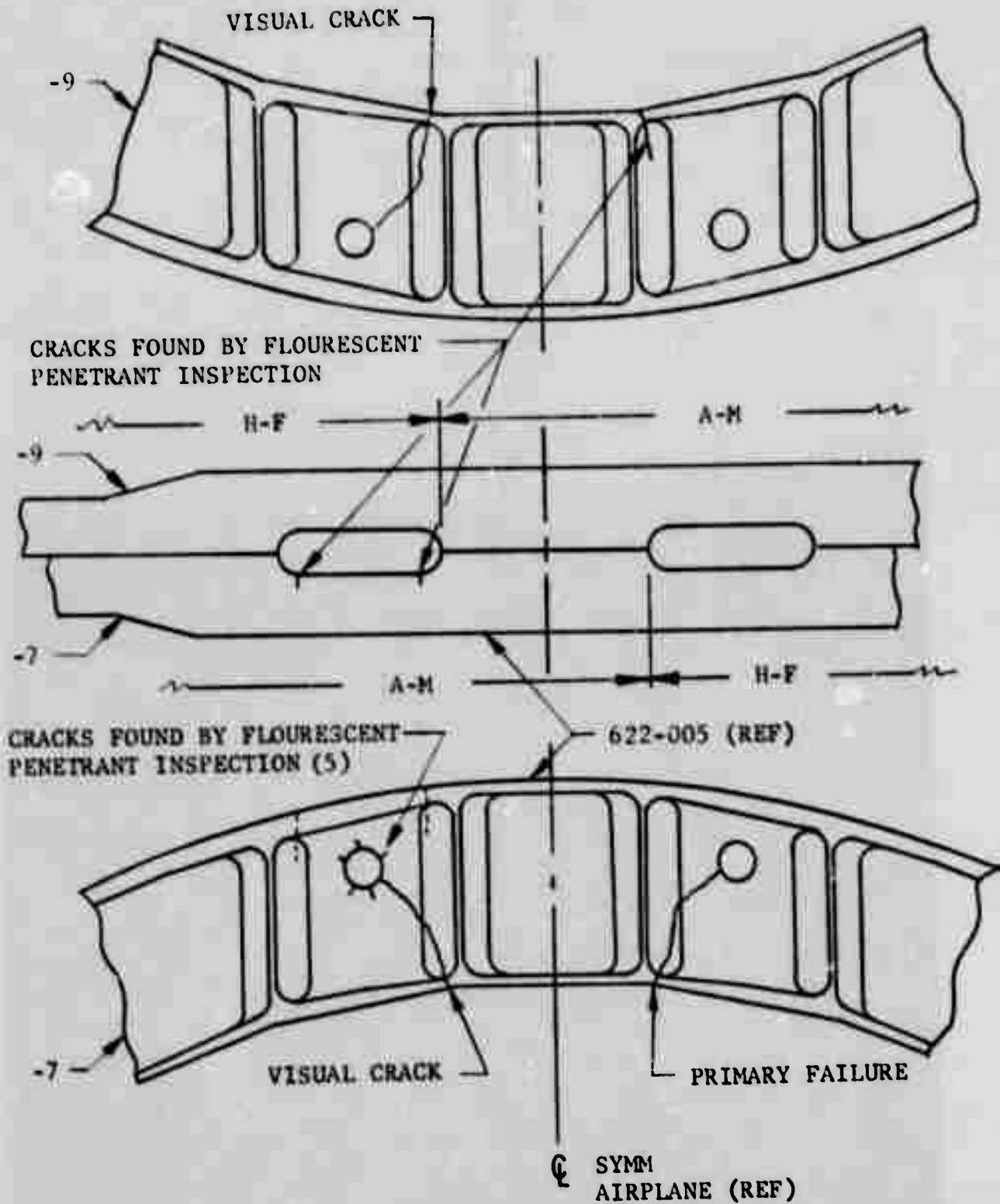
YF-16 FRAME PENETRANT INSPECTION CRACK DISCLOSURE
