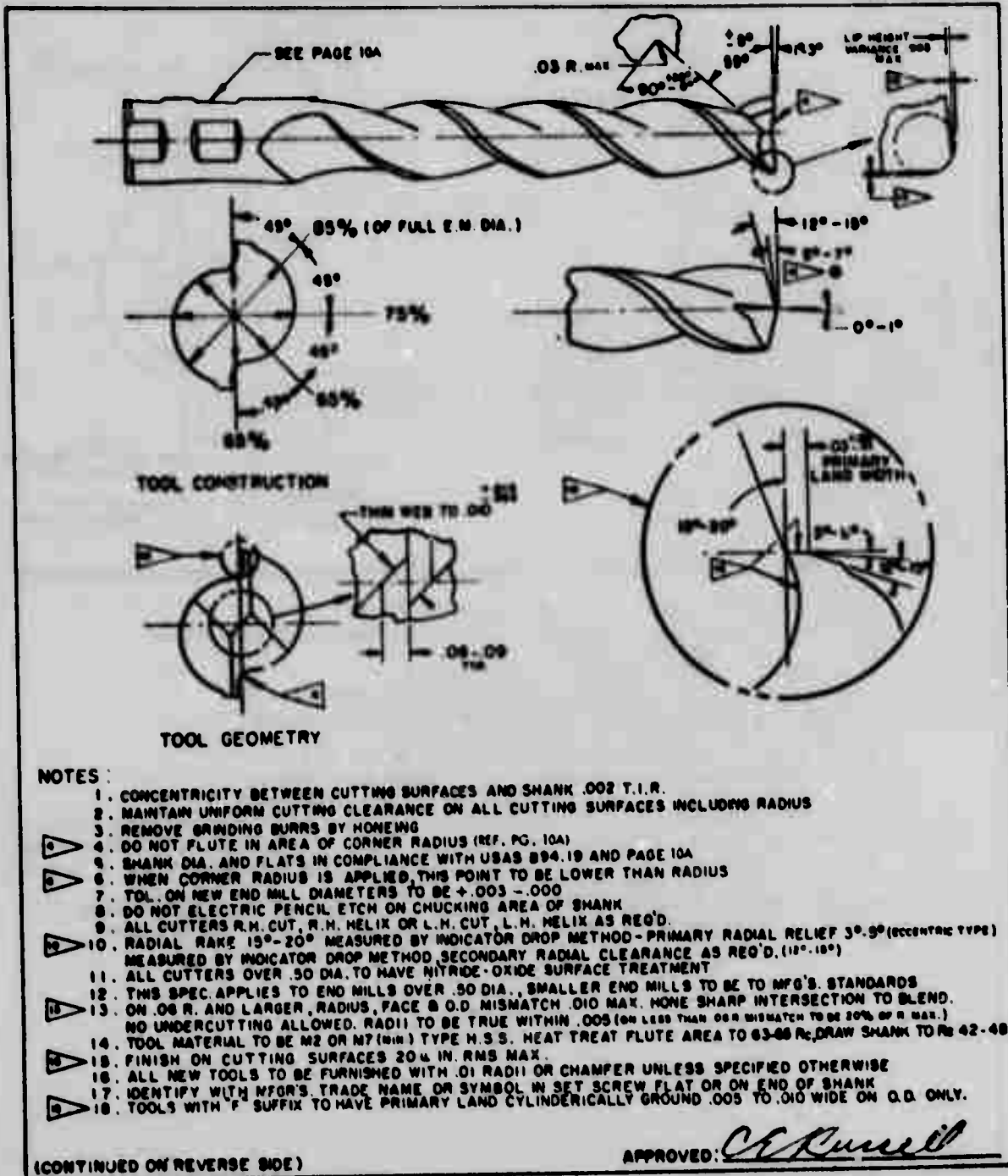
FIGURE C-7 CUTTING TOOL SPECIFICATION - HIGH HELIX ALUMINUM CUTTING END MILLS
